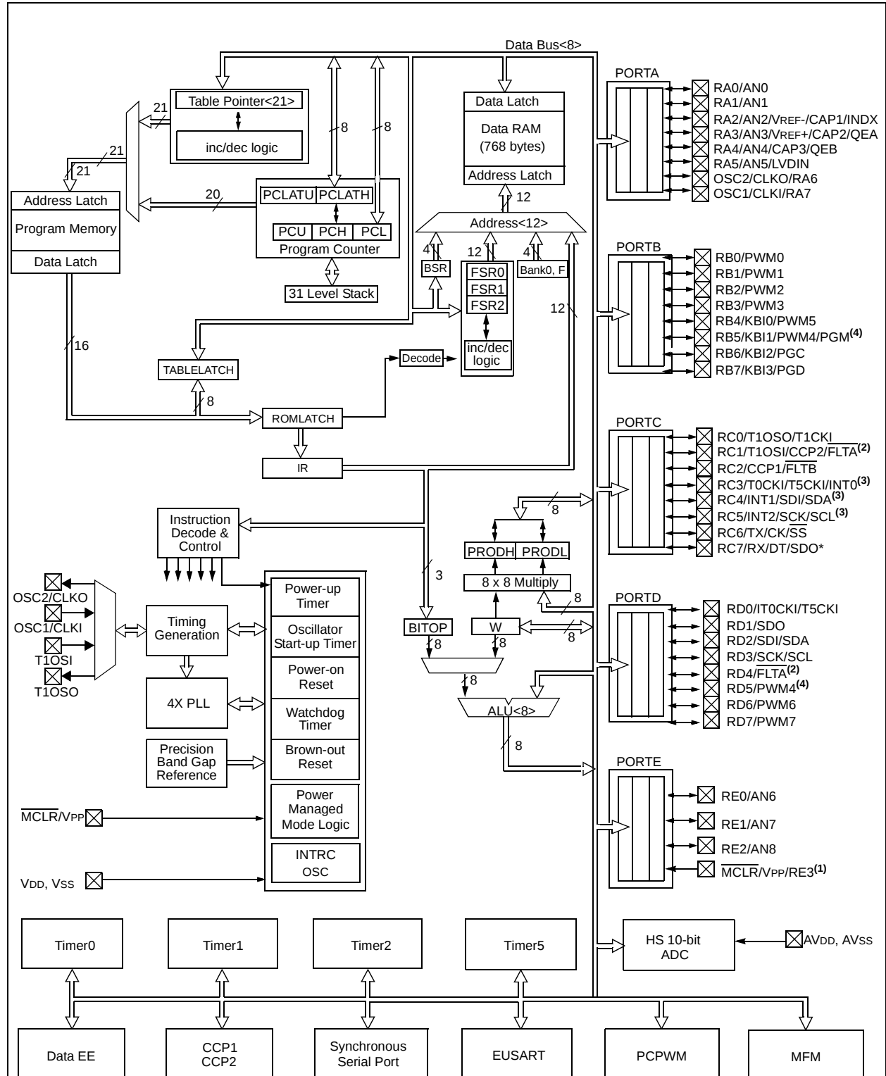
FIGURE 1-2: PIC18F4331/4431 BLOCK DIAGRAM
