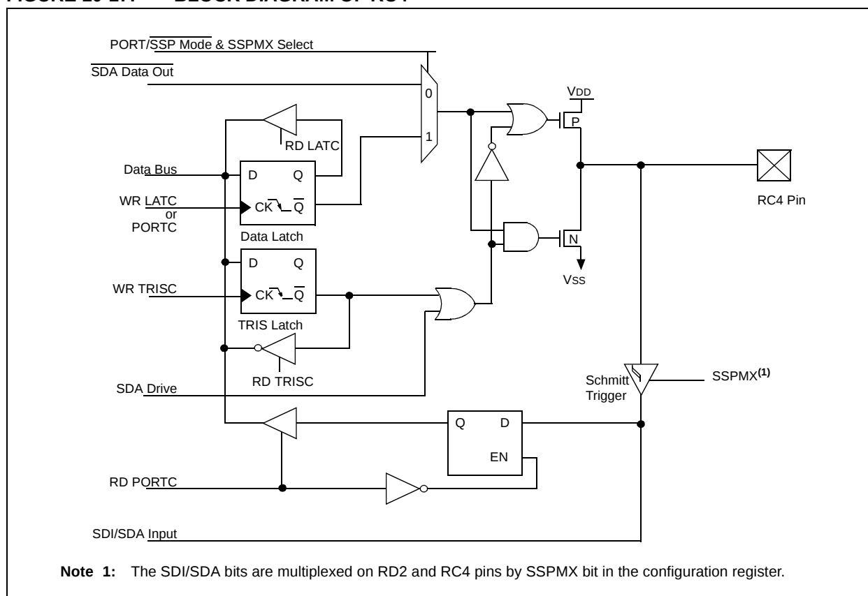
FIGURE 10-17: BLOCK DIAGRAM OF RC4
