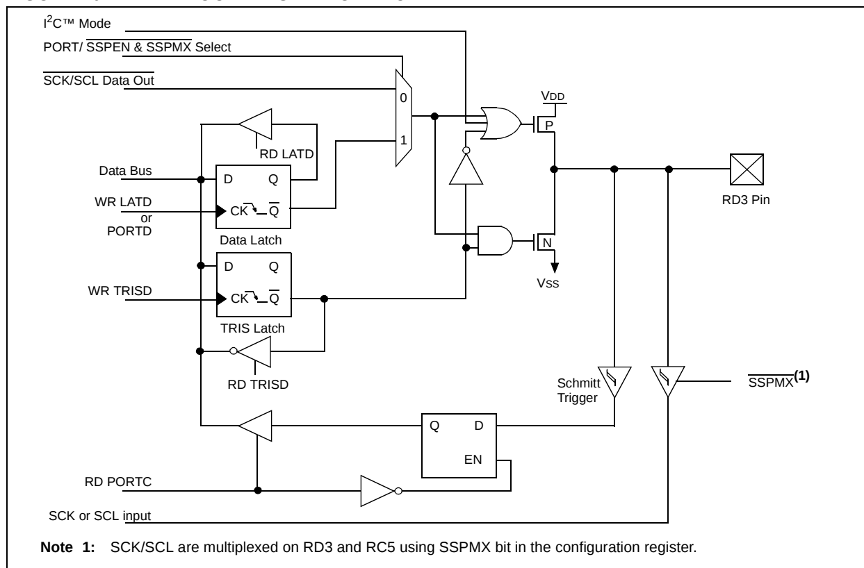
FIGURE 10-24: BLOCK DIAGRAM OF RD3
