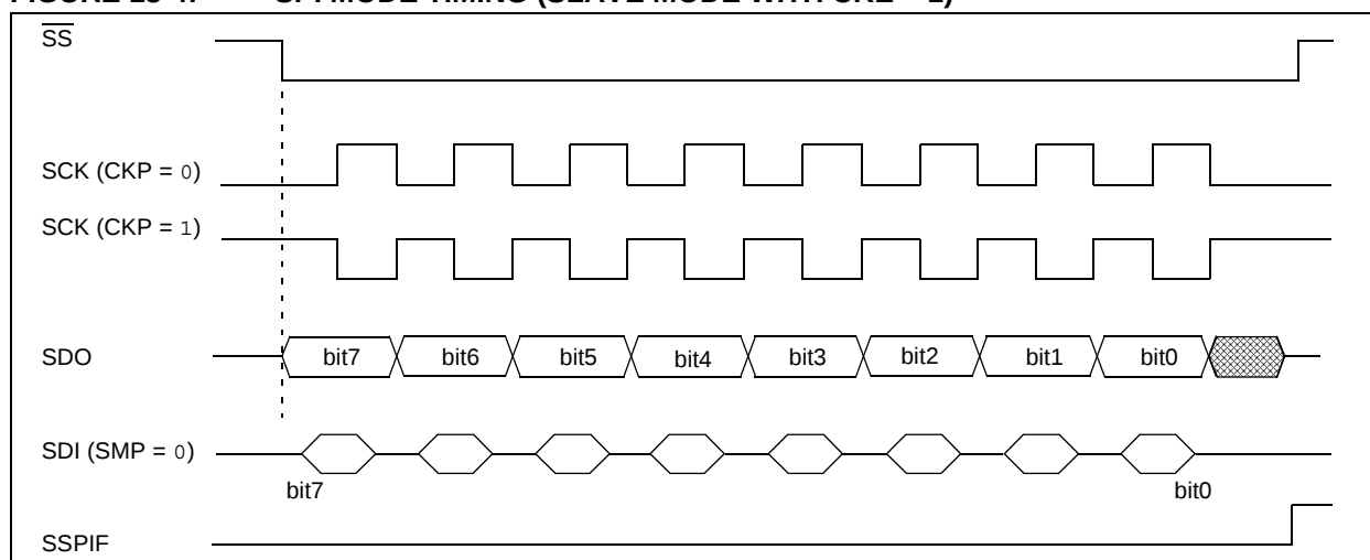
FIGURE 18-4: SPI MODE TIMING (SLAVE MODE WITH CKE = 1)
