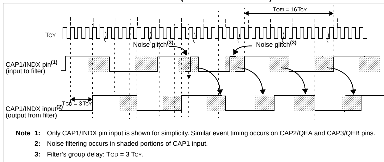
FIGURE 16-14: FILTER TIMING DIAGRAM (CLOCK DIVIDER = 1:1)
