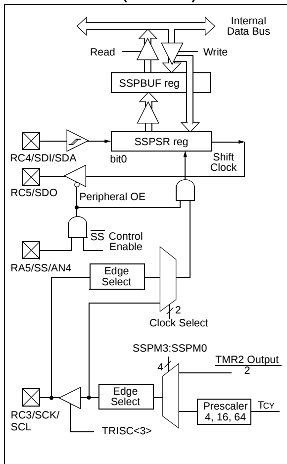
FIGURE 18-1: SSP BLOCK DIAGRAM (SPI MODE)
