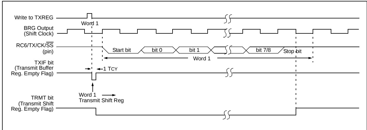
FIGURE 19-3: ASYNCHRONOUS TRANSMISSION
