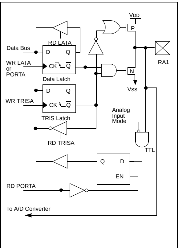
FIGURE 10-3: BLOCK DIAGRAM OF RA1
