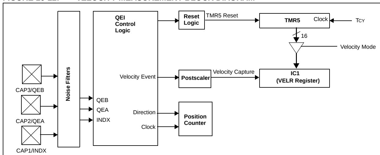
FIGURE 16-12: VELOCITY MEASUREMENT BLOCK DIAGRAM
