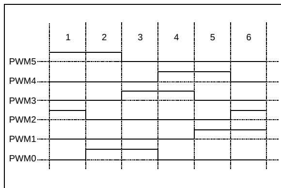
FIGURE 17-21: PWM OUTPUT OVERRIDE EXAMPLE #1
