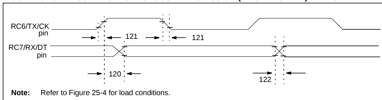
FIGURE 25-19: USART SYNCHRONOUS TRANSMISSION (MASTER/SLAVE) TIMING
