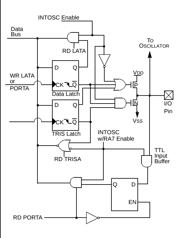
FIGURE 10-8: BLOCK DIAGRAM OF RA7
