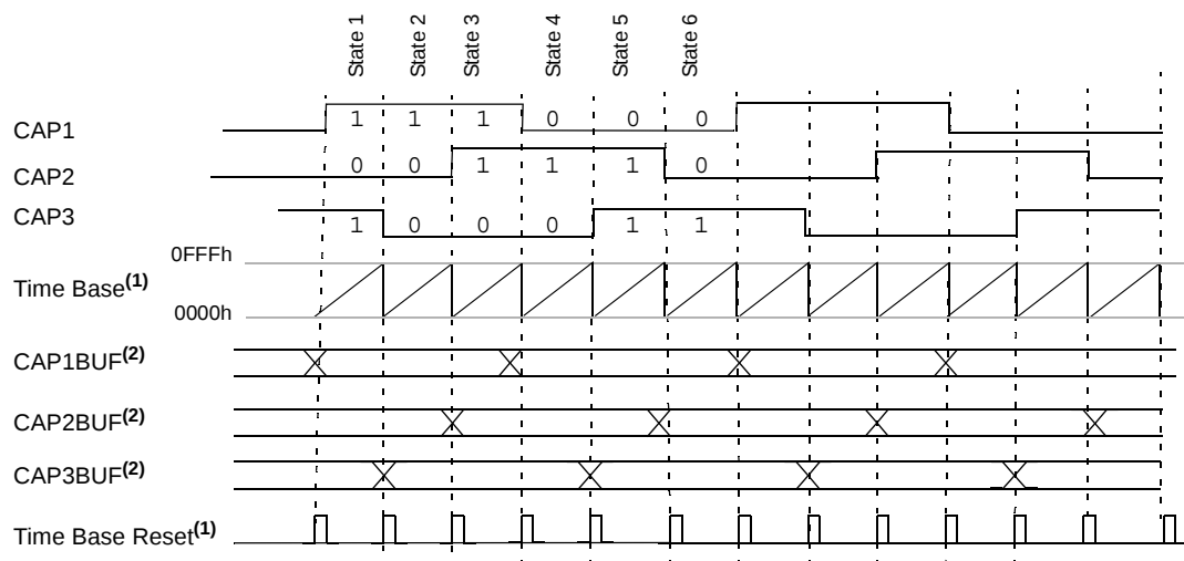
FIGURE 16-6: INPUT CAPTURE ON STATE CHANGE (HALL-EFFECT SENSOR MODE)
