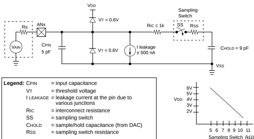
FIGURE 20-2: ANALOG INPUT MODEL
