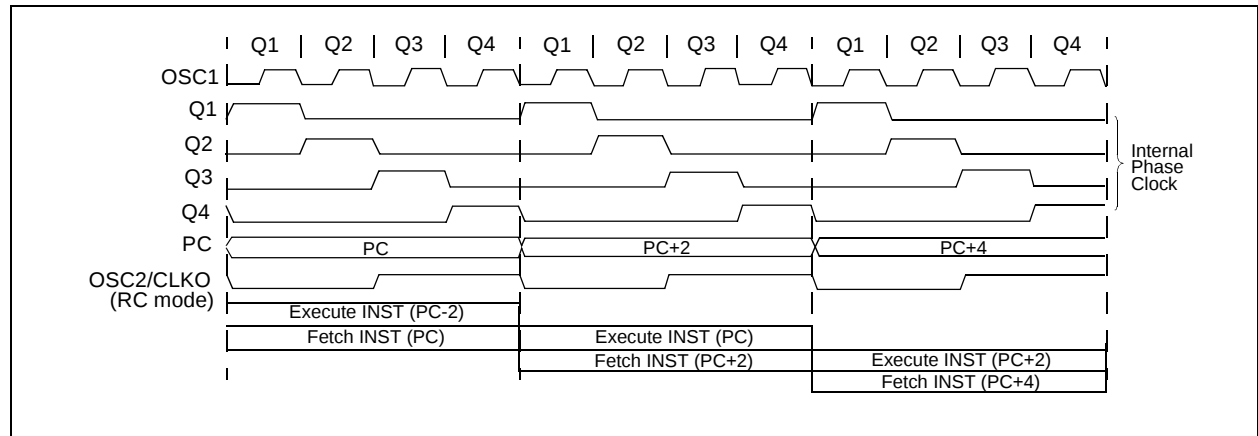
FIGURE 5-4: CLOCK/INSTRUCTION CYCLE
