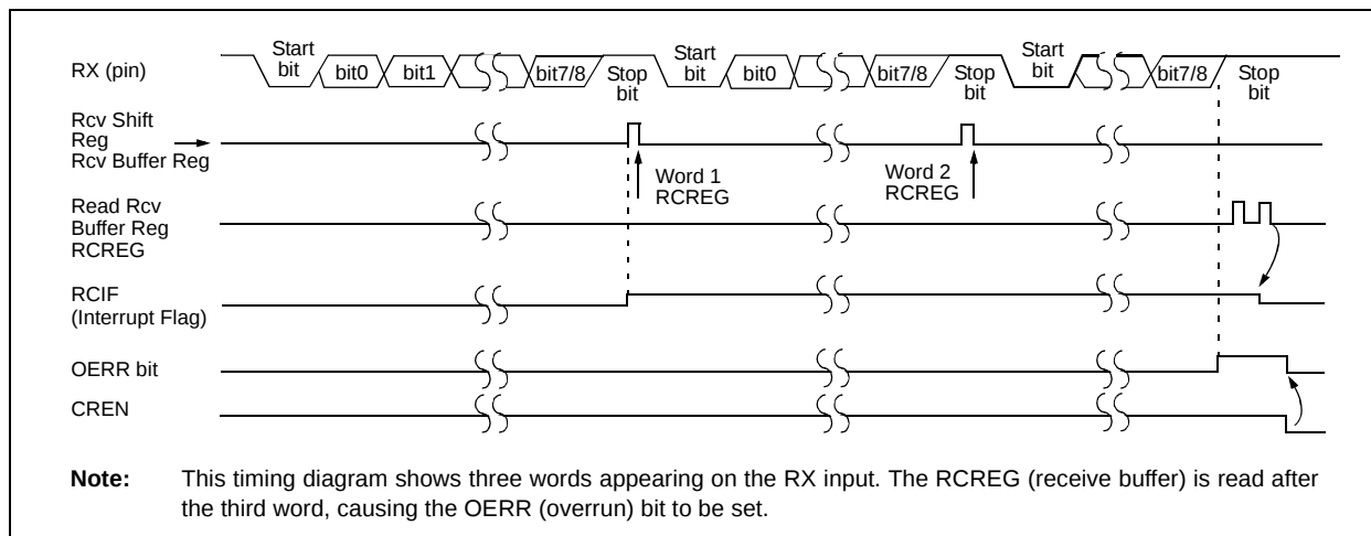
FIGURE 19-6: ASYNCHRONOUS RECEPTION
