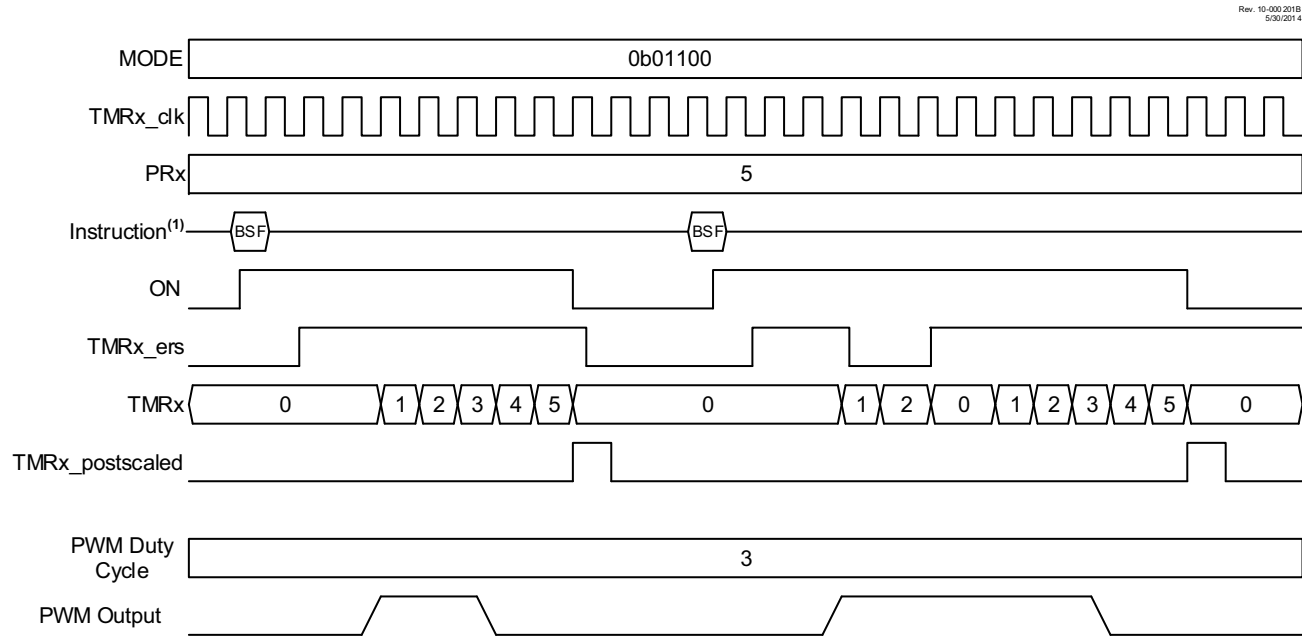
FIGURE 20-10: EDGE-TRIGGERED HARDWARE LIMIT ONE-SHOT TIMING DIAGRAM
