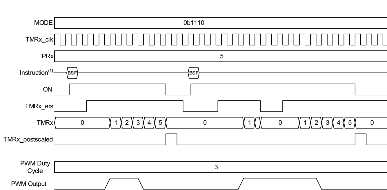
FIGURE 20-11: LEVEL-TRIGGERED HARDWARE LIMIT ONE-SHOT MODE TIMING DIAGRAM
