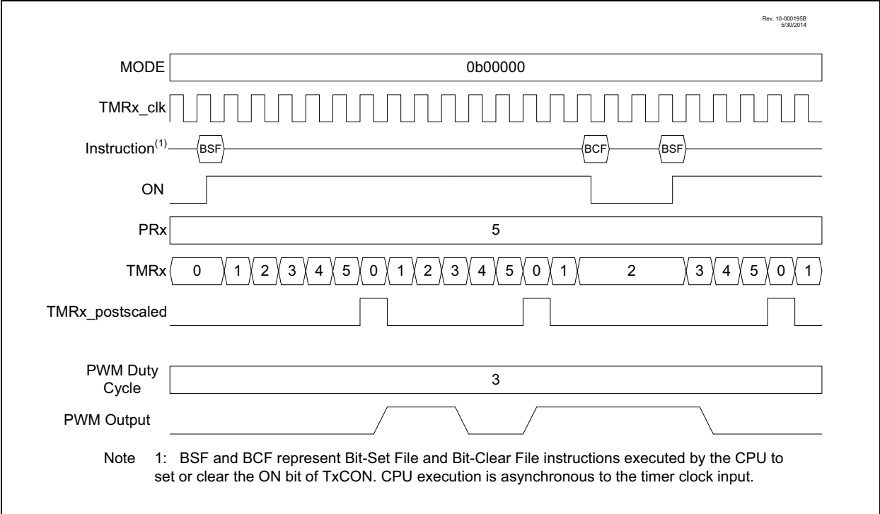
FIGURE 20-4: SOFTWARE GATE MODE TIMING DIAGRAM
