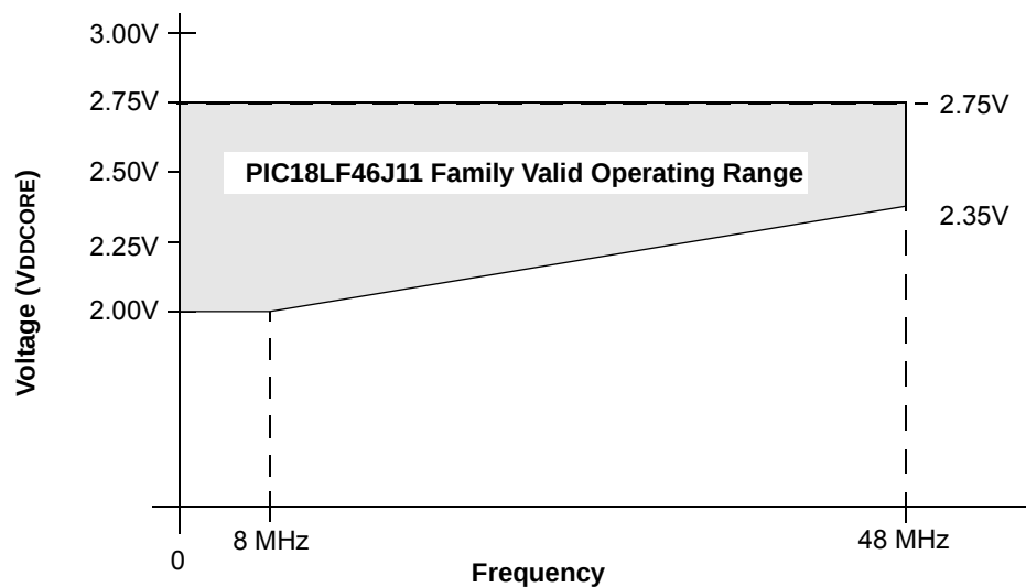
FIGURE 29-2: PIC18LF46J11 V DDCORE FREQUENCY GRAPH (INDUSTRIAL) (1)
