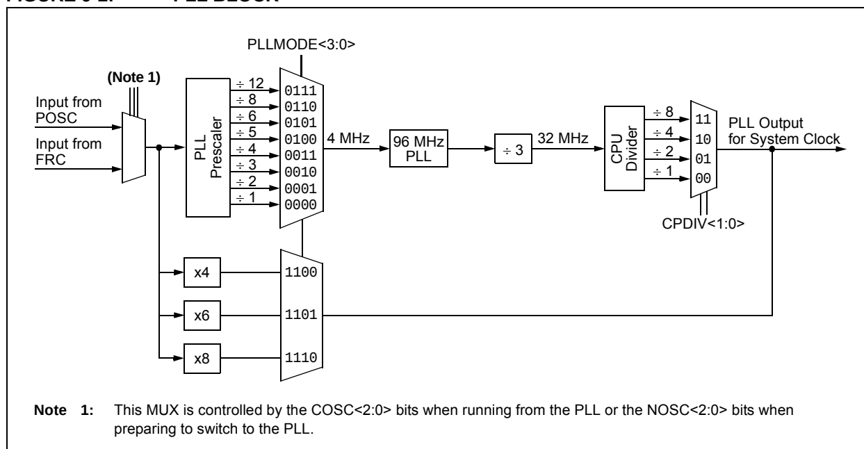
FIGURE 9-2: PLL BLOCK
