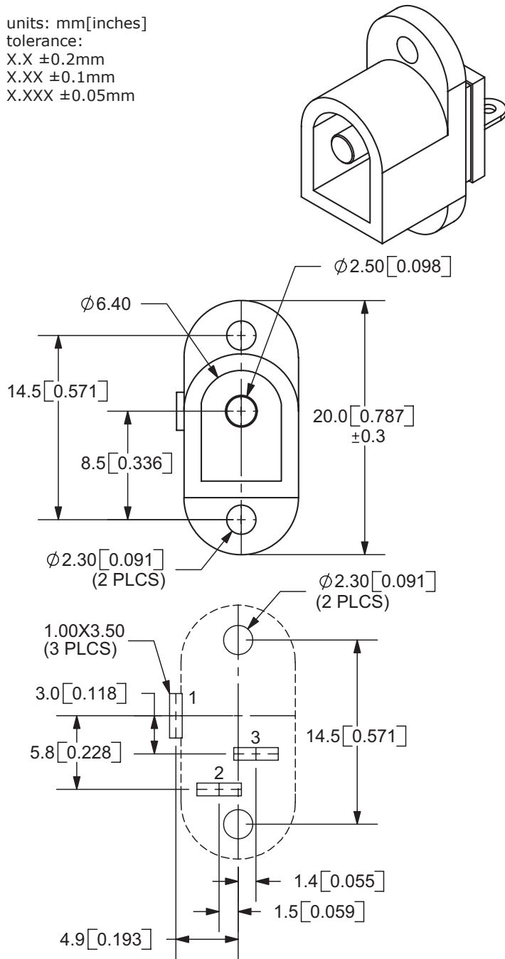
PCB LAYOUT FRONT VIEW
