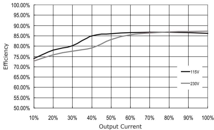
Efficiency vs. Output Current (PLDS60-A-277)
