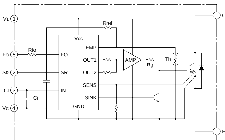
Outline Drawing and Circuit Diagram
