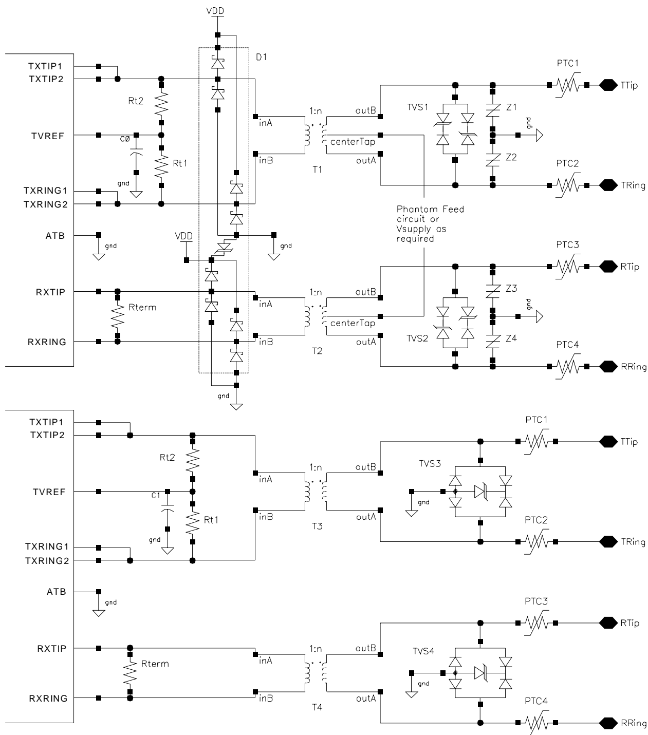
Figure 5 gives the recommended external protection circuitry for two cases:
