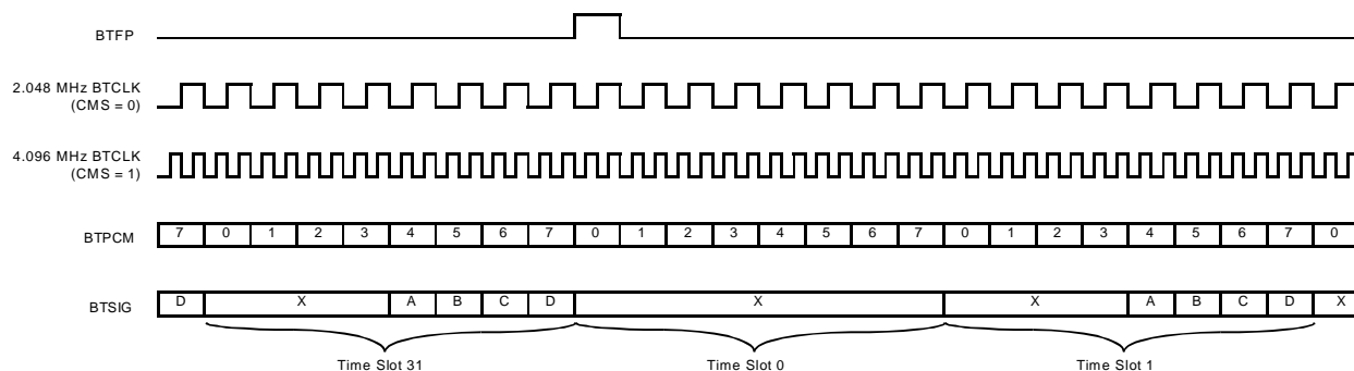
Figure 21 - Transmit Backplane at 2.048 Mbit/s (E1 mode)
