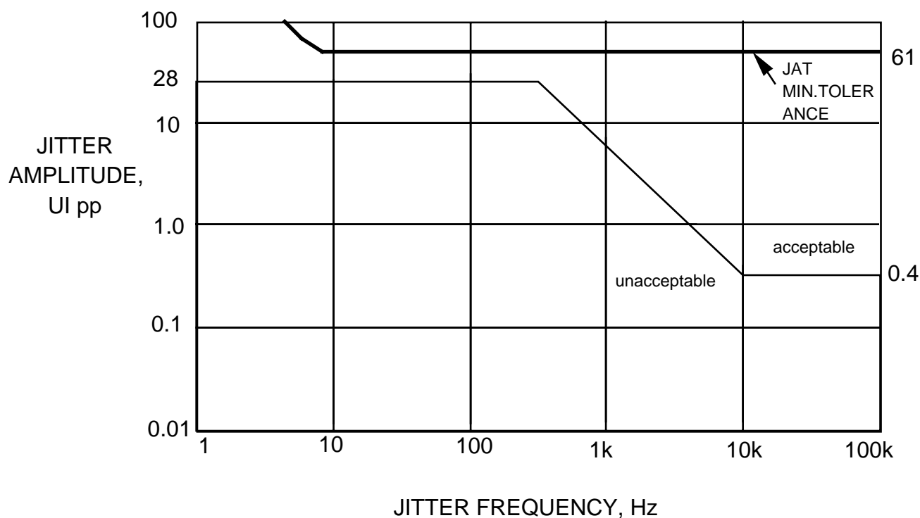
Figure 9 - TJAT Jitter Tolerance
