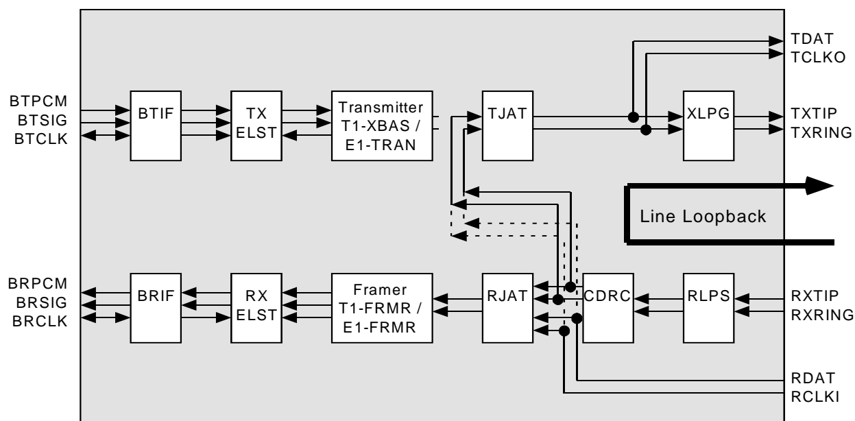
Figure 39 - Line Loopback
