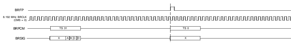
Figure 34 - Receive Backplane at 8.192 Mbit/s (E1 Mode)
