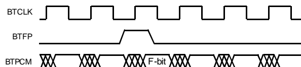
Figure 15 - Transmit Backplane: CMS=1, FE=1, DE=1, BTFP is Input
