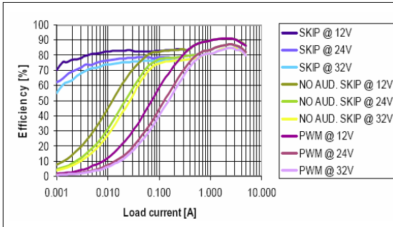
Figure 3. OUT1 = 3.3 V efficiency
