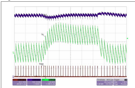
Figure 17. OUT1 = 3.3V load transient 0→2A
