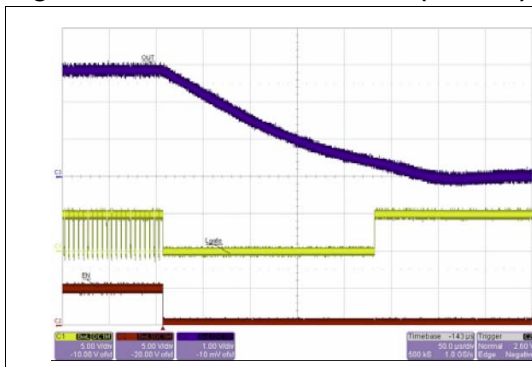
Figure 23. OUT1 = 3.3 V soft end (0.8 load)
