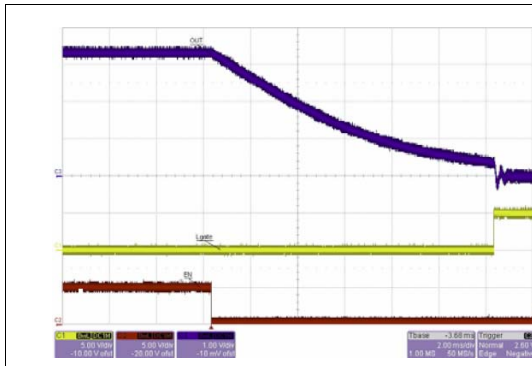
Figure 21. OUT1 = 3.3 V soft end (no load)
