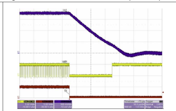
Figure 24. OUT2 = 1.8 V soft end (0.6 load)
