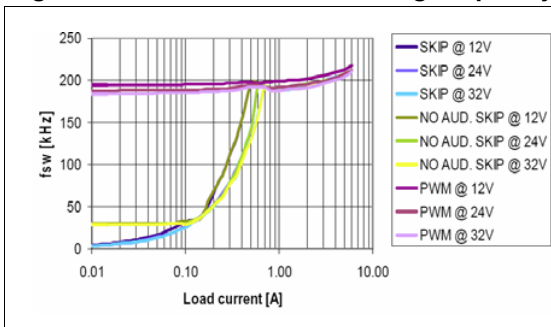
Figure 11. OUT1 = 3.3 V switching frequency
