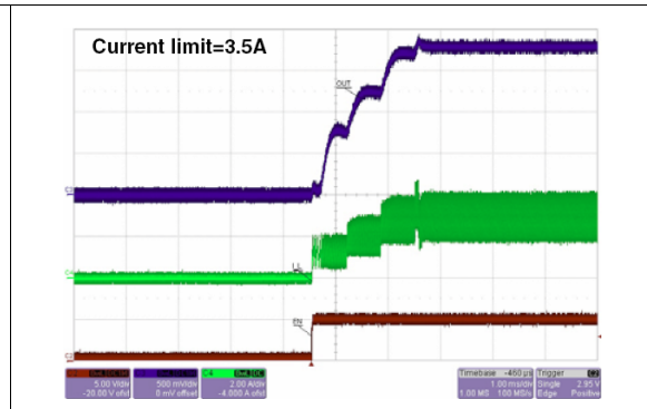
Figure 20. 1.8 V soft start (0.6Ω load)
