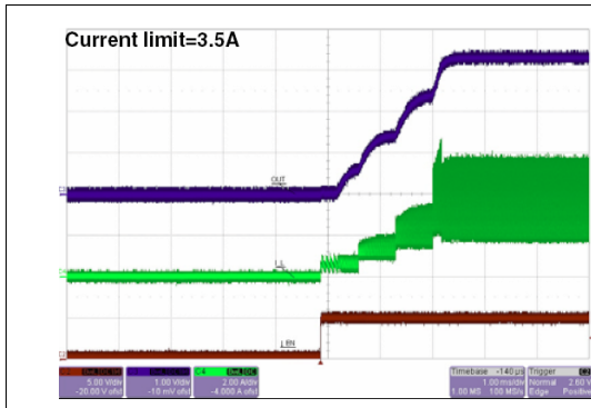
Figure 19. 3.3 V soft start (1Ω load)
