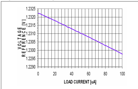
Figure 15. Voltage reference vs load current
