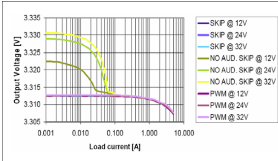
Figure 13. OUT1 = 3.3 V load regulation
