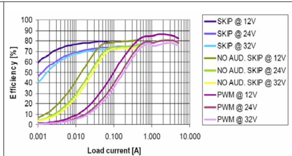
Figure 4. OUT2 = 1.8 V efficiency
