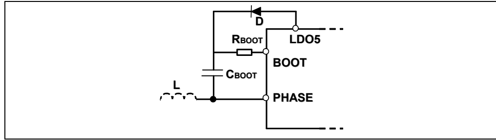
Figure 40. Bootstrap circuit
