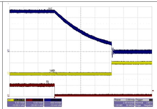
Figure 27. OUT2 = 1.8 V soft-end (0.6 \Omega load)
