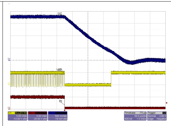
Figure 27. OUT2 = 1.8 V soft-end (0.6 \Omega load)
