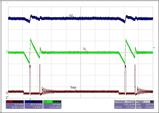
Figure 29. 1.8 V no-audible skip mode
