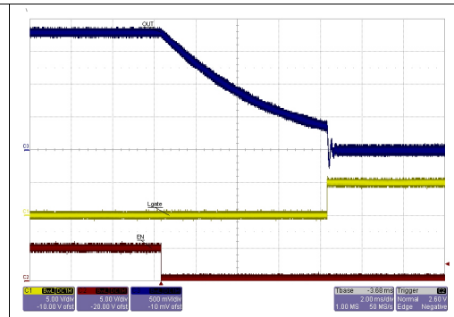
Figure 27. OUT2 = 1.8 V soft-end (0.6 \Omega load)
