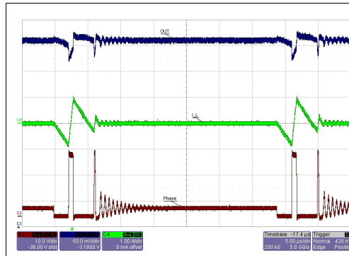
Figure 28. 3.3 V no-audible skip mode
