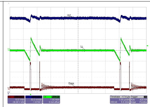
Figure 29. 1.8 V no-audible skip mode
