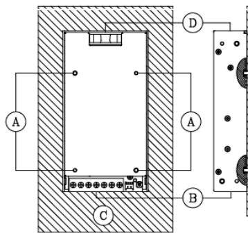
Fig. 2 Mounting Orientation
