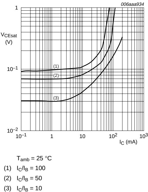
Fig 14. TR2: Collector-emitter saturation voltage as a function of collector current; typical values
