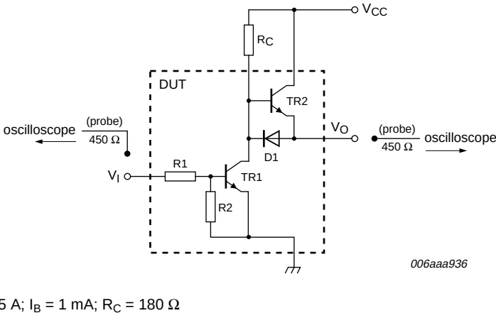
Fig 15. Test circuit for switching times
