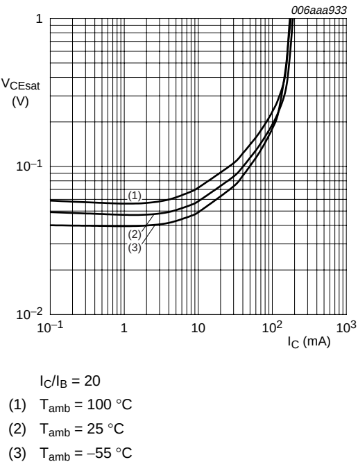
Fig 13. TR2: Collector-emitter saturation voltage as a function of collector current; typical values
