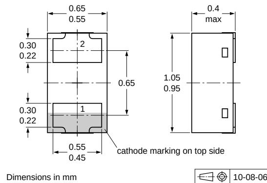
Fig 17. Package outline DFN1006D-2 (SOD882D)
