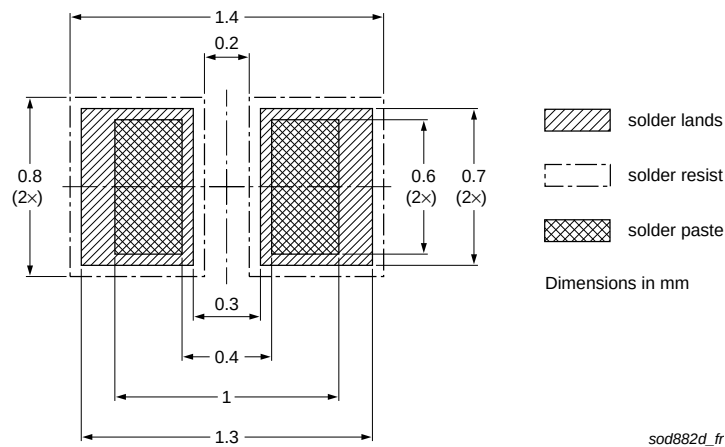
Fig 18. Reflow soldering footprint for DFN1006D-2 (SOD882D)
