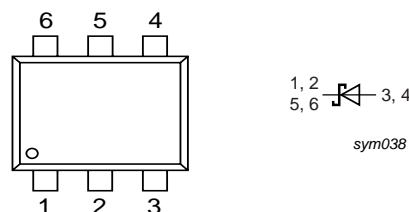
Fig.2 Simplified outline (SOT666) and symbol.
