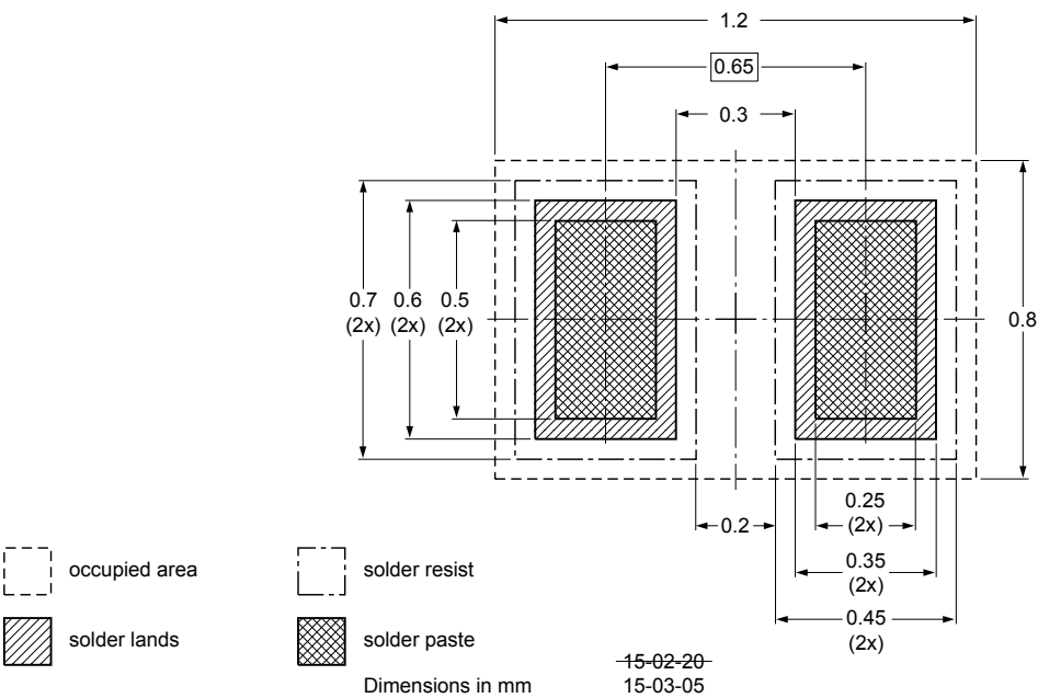
Fig. 16. Reflow soldering footprint for DSN1006-2 (SOD993)
