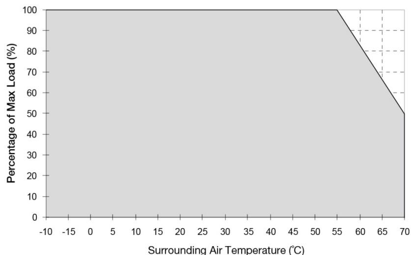
Fig. 1 De-rating for Vertical and Horizontal Mounting Orientation > 55°C de-rate power by 3.33% / °C
