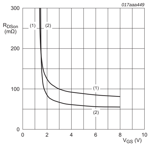
Fig 9. Drain-source on-state resistance as a function of gate-source voltage; typical values I_D = 1.8\text{ A} (1) T_j = 150\text{ }^\circ\text{C} (2) T_j = 25\text{ }^\circ\text{C}
