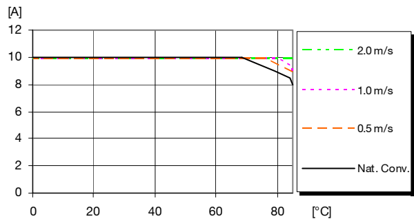
Output Current Derating
