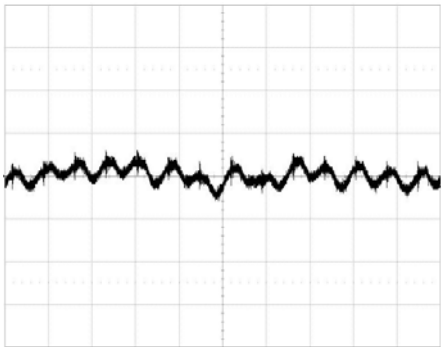
Output voltage ripple (5 mV/div.) at: T_{ref} = +25^{\circ}\text{C} , I_O = 60\text{ A} electrical load, V_i = 5\text{ V} . Time scale: 5 μs/div. Output capacitor: 660 μF electrolysis type. See the filter in the Output ripple and noise section (EMC Specification).
