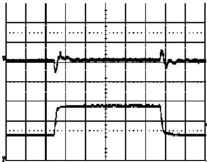
Output voltage response to load current step- change (30-60-30 A) at: T_{ref} = +25^{\circ}\text{C} , V_i = 5.0\text{ V} . Top trace: output voltage (100 mV/div.). Bottom trace: load current (20 A/div.). Time scale: 0.2 ms/div.
