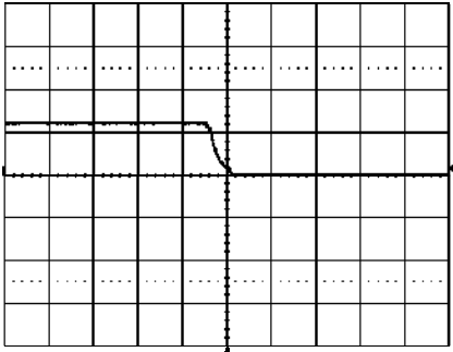
Shut-down enabled by disconnecting V_i at: T_{ref} = +25^{\circ}\text{C} , I_O = 60\text{ A} resistive load, V_i = 5.0\text{ V} . Top trace: output voltage (1.0 V/div.). Time scale: 0.5 ms/div.
