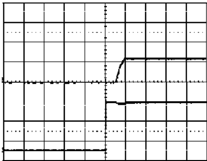
Start-up enabled by connecting V_i at: T_{ref} = +25^{\circ}\text{C} , I_O = 60\text{ A} resistive load, V_i = 5.0\text{ V} . Top trace: output voltage (1.0 V/div.). Bottom trace: input voltage (2.0 V/div.). Time scale: 10 ms/div.
