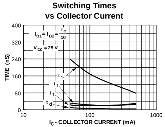
Figure 8. Switching Times vs Collector Current
