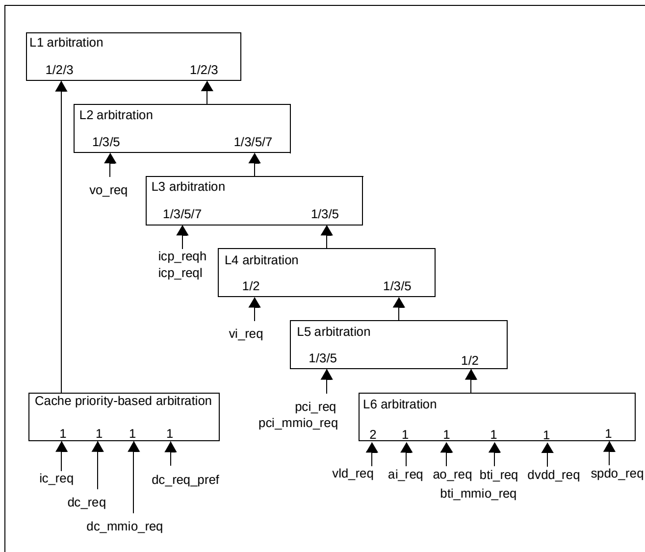
Figure 20-5. Arbitration architecture
