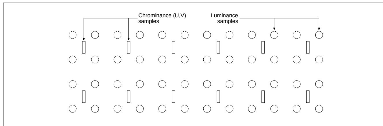
Figure 7-21. YUV 4:2:0 format.
