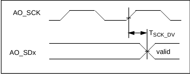
Figure 1-21. Audio Out I/O Timing
