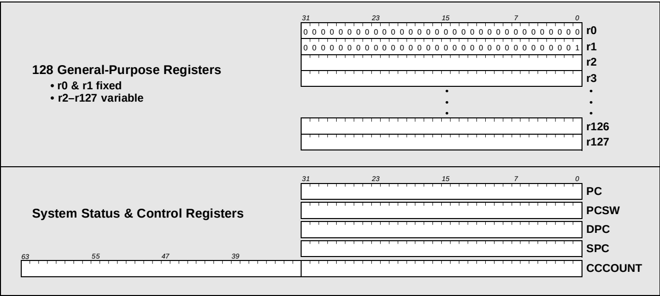
Figure 3-1. PNX1300 registers.
