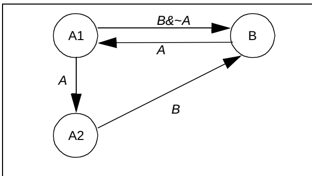
Figure 20-3. State diagram of round robin arbitrator with 2 requesters; A has double weight.
