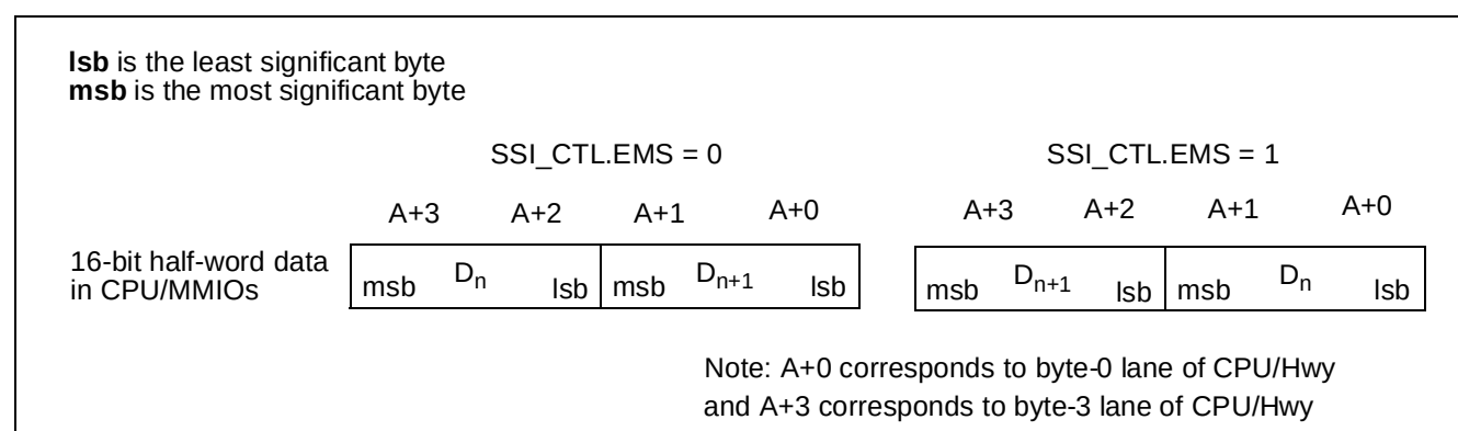
Figure C-15. SSI data format as seen in highway
