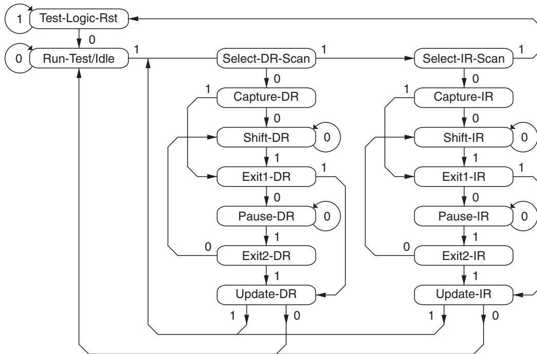
Figure 4-18. TAP States
