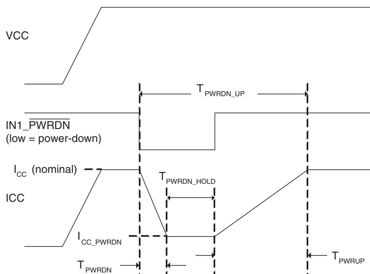
Figure 4-3. Power-Down Mode Timing
