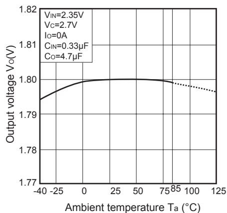
Fig.17 Output Voltage vs. Ambient Temperature (PQ018EF02SZH)
