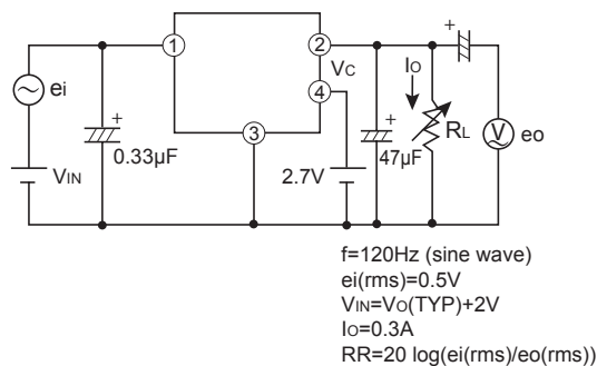
Fig.2 Test Circuit of Ripple Rejection
