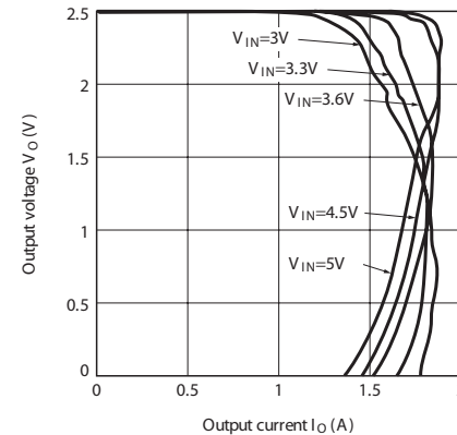
Fig.6 Overcurrent Protection Characteristics (Typical Value) (PQ025EH01ZxH)
