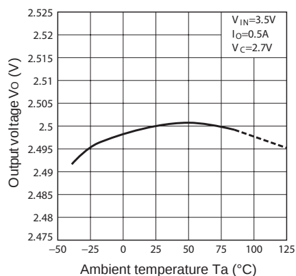
Fig.9 Output Voltage vs. Ambient Temperature (PQ025EH01ZxH)
