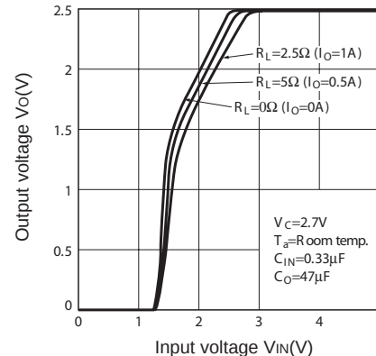
Fig.12 Output Voltage vs. Input Voltage (PQ025EH01ZxH)
