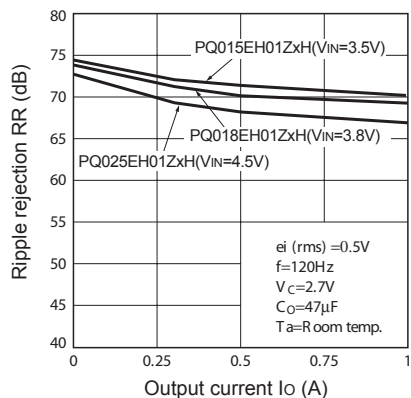
Fig.19 Ripple Rejection vs. Output Current
