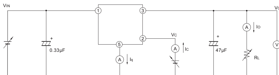
Fig.1 Test Circuit
