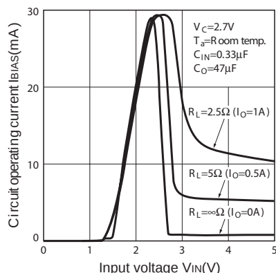
Fig.15 Circuit Operating Current vs. Input Voltage (PQ025EH01ZxH)
