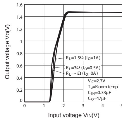
Fig.10 Output Voltage vs. Input Voltage (PQ015EH01ZxH)
