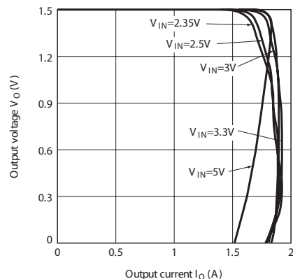
Fig.4 Overcurrent Protection Characteristics (Typical Value) (PQ015EH01ZxH)
