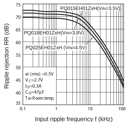
Fig.18 Ripple Rejection vs. Input Ripple Frequency
