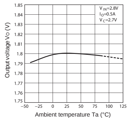
Fig.8 Output Voltage vs. Ambient Temperature (PQ018EH01ZxH)
