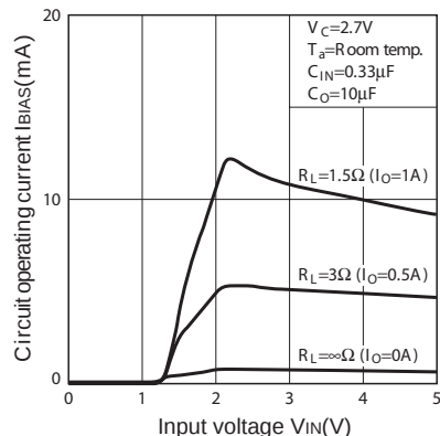
Fig.13 Circuit Operating Current vs. Input Voltage (PQ015EH01ZxH)
