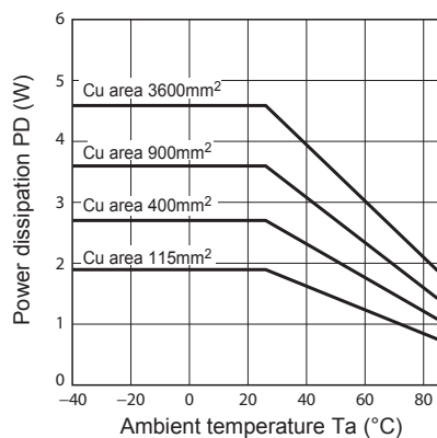
Fig.20 Power Dissipation vs. Ambient Temperature (Typical Value)
