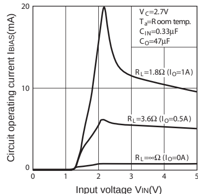
Fig.14 Circuit Operating Current vs. Input Voltage (PQ018EH01ZxH)
