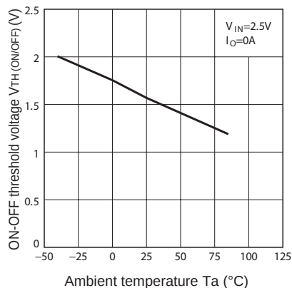
Fig.17 ON-OFF Threshold Voltage vs. Ambient Temperature (PQ018EH01ZxH)
