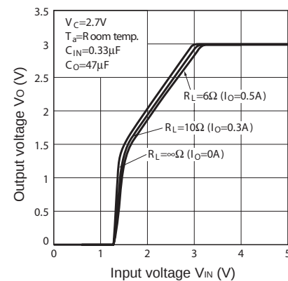
Fig.22 Output Voltage vs. Input Voltage (PQ030EZ5MZxH)
