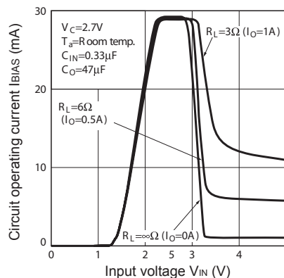
Fig.37 Circuit Operating Current vs. Input Voltage (PQ030EZ01ZxH)
