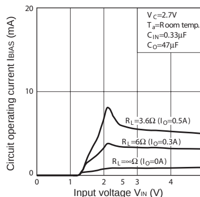
Fig.30 Circuit Operating Current vs. Input Voltage (PQ018EZ5MZxH)
