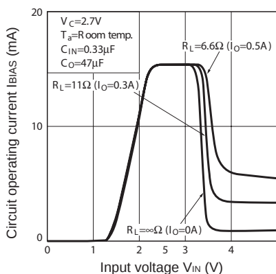
Fig.33 Circuit Operating Current vs. Input Voltage (PQ033EZ5MZxH)
