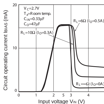
Fig.32 Circuit Operating Current vs. Input Voltage (PQ030EZ5MZxH)
