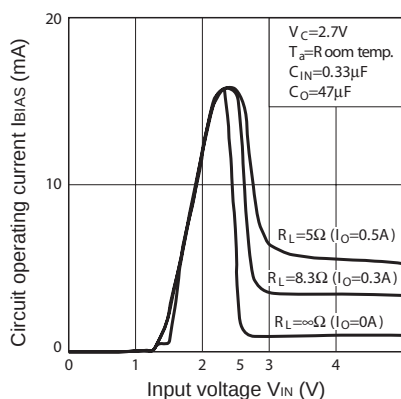
Fig.31 Circuit Operating Current vs. Input Voltage (PQ025EZ5MZxH)
