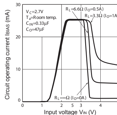
Fig.38 Circuit Operating Current vs. Input Voltage (PQ033EZ01ZxH)
