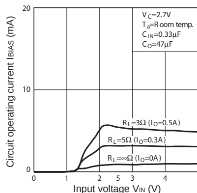
Fig.29 Circuit Operating Current vs. Input Voltage (PQ015EZ5MZxH)
