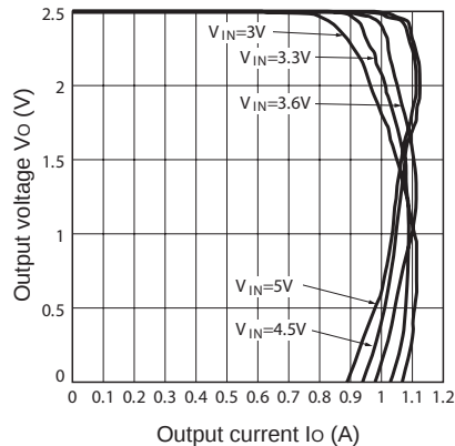
Fig.6 Overcurrent Protection Characteristics (PQ025EZ5MZxH)
