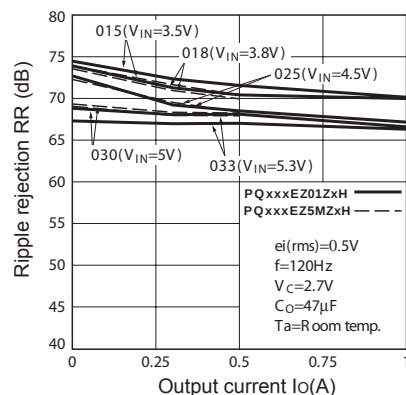
Fig.42 Ripple Rejection vs. Output Current
