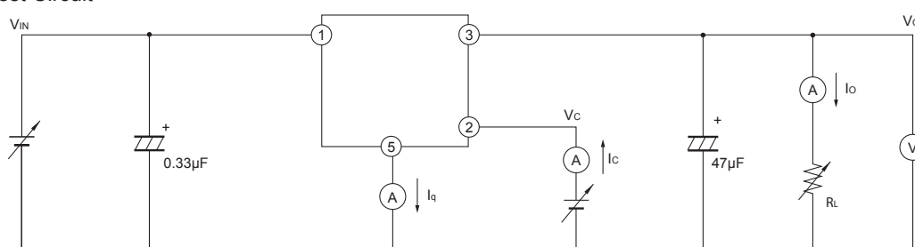
Fig.1 Test Circuit
