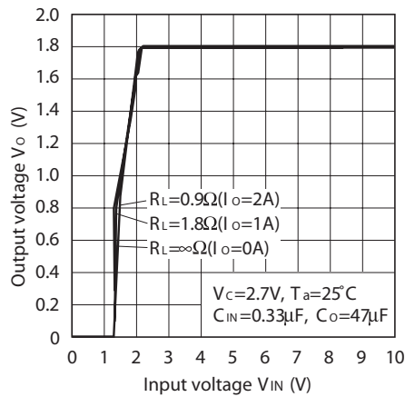
Fig.11 Output Voltage vs. Input Voltage (PQ018EH02ZxH)
