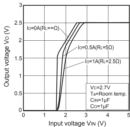
Fig.19 Output Voltage vs. Input Voltage (PQ025ENA1ZPH)
