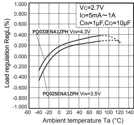
Fig.13 Load Regulation vs. Ambient Temperature
