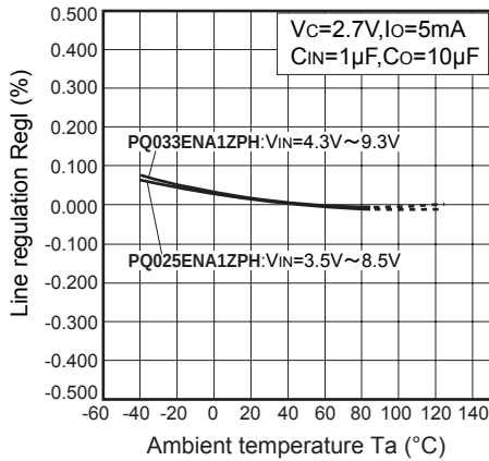
Fig.12 Line Regulation vs. Ambient Temperature
