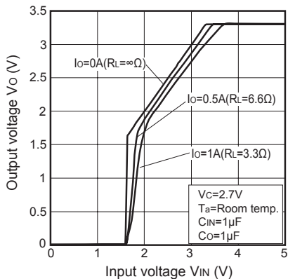
Fig.20 Output Voltage vs. Input Voltage (PQ033ENA1ZPH)
