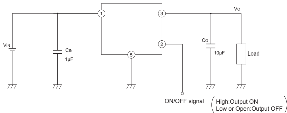
Fig.1 Typical Application
