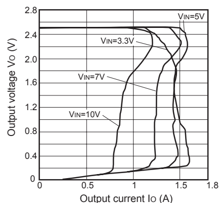
Fig.7 Overcurrent Protection Characteristics (PQ025ENA1ZPH)
