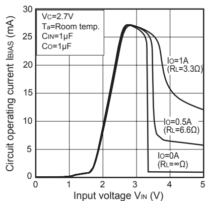
Fig.22 Circuit Operating Current vs. Input Voltage (PQ033ENA1ZPH)
