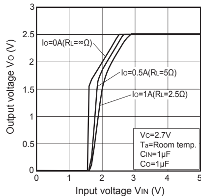
Fig.19 Output Voltage vs. Input Voltage (PQ025ENA1ZPH)
