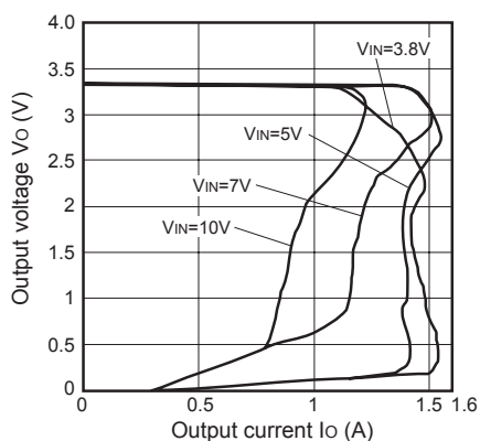
Fig.8 Overcurrent Protection Characteristics (PQ033ENA1ZPH)
