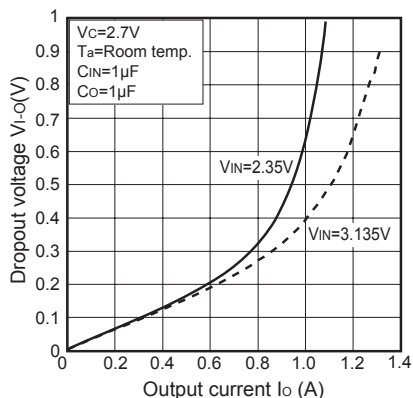
Fig.24 Dropout Voltage vs. Output Current (PQ033ENA1ZPH)
