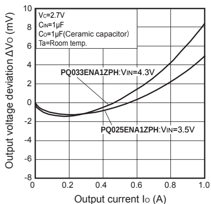
Fig.18 Output Voltage Deviation vs. Output Current
