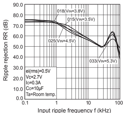
Fig.25 Ripple Rejection vs. Input Ripple Frequency (PQxxxENA1ZPH)
