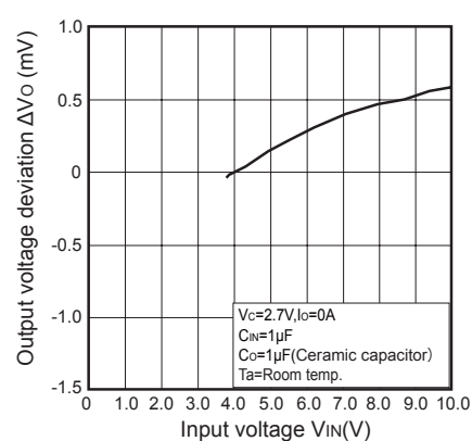
Fig.17 Output Voltage Deviation vs. Input Voltage (PQ033ENA1ZPH)
