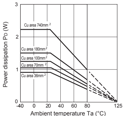
Fig.27 Power Dissipation vs. Ambient Temperature (Typical Value)
