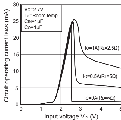
Fig.21 Circuit Operating Current vs. Input Voltage (PQ025ENA1ZPH)
