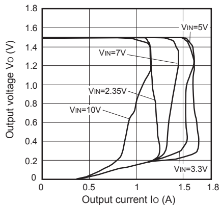
Fig.5 Overcurrent Protection Characteristics (PQ015ENA1ZPH)
