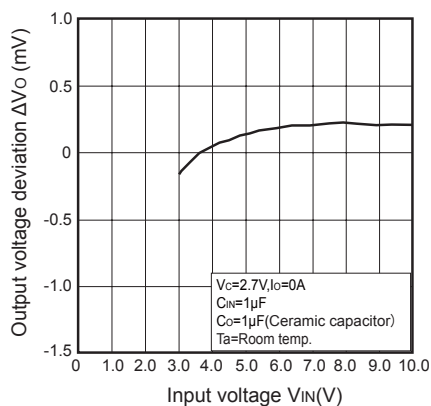
Fig.16 Output Voltage Deviation vs. Input Voltage (PQ025ENA1ZPH)
