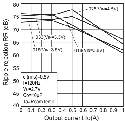
Fig.26 Ripple Rejection vs. Output Current (PQxxxENA1ZPH)
