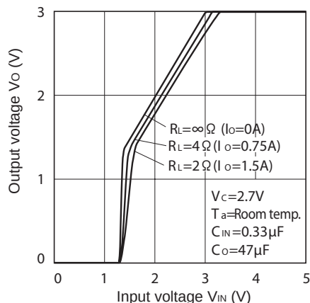
Fig.17 Output Voltage vs. Input Voltage (PQ030EZ1HZxH)
