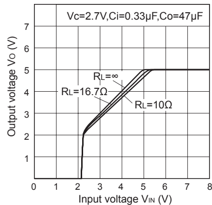
Fig.18 Output Voltage vs. Input Voltage (Typical Value) (PQ05DZ51J00H)
