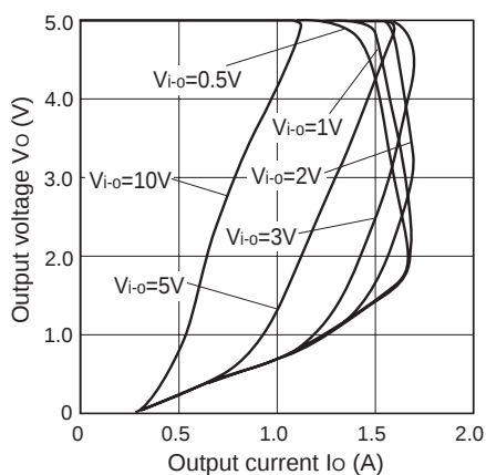
Fig.9 Overcurrent Protection Characteristics (Typical Value) (PQ05DZ11J00H)
