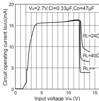
Fig.28 Circuit Operating Current vs. Input Voltage(PQ12DZ51J00H)
