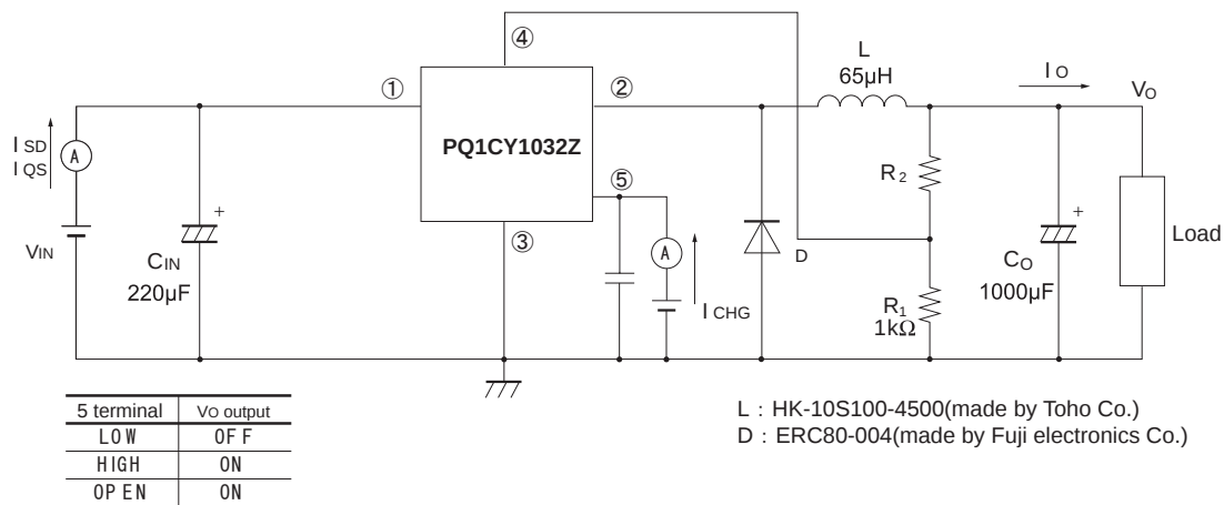
Fig.1 Test Circuit
