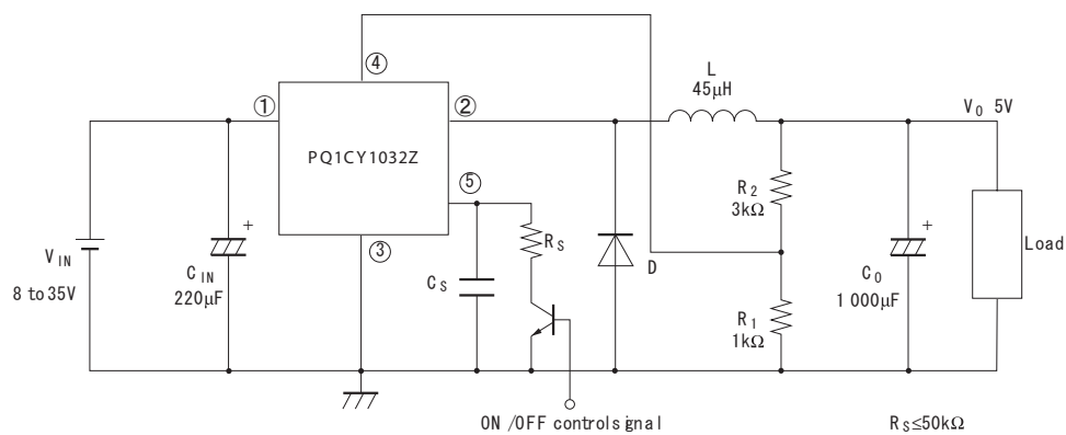
Fig.16 Step Down Type Circuit Diagram
