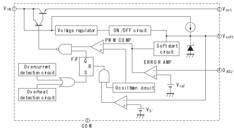
Fig.15 Block Diagram
