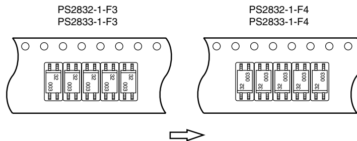
Tape Direction
