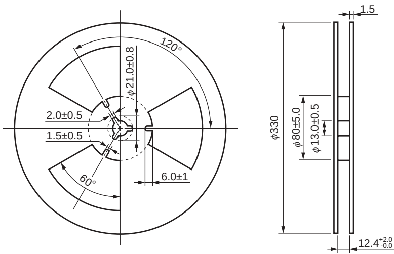
Reel Outline and Dimensions
