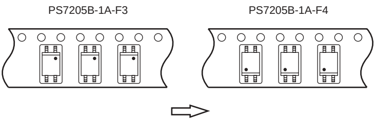
Reel Outline and Dimensions
