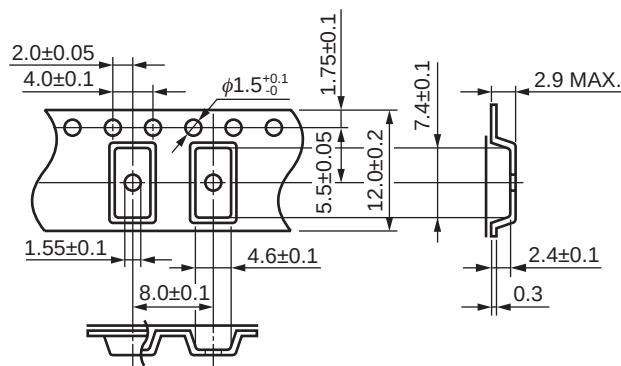
Tape Outline and Dimensions
