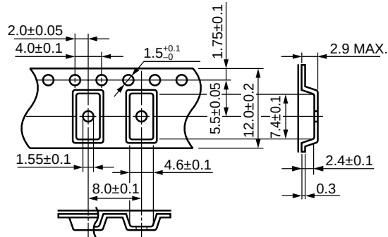
Outline and Dimensions (Tape)
