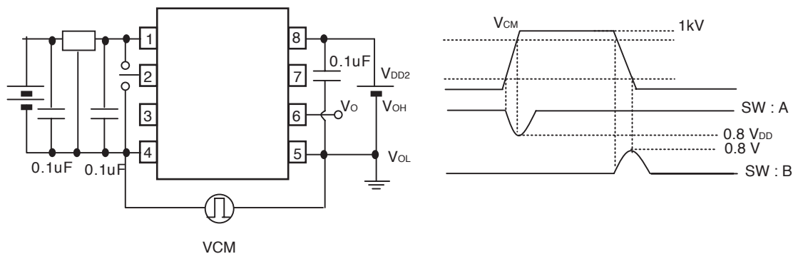
Fig. 10 C_{MH}/C_{ML}
