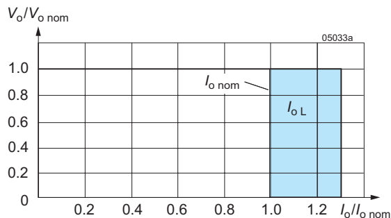
Fig. 6a Short-circuit behaviour V_o vs. I_o for regulators with V_{i\text{max}} \leq 80\text{ V}
