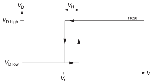
Fig. 15 Definition of V_t and V_H
