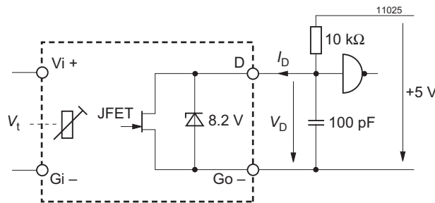
Fig. 14 Test circuit with definition of voltage V_D and current I_D
