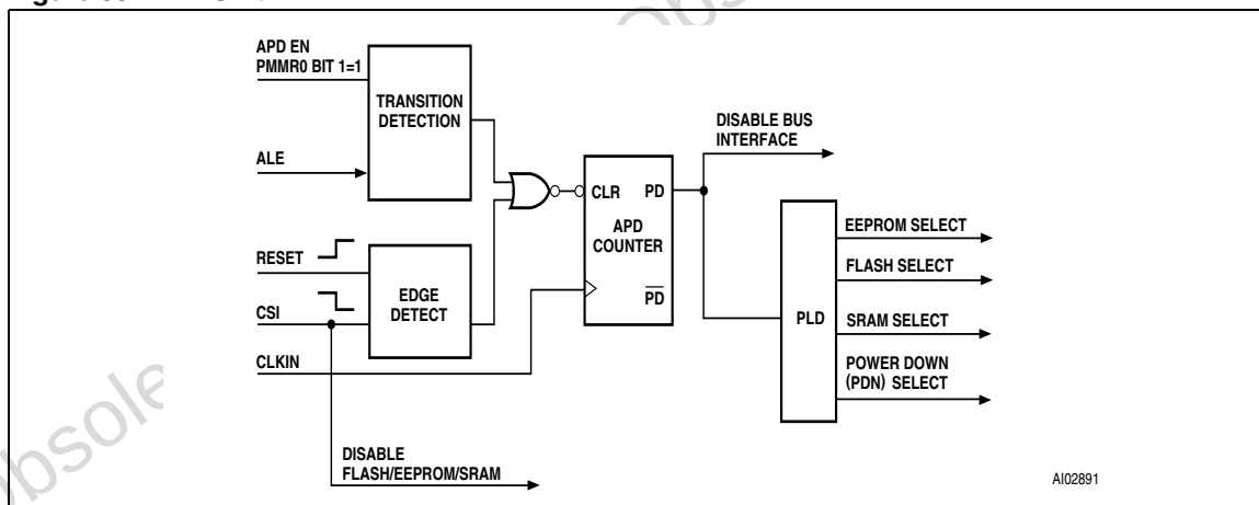
Figure 33. APD Unit
