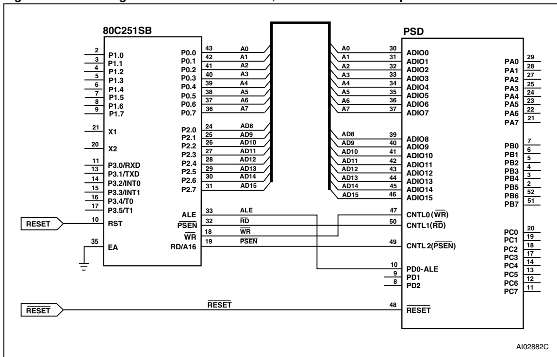
Figure 24. Interfacing the PSD with the 80C251, with \overline{\text{RD}} and \overline{\text{PSEN}} Inputs
