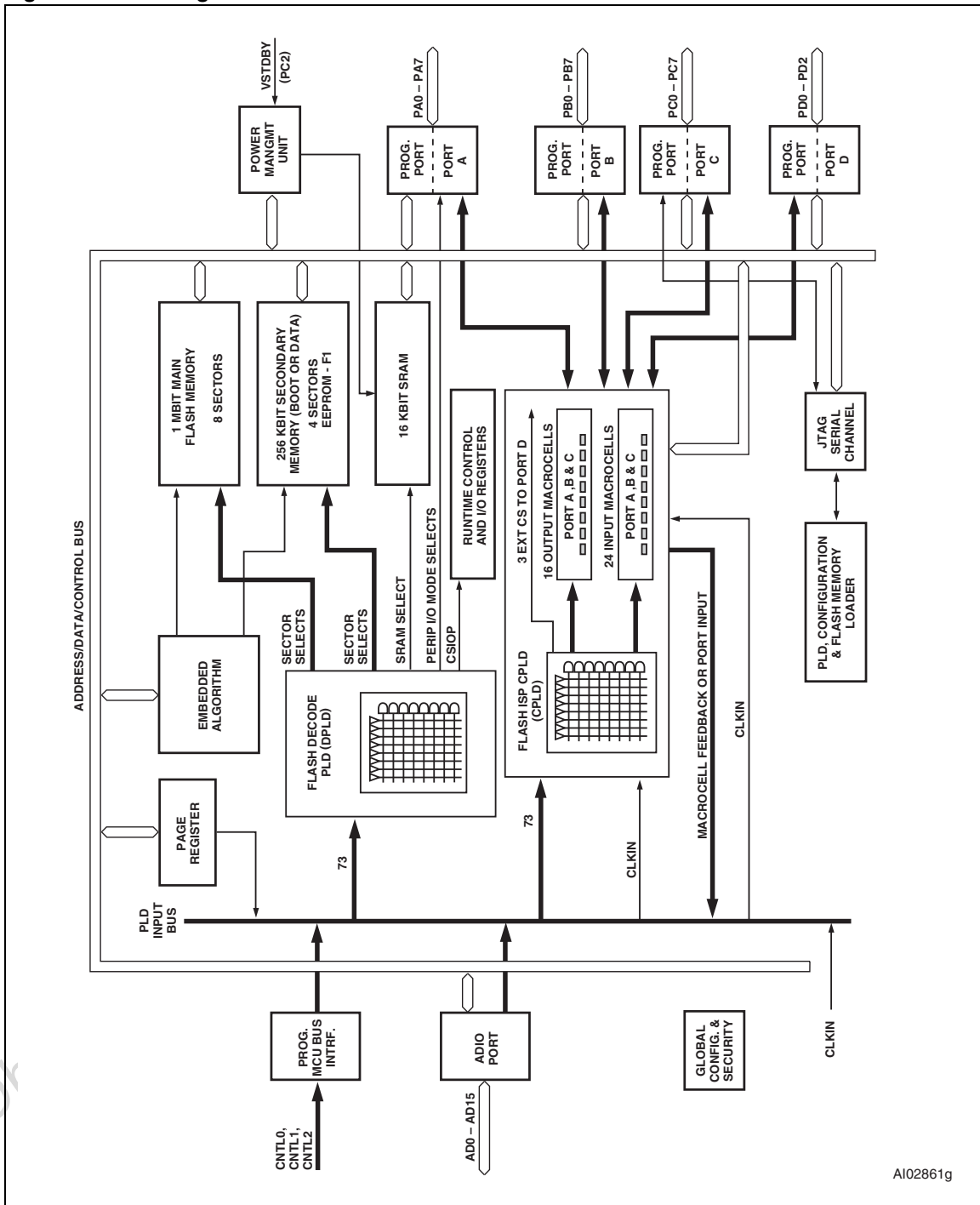
Figure 5. Block Diagram
