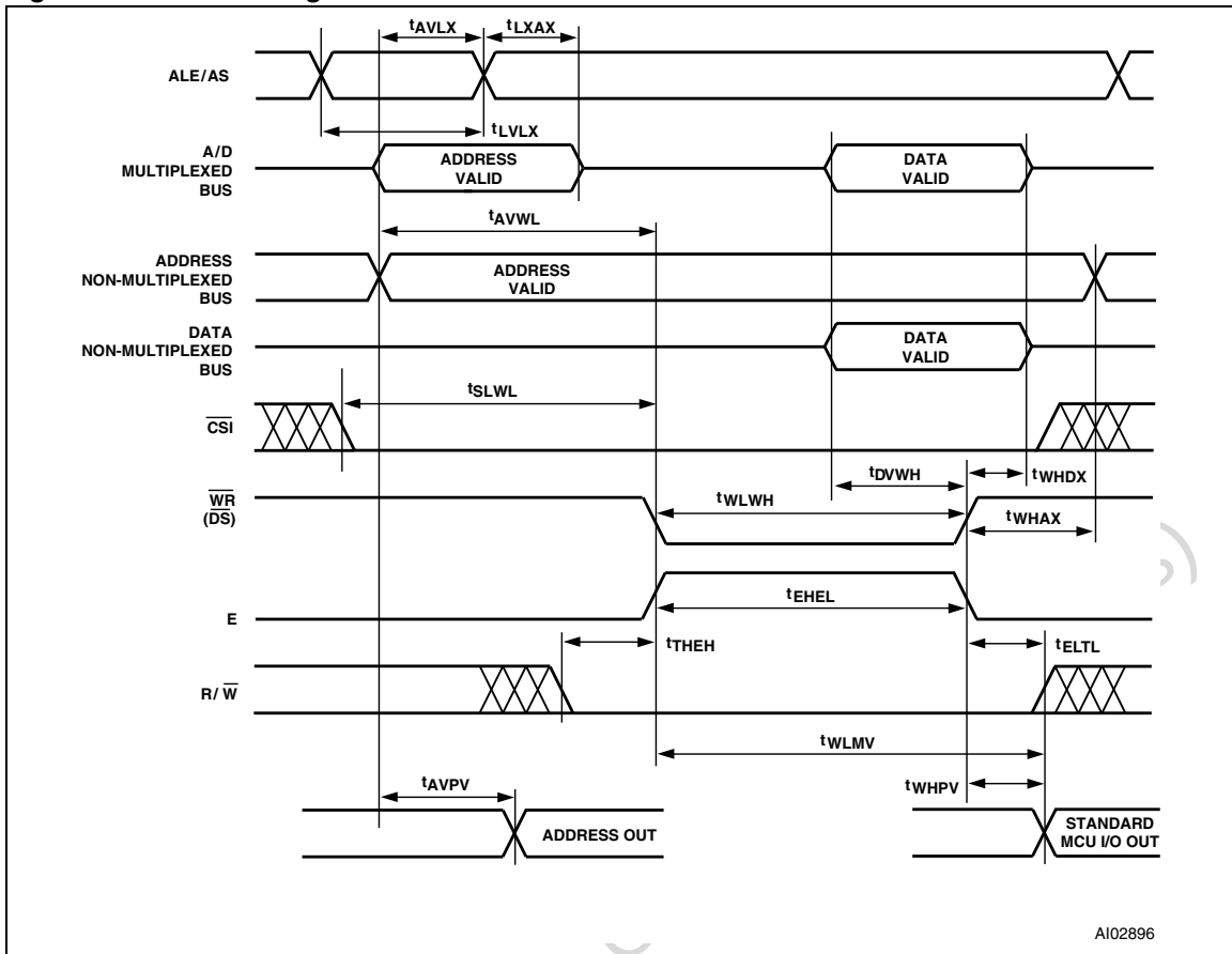
Figure 48. WRITE Timing
