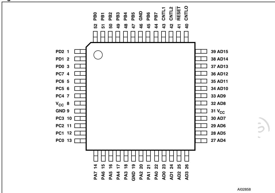
Figure 2. PQFP52 Connections
