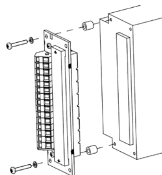
Fig. 23 Cage clamp adapter HZZ00144-G
