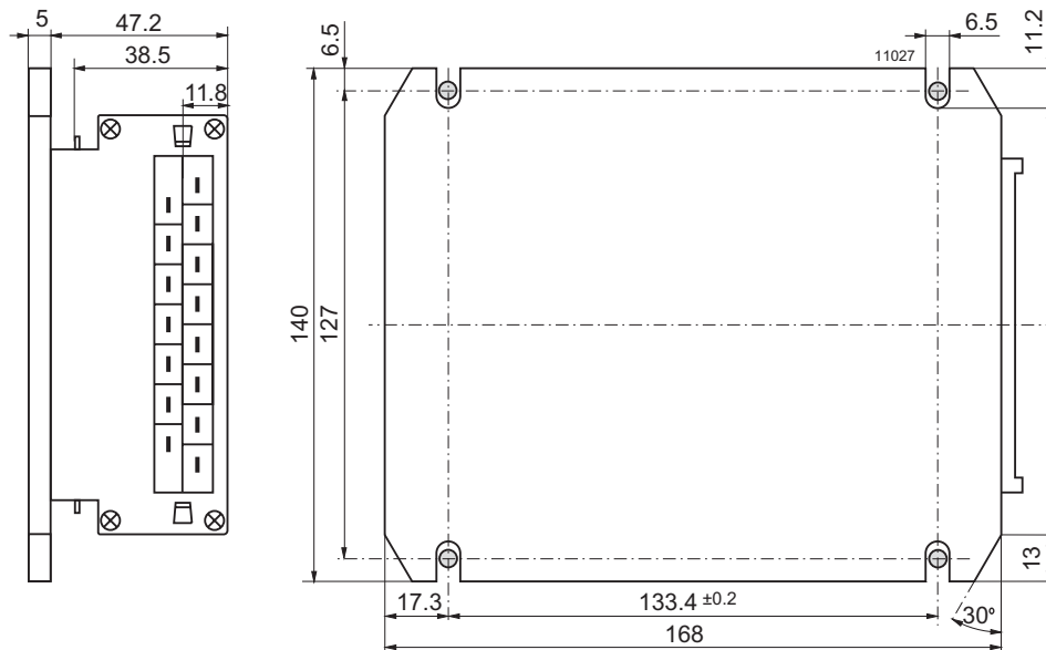
Fig. 15 Option B, large cooling plate Weight: 1.3 kg
