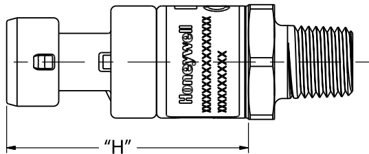
Figure 5. Electrical Connector Type Dimensions (For reference only: mm/[in].)
