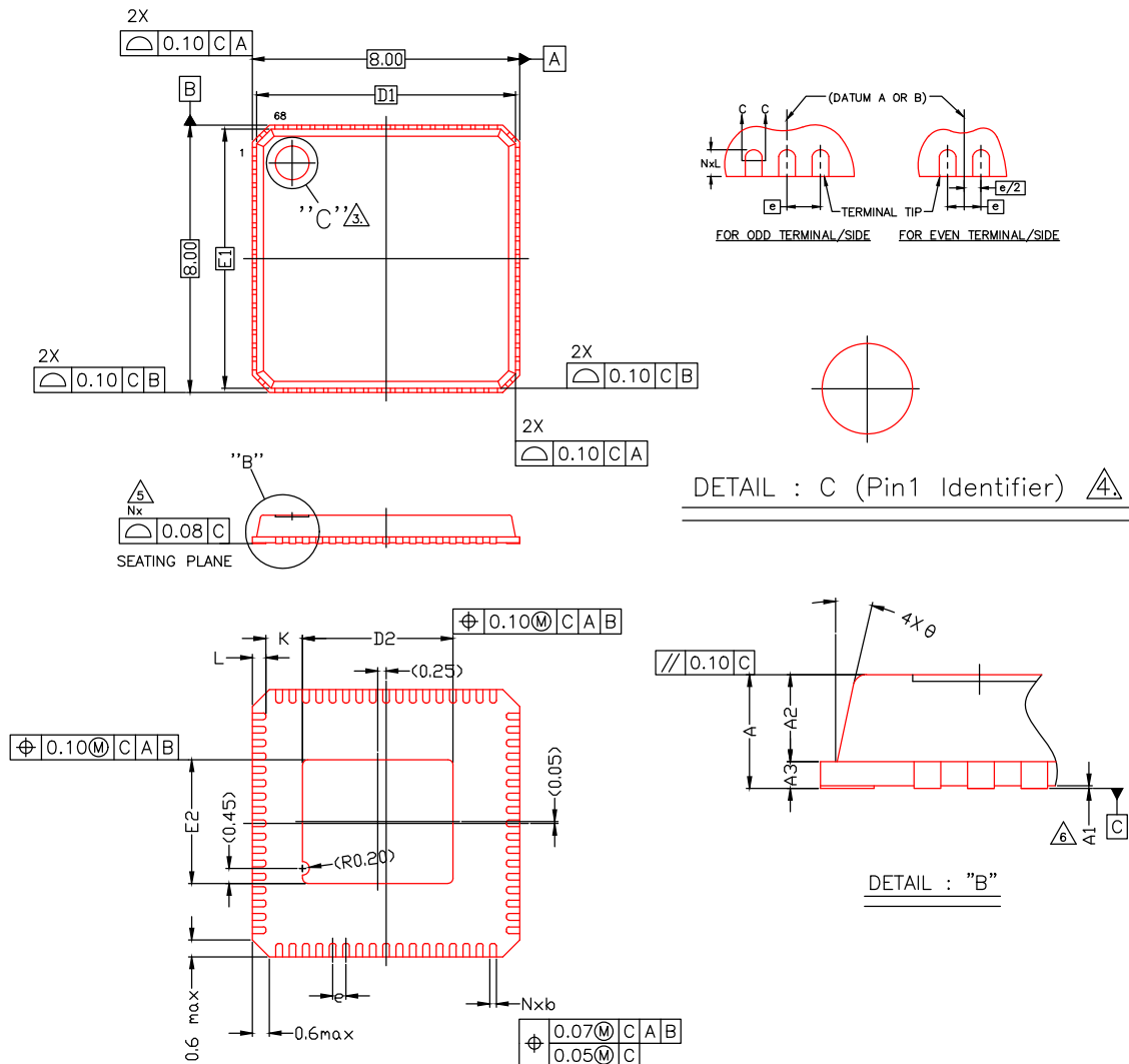
Figure 4-1 QCA4004 mechanical dimensions, top and bottom views
