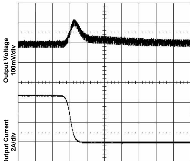
Time - t (100μs/div) Figure 7. Transient Load Response
