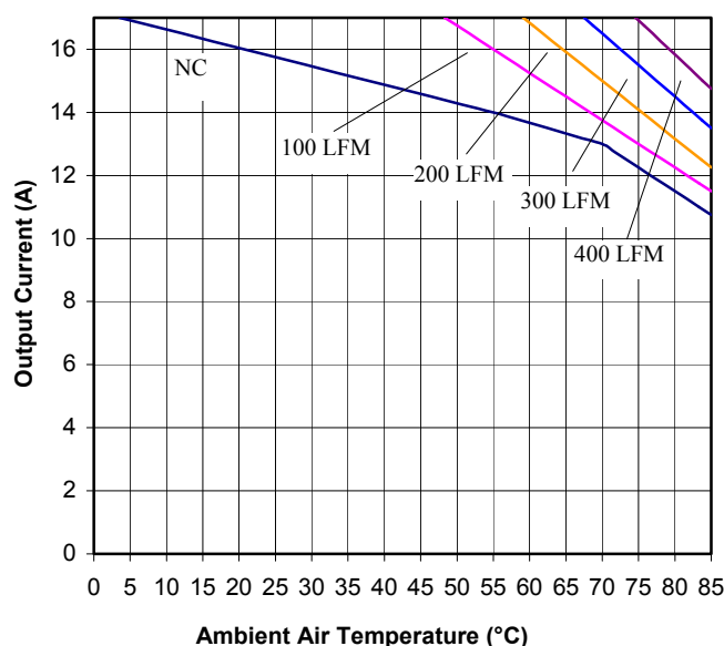
Figure 13. Current Derating Curve for Airflow Direction 2 (Ref. Fig. 14 for Airflow Direction; Vin = 24V open frame unit using socket interface)
