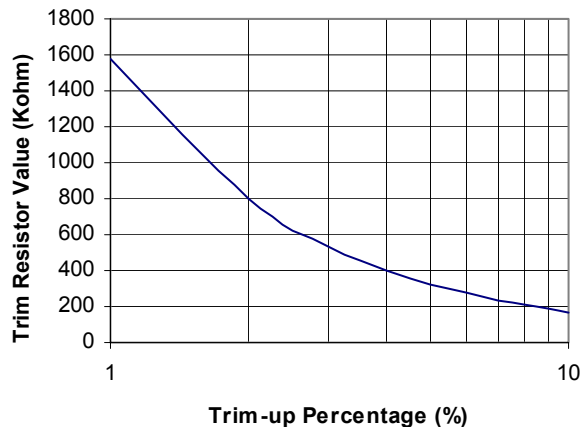
Fig. 19 Trim-up Resistor Selection
