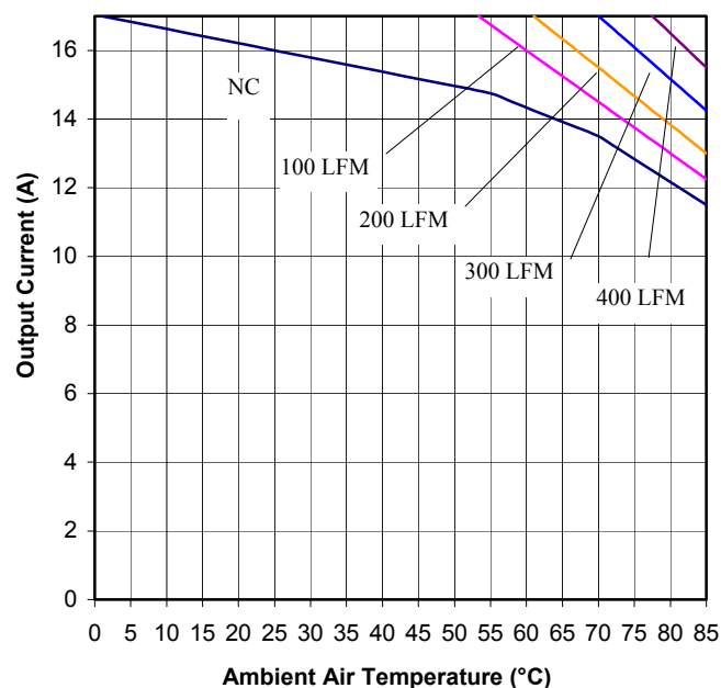
Figure 11. Current Derating Curve for Airflow Direction 3 (Ref. Fig. 12 for Airflow Direction; V_{in} = 24V open frame unit using socket interface)
