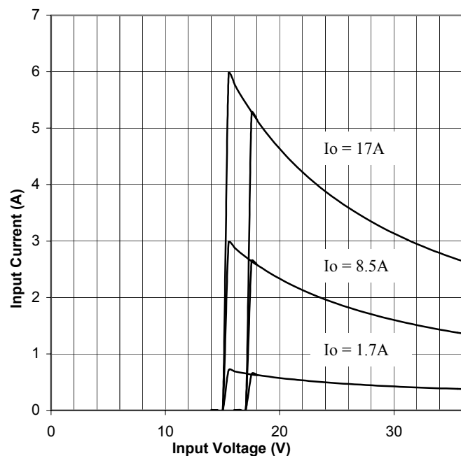
Figure 9. Input Characteristics
