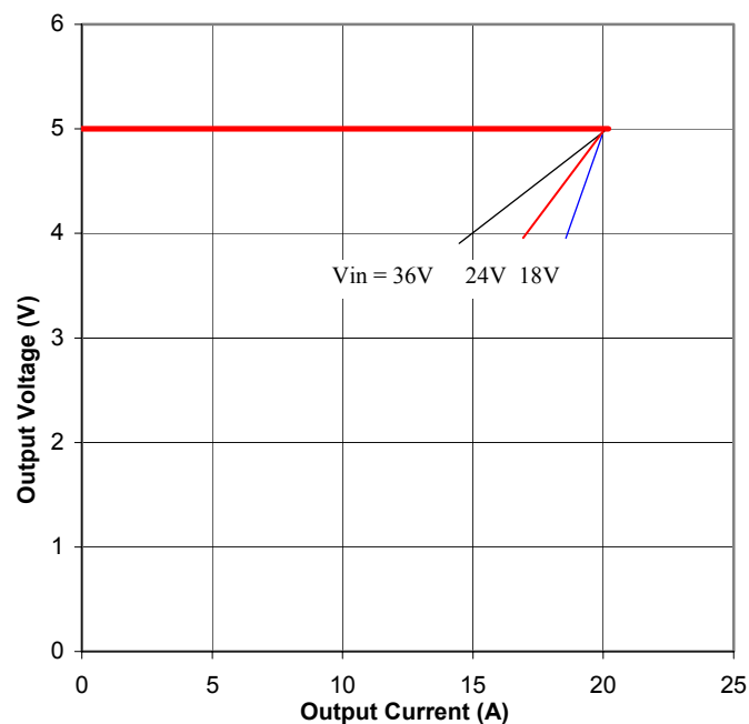
Figure 10. Output Characteristics
