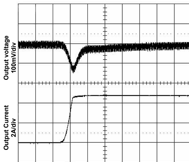
Time - t (100μs/div) Figure 8. Transient Load Response
