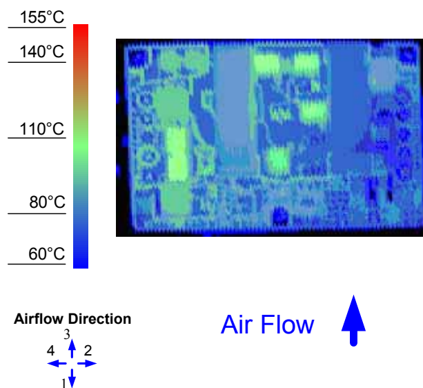
Figure 12. Thermal Image for Airflow Direction 3 (17A output, 55°C ambient, 200 LFM, V_{in} = 24V open frame unit using socket interface)
