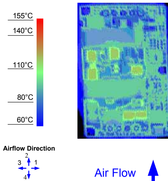
Figure 14. Thermal Image for Airflow Direction 2 (17A output, 55°C ambient, 200 LFM, Vin = 24V open frame unit using solder interface)
