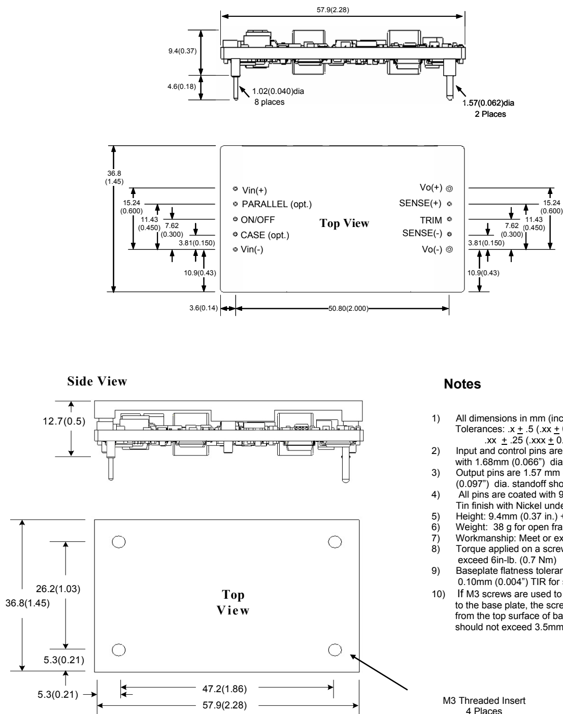
Figure 25. Converter with Optional Baseplate
