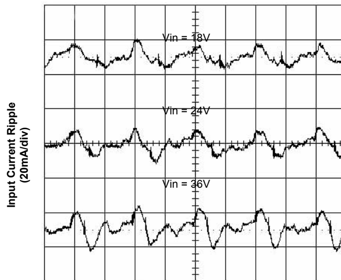
Time - t (2μs/div) Figure 6. Input Reflected Ripple Current at 17A Load
