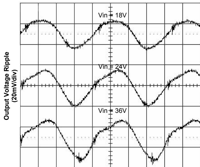
Time - t (1μs/div) Figure 5. Output Ripple Voltage at 17A Load
