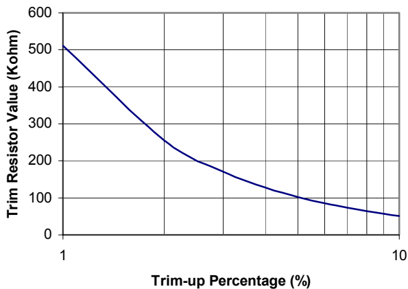
Fig. 19 Trim-Up Resistor Selection
