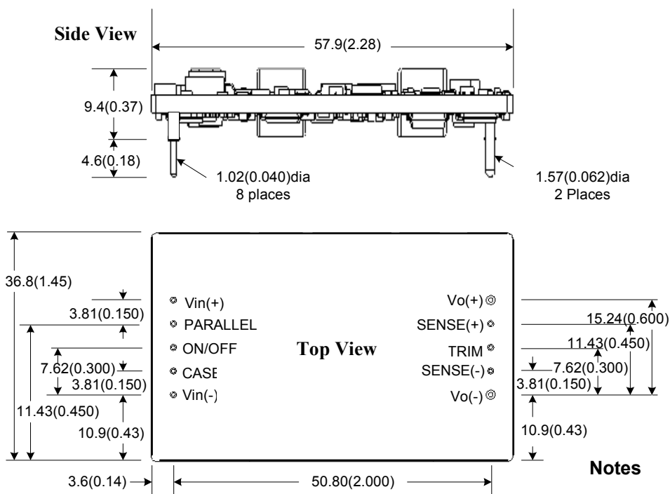
Figure 24. Open frame converter
