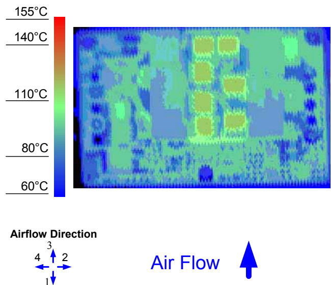
Figure 12. Thermal Image for Airflow Direction 3 (36.5A output, 55 ^{\circ}C ambient, 200 LFM, V_{in} = 48V open frame unit using socket interface)
