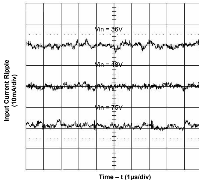
Figure 6. Input Reflected Ripple Current at 40A Load
