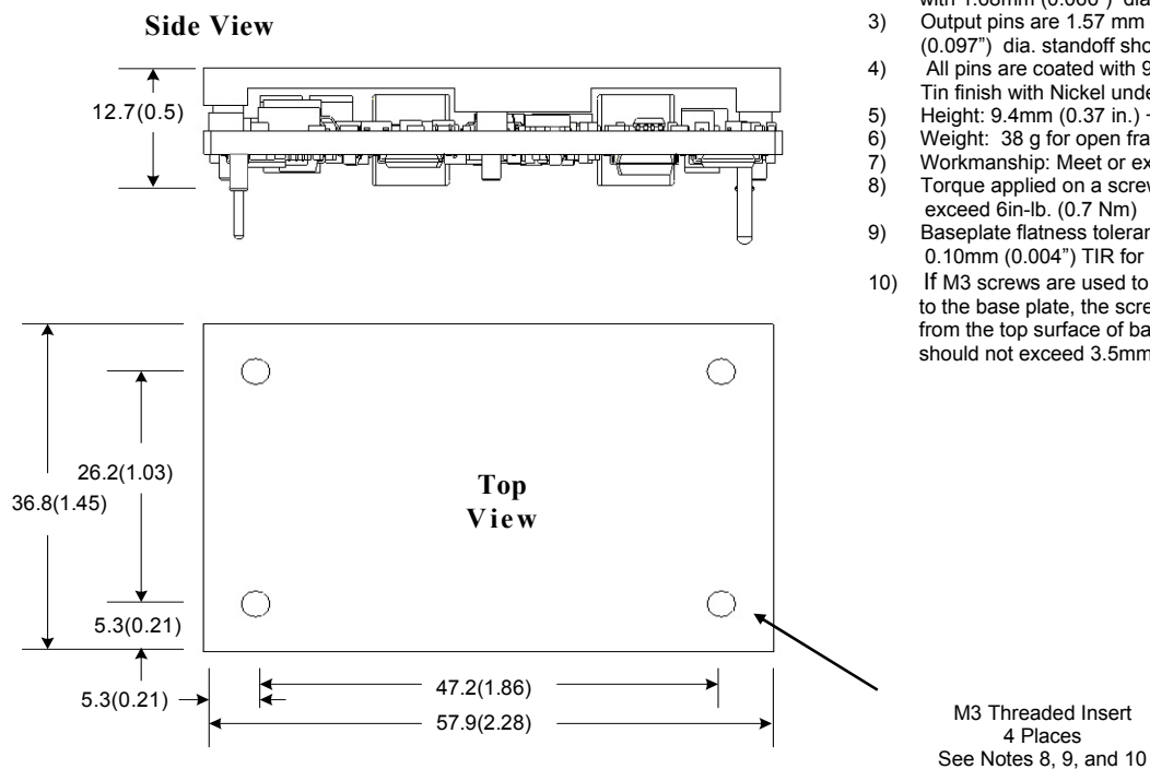
Figure 25. Converter with Optional Baseplate
