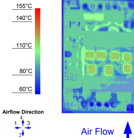
Figure 14. Thermal Image for Airflow Direction 4 (33A output, 55°C ambient, 200 LFM, Vin = 48V open frame unit using solder interface)
