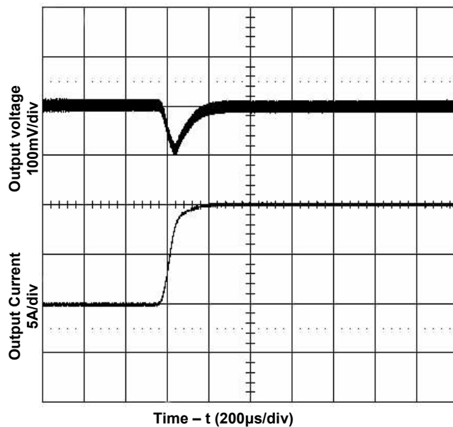
Figure 8. Transient Load Response
