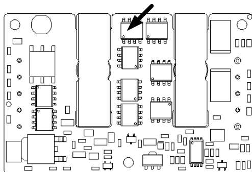
Figure 23. Temperature Monitoring Location
