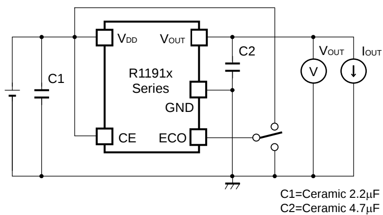
Basic Test Circuit
