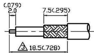
STRIPPING DIMENSION
