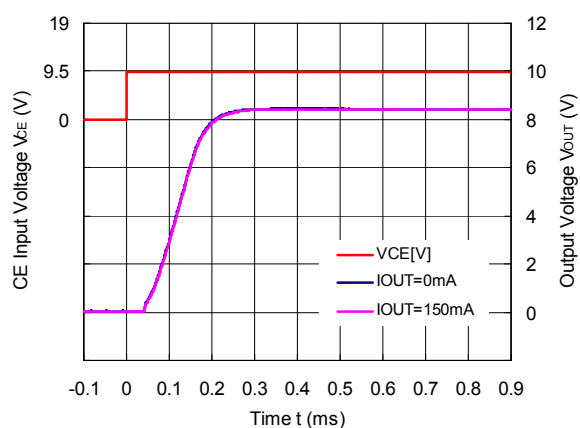
R1517x85xB/D (C2 = 0.1 \mu F)
