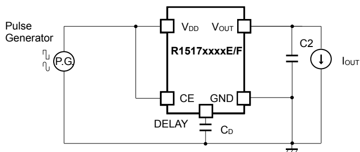
R1517xxxE/F Ripple Rejection Test Circuit
