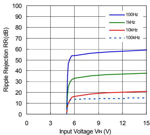
R1517x50xx ( I_{OUT} = 1\text{ mA} )
