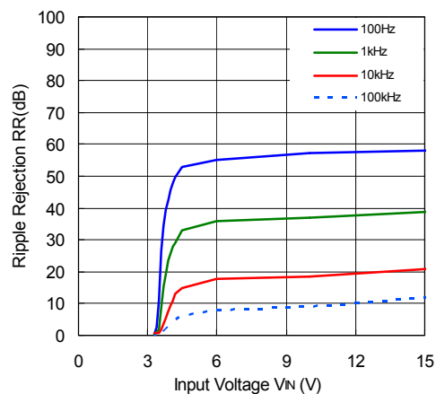
R1517x33xx ( I_{OUT} = 150\text{ mA} )
