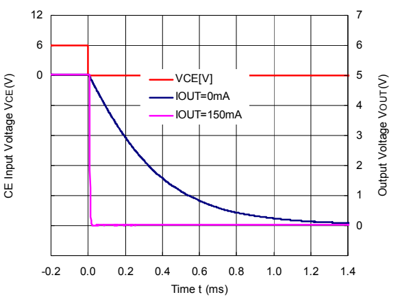
R1517x50xF (C2 = 0.1 μF, CD = 1 nF)
