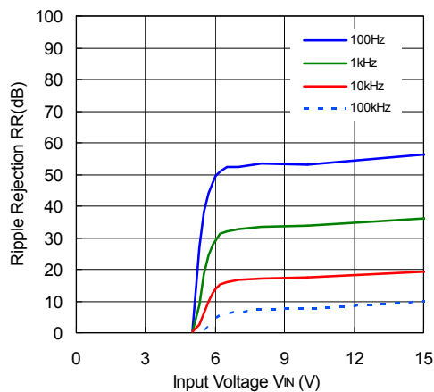
R1517x50xx ( I_{OUT} = 150\text{ mA} )
