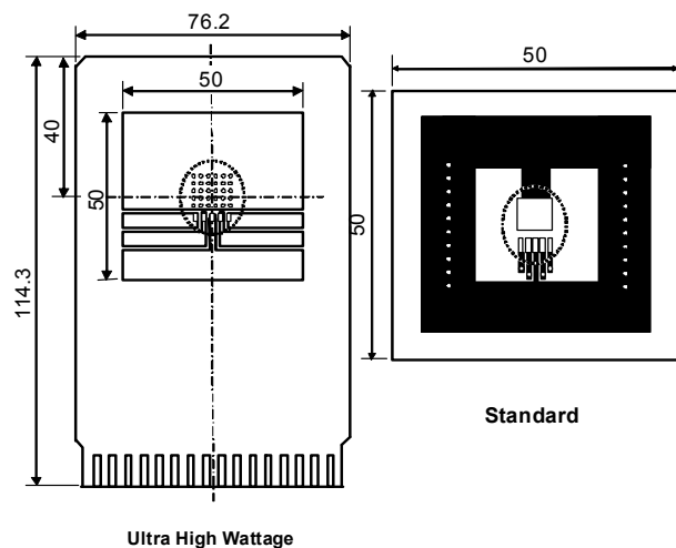
Measurement Board Pattern
