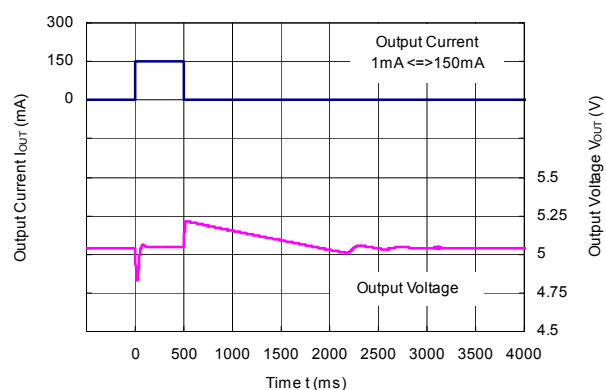
R1517x50xx ( C_2 = 10\text{ }\mu\text{F} )
