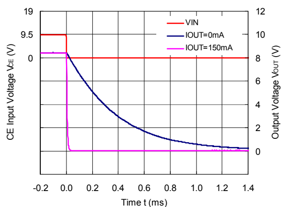
R1517x85xD (C2 = 0.1 \mu F)
