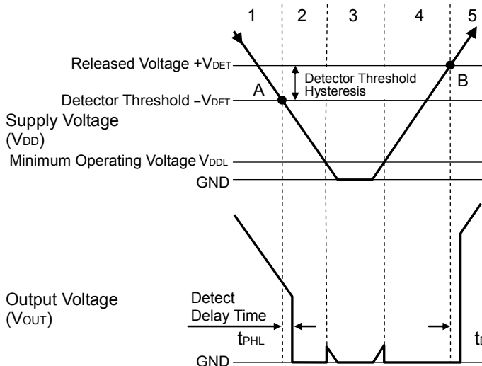
Fig. 2 Operation Diagram
