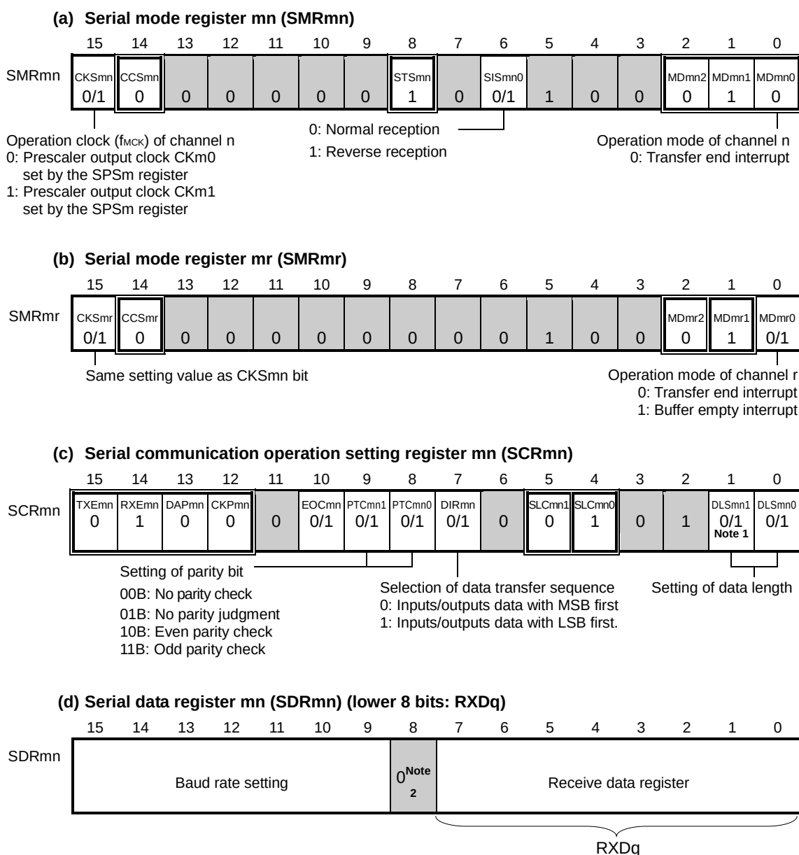
Figure 14-84. Example of Contents of Registers for UART Reception of UART (UART0 to UART2) (1/2)
