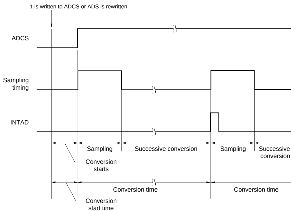
&lt;R&gt; Figure 12-5. A/D Converter Sampling and A/D Conversion Timing (Example for Software Trigger Mode)
