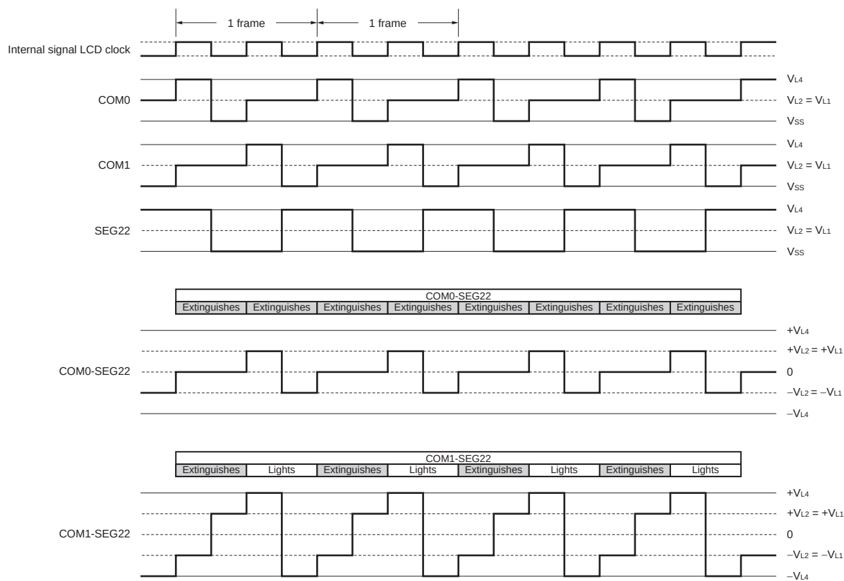
Figure 16-29. Two-Time-Slice LCD Drive Waveform Examples Between SEG22 and Each Common Signals (1/2 Bias Method)
