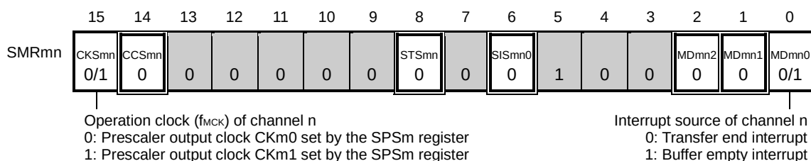
Figure 14-33. Example of Contents of Registers for Master Reception of 3-Wire Serial I/O (CSI00) (1/2)
