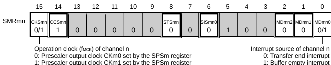
Figure 14-49. Example of Contents of Registers for Slave Transmission of 3-Wire Serial I/O (CSI00) (1/2)
