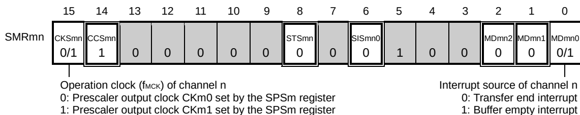
Figure 14-63. Example of Contents of Registers for Slave Transmission/Reception of 3-Wire Serial I/O (CSI00) (1/2)
