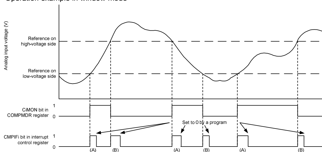
Figure 13-7. Example of Comparator i (i = 0 or 1) Operation in Window Mode
