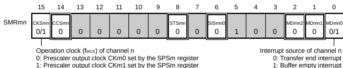
Figure 14-25. Example of Contents of Registers for Master Transmission of 3-Wire Serial I/O (CSI00) (1/2)
