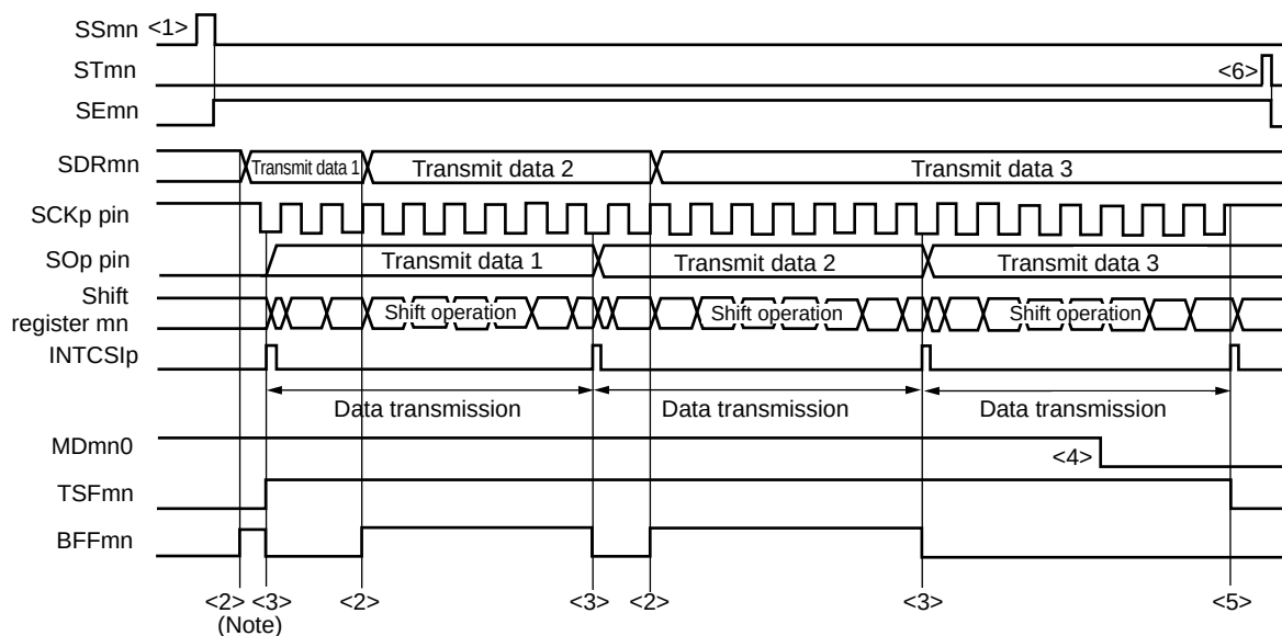
Figure 14-55. Timing Chart of Slave Transmission (in Continuous Transmission Mode)
