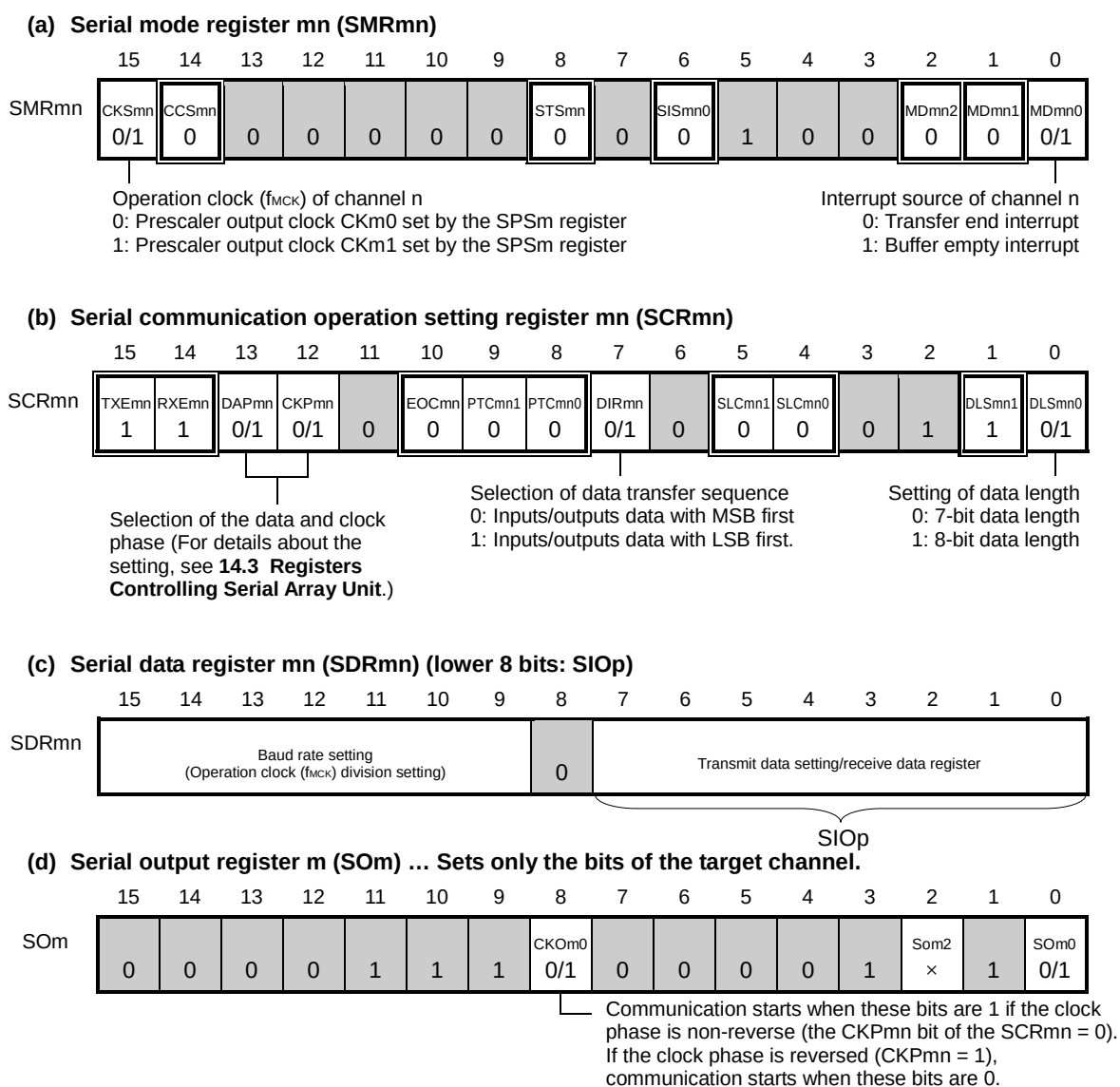
Figure 14-41. Example of Contents of Registers for Master Transmission/Reception of 3-Wire Serial I/O (CSI00) (1/2)
