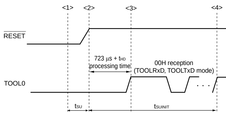
Figure 27-7. Setting of Flash Memory Programming Mode
