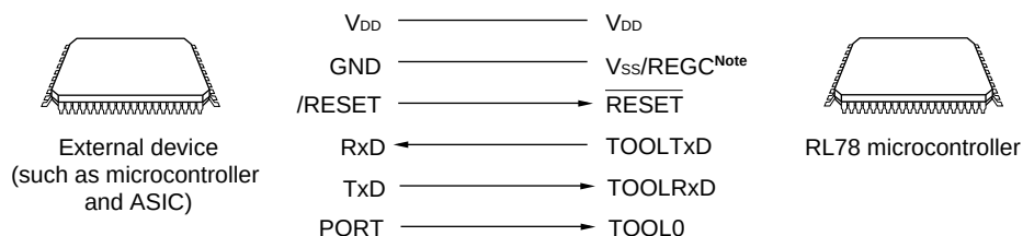
Figure 27-4. Communication with External Device
