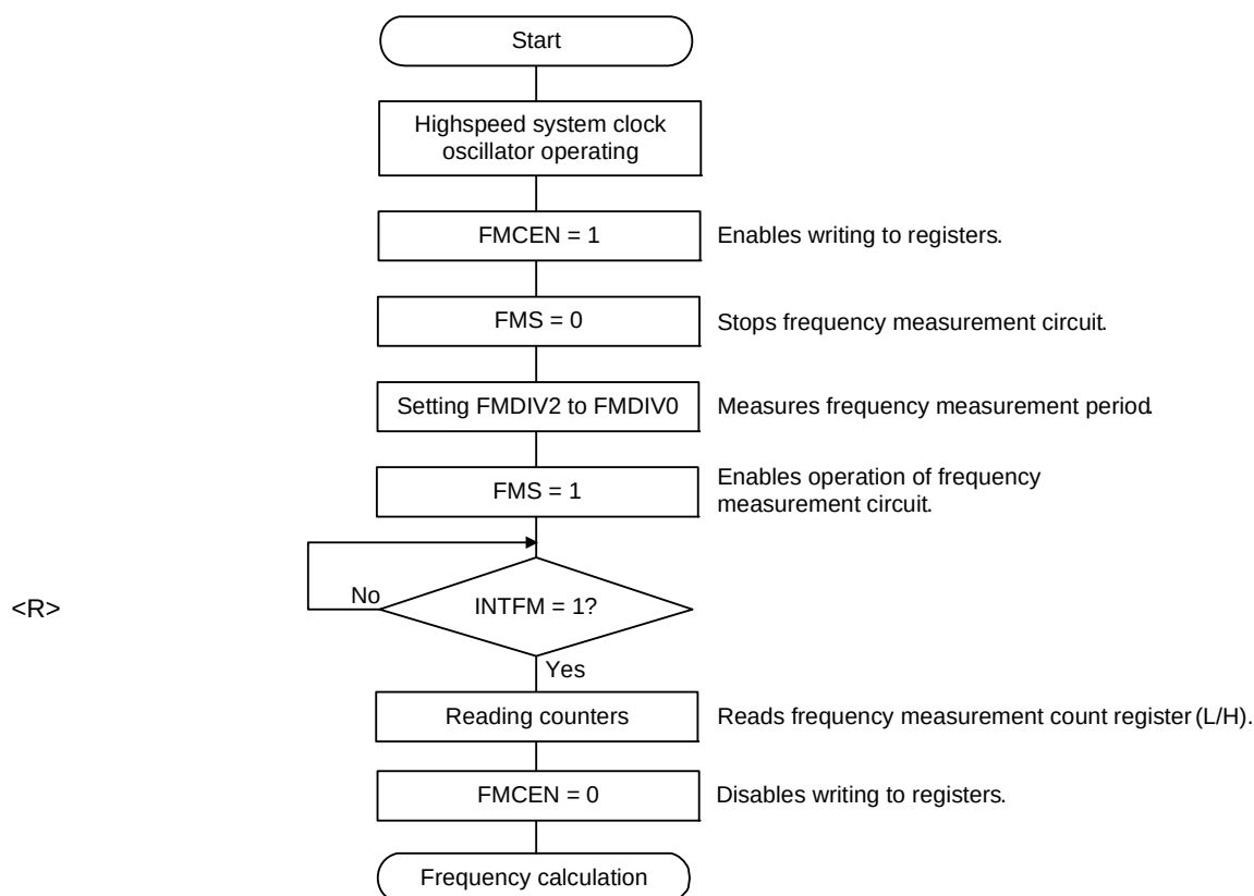
Figure 8-8. Procedure for Setting Subsystem Clock Frequency Measurement Circuit
