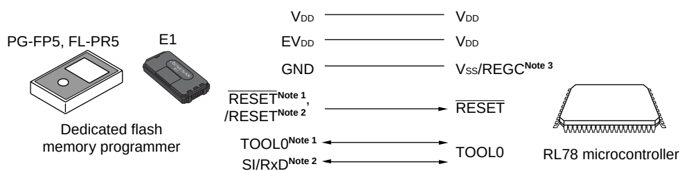
Figure 27-2. Communication with Dedicated Flash Memory Programmer
