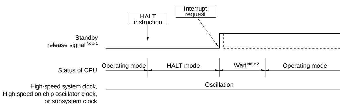
Figure 20-1. HALT Mode Release by Interrupt Request Generation
