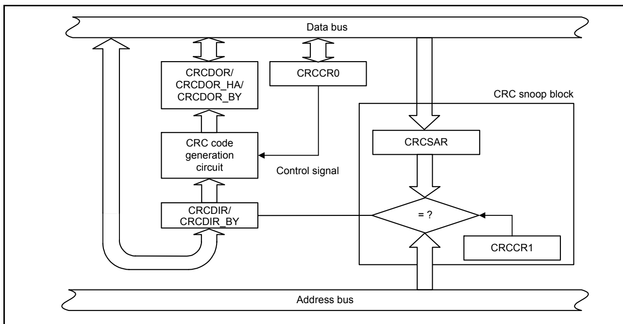
Figure 32.1 CRC block diagram
