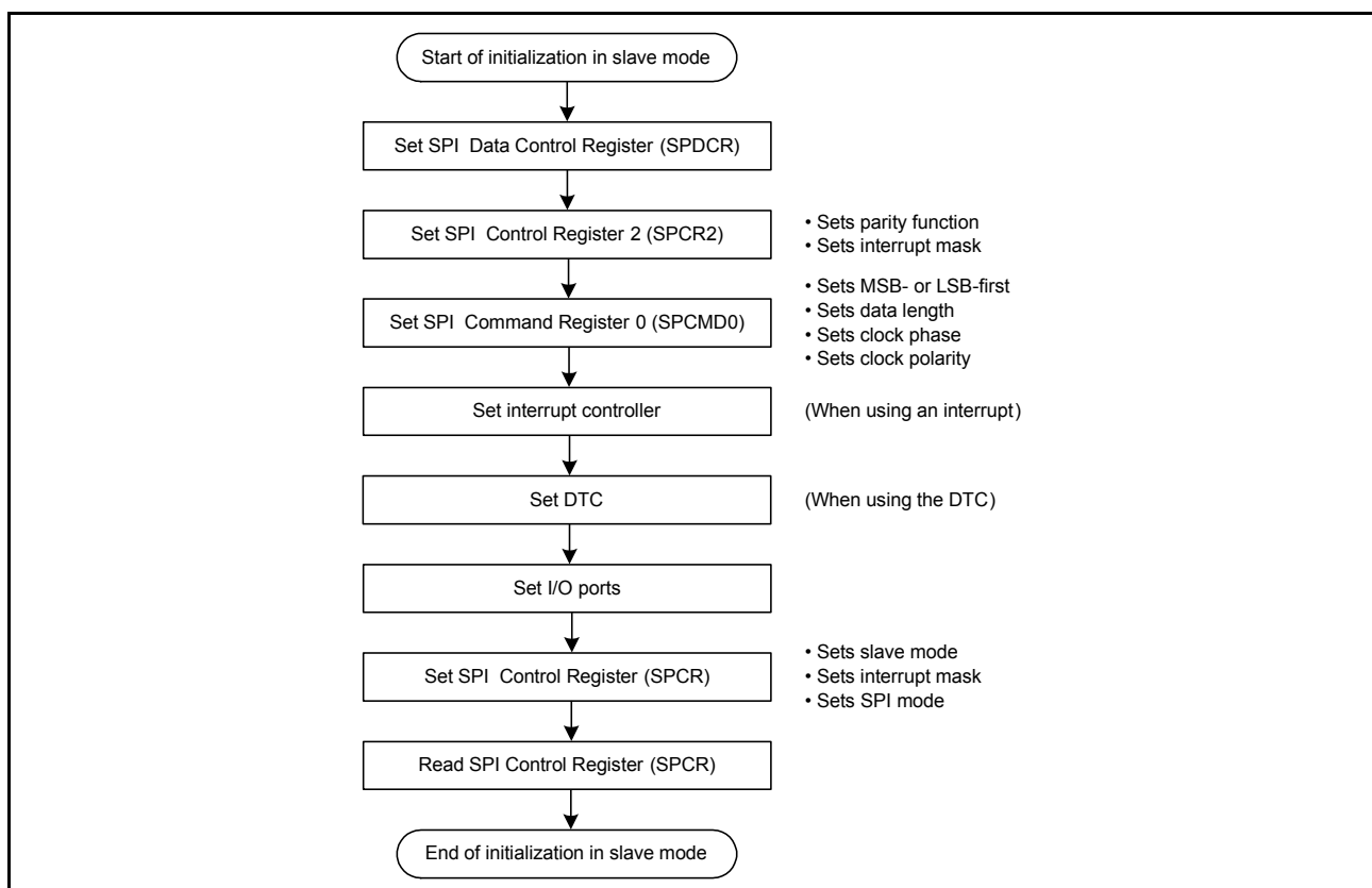
Figure 31.41 Example of initialization flow in slave mode for clock synchronous operation
