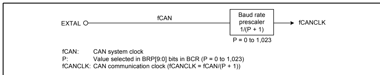
Figure 30.11 Block diagram of CAN clock generator
