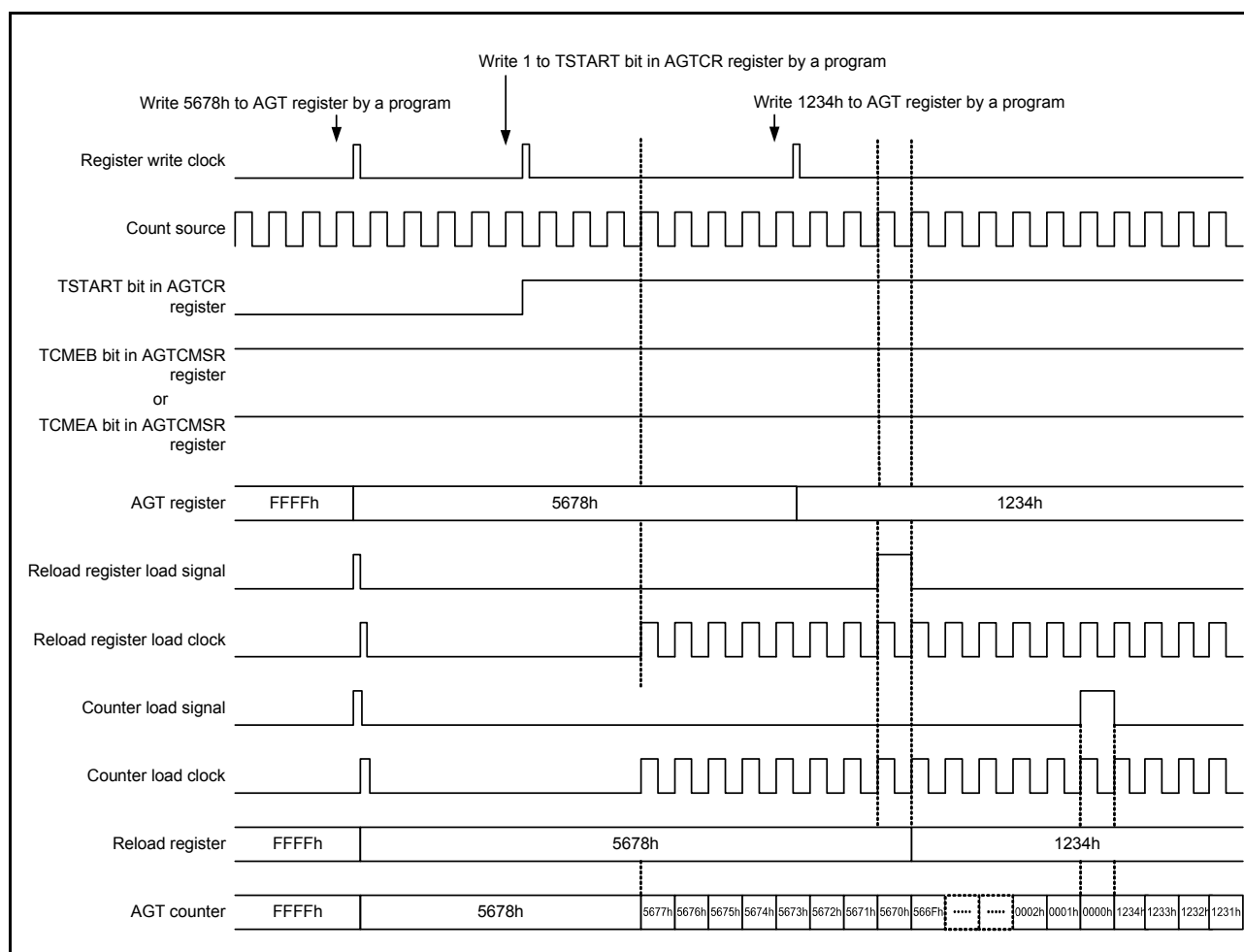
Figure 22.3 Timing of rewrite operation with TSTART and TCMEA or TCMEB bit values when compare match A register or B is valid
