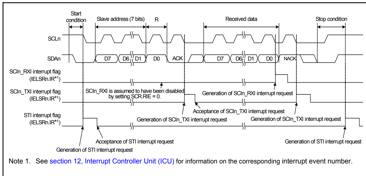
Figure 27.66 Example operations for master reception in simple IIC bus mode with 7-bit slave addresses, transmission interrupts, and reception interrupts
