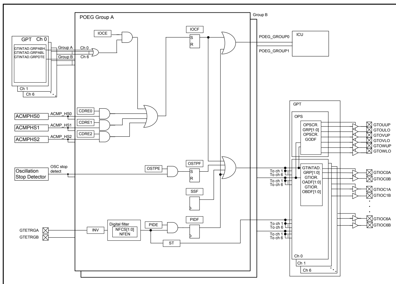
Figure 19.1 POEG block diagram
