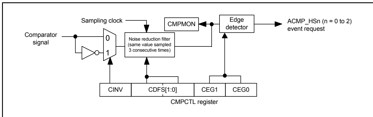
Figure 37.3 Noise filter and edge detection configuration
