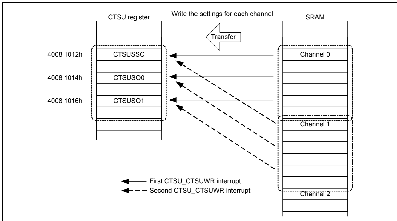
Figure 39.19 Example DTC transfer operation using the CTSUS_CTSUWR interrupt
