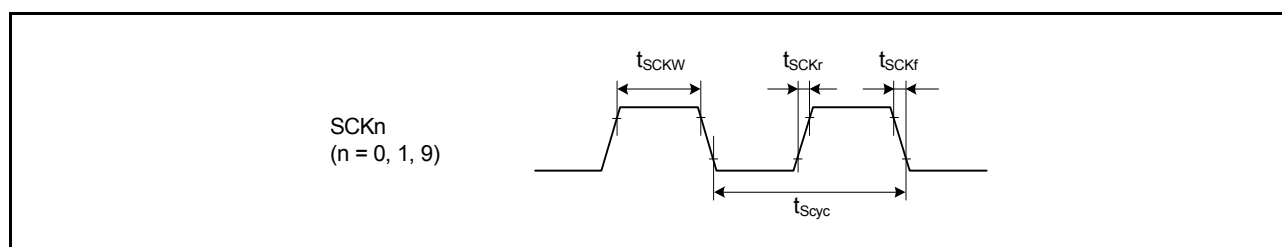
Figure 46.34 SCK clock input timing
