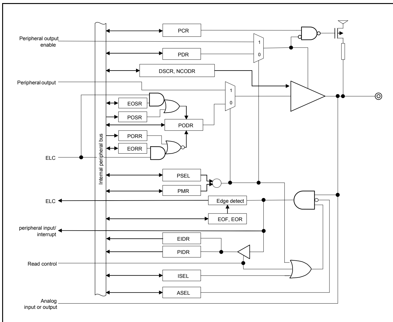
Figure 17.1 I/O Ports registers connection diagram
