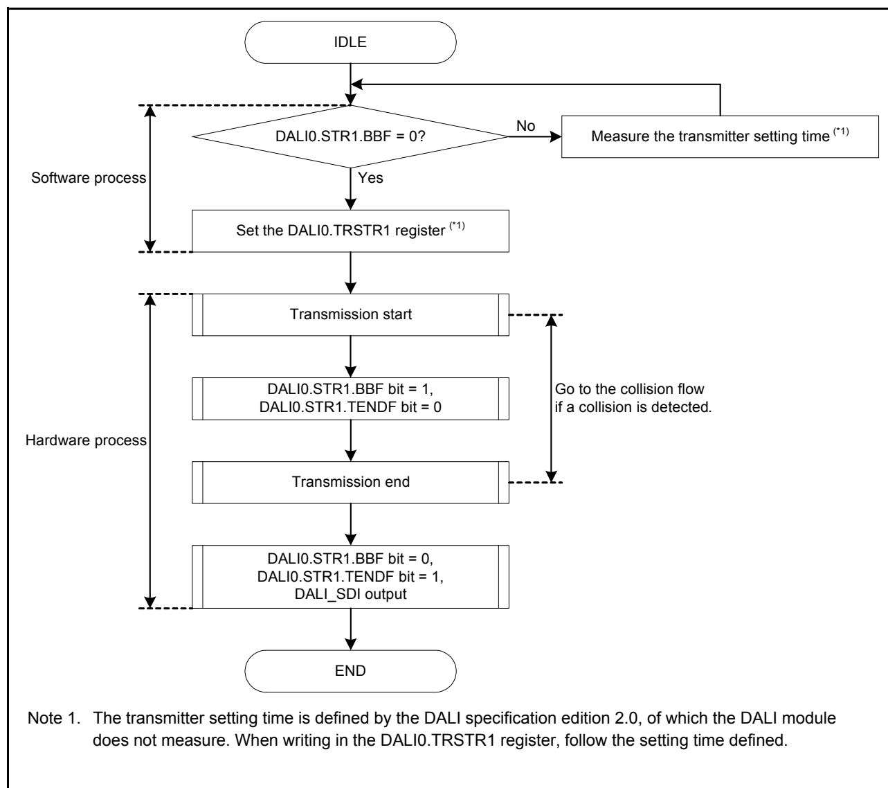
Figure 28.22 Transmission flow
