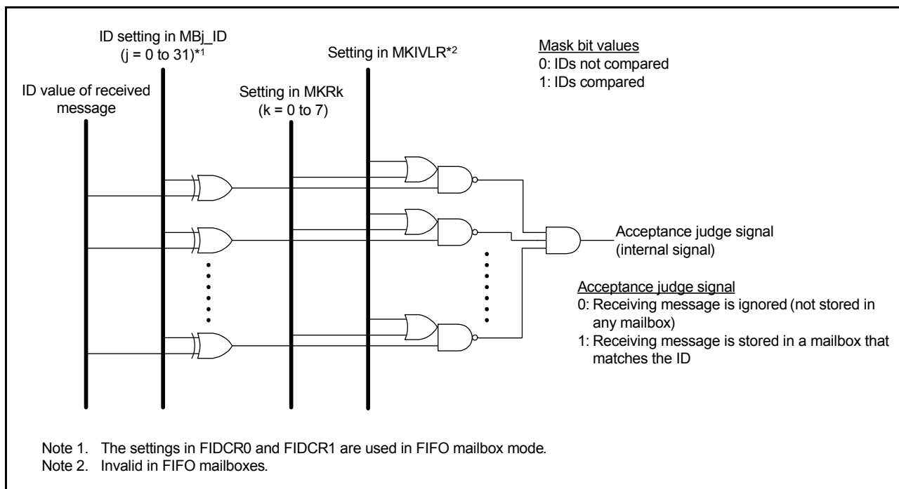
Figure 30.17 Acceptance filtering
