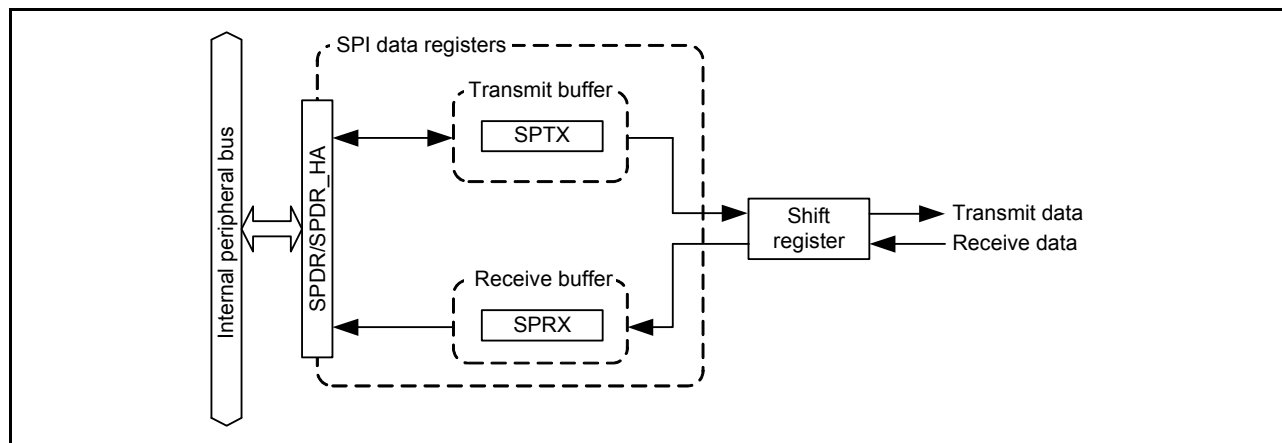
Figure 31.2 Configuration of SPDR/SPDR_HA
