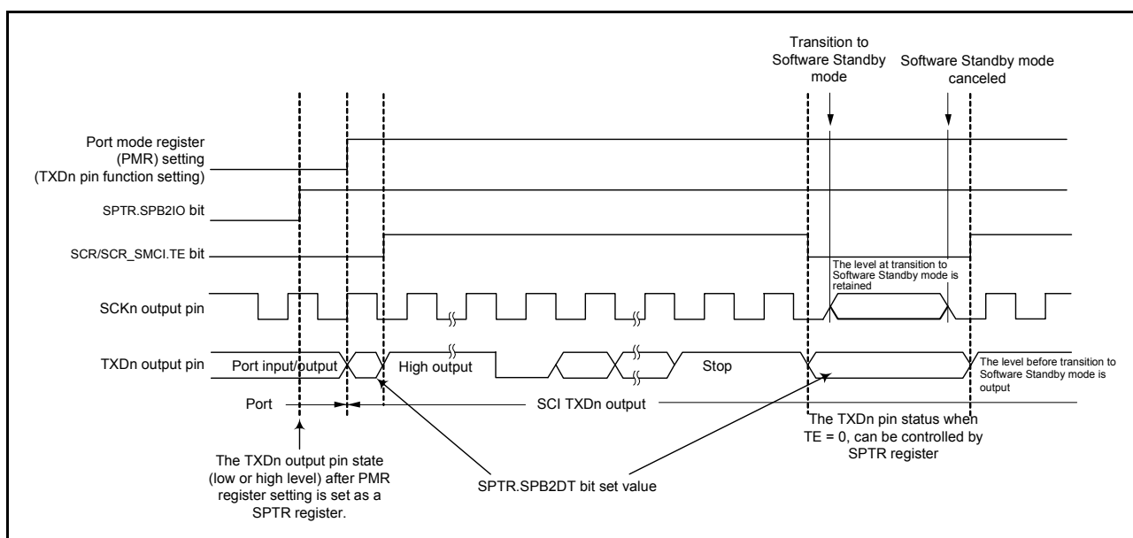
Figure 27.73 Port pin states during transition to Software Standby mode with internal clock and asynchronous transmission
