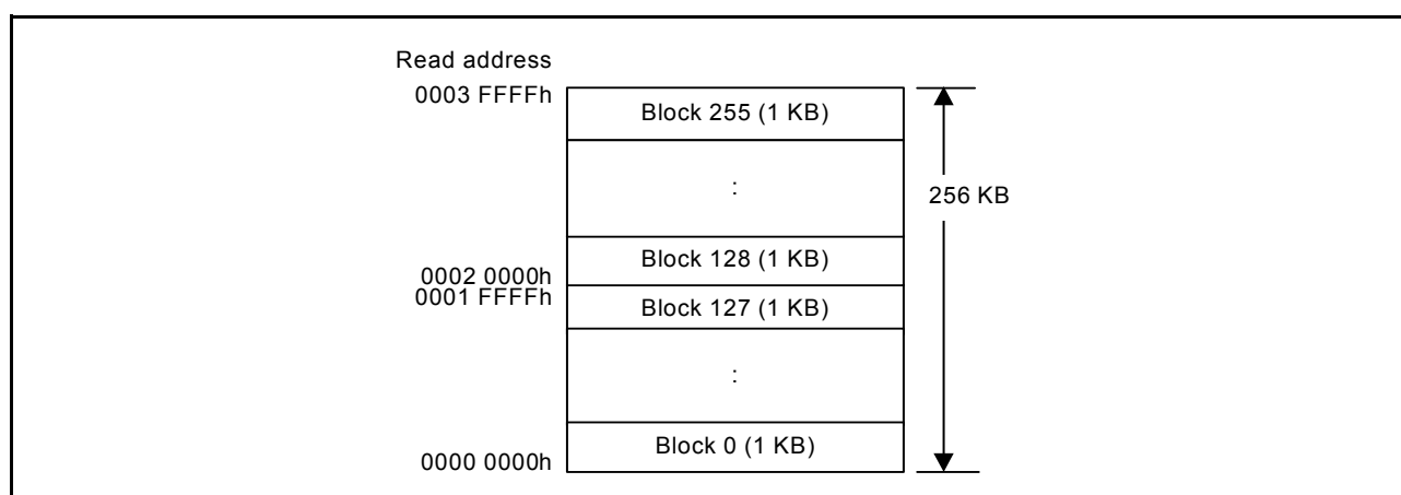
Figure 42.2 Mapping of the code flash memory
