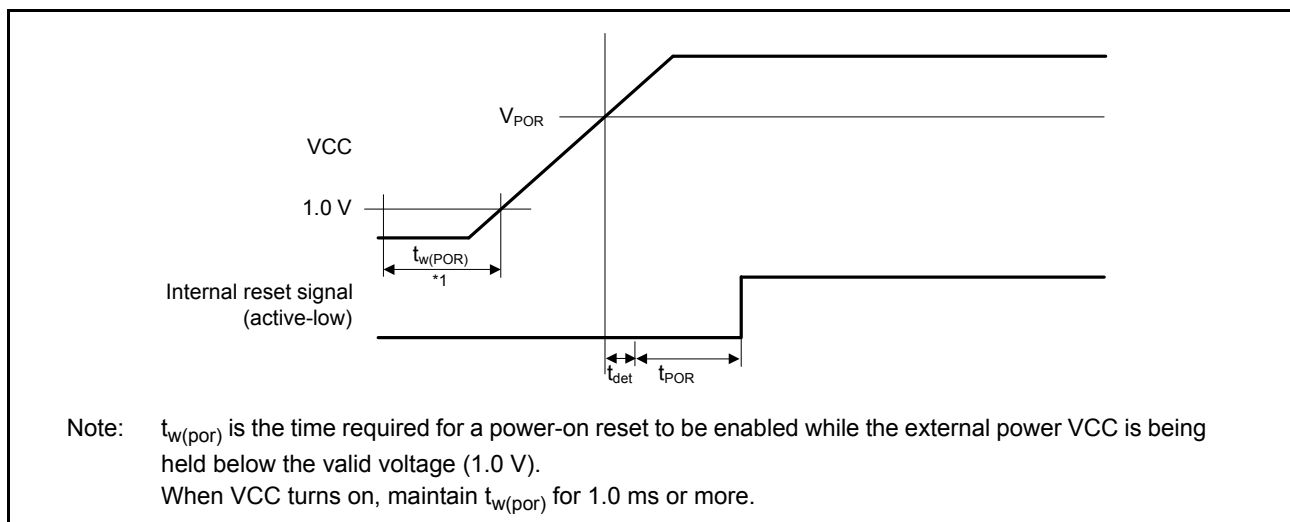
Figure 46.58 Power-on reset timing
