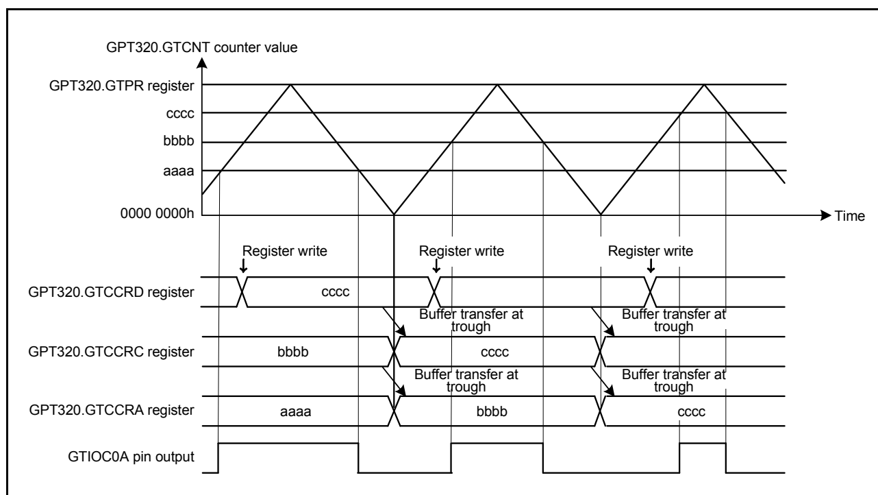
Figure 20.23 Example of GTCCRA and GTCCRB double buffer operation with output compare, triangle waves, buffer operation at trough, output toggled at GTCCRA compare match, and output retained at cycle end
