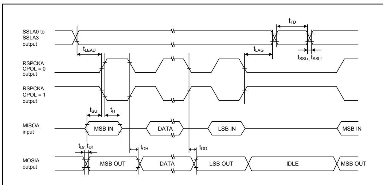
Figure 46.43 SPI timing (master, CPHA = 0) (bit rate: PCLKB division ratio is set to any value other than 1/2)
