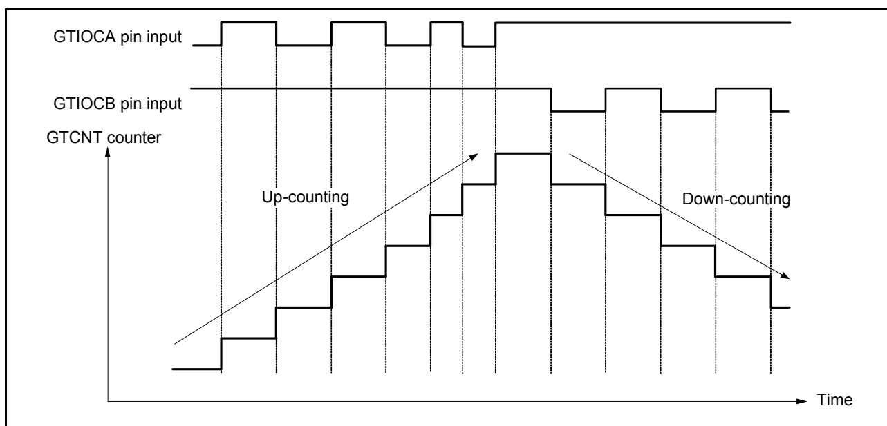
Figure 20.73 Example of phase counting mode 3 (C)
