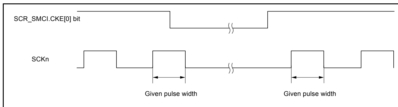
Figure 27.56 Clock output fixed timing
