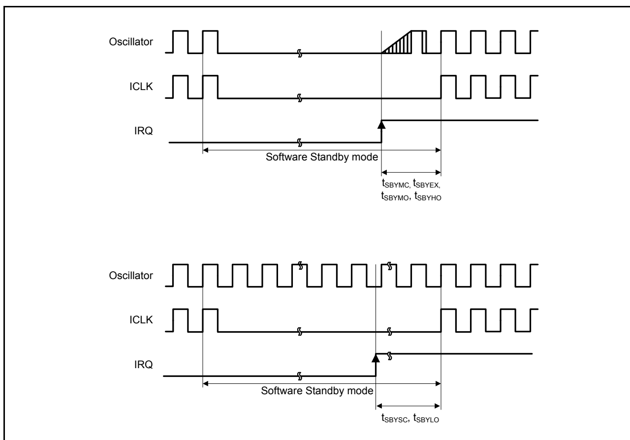
Figure 46.25 Software Standby mode cancellation timing
