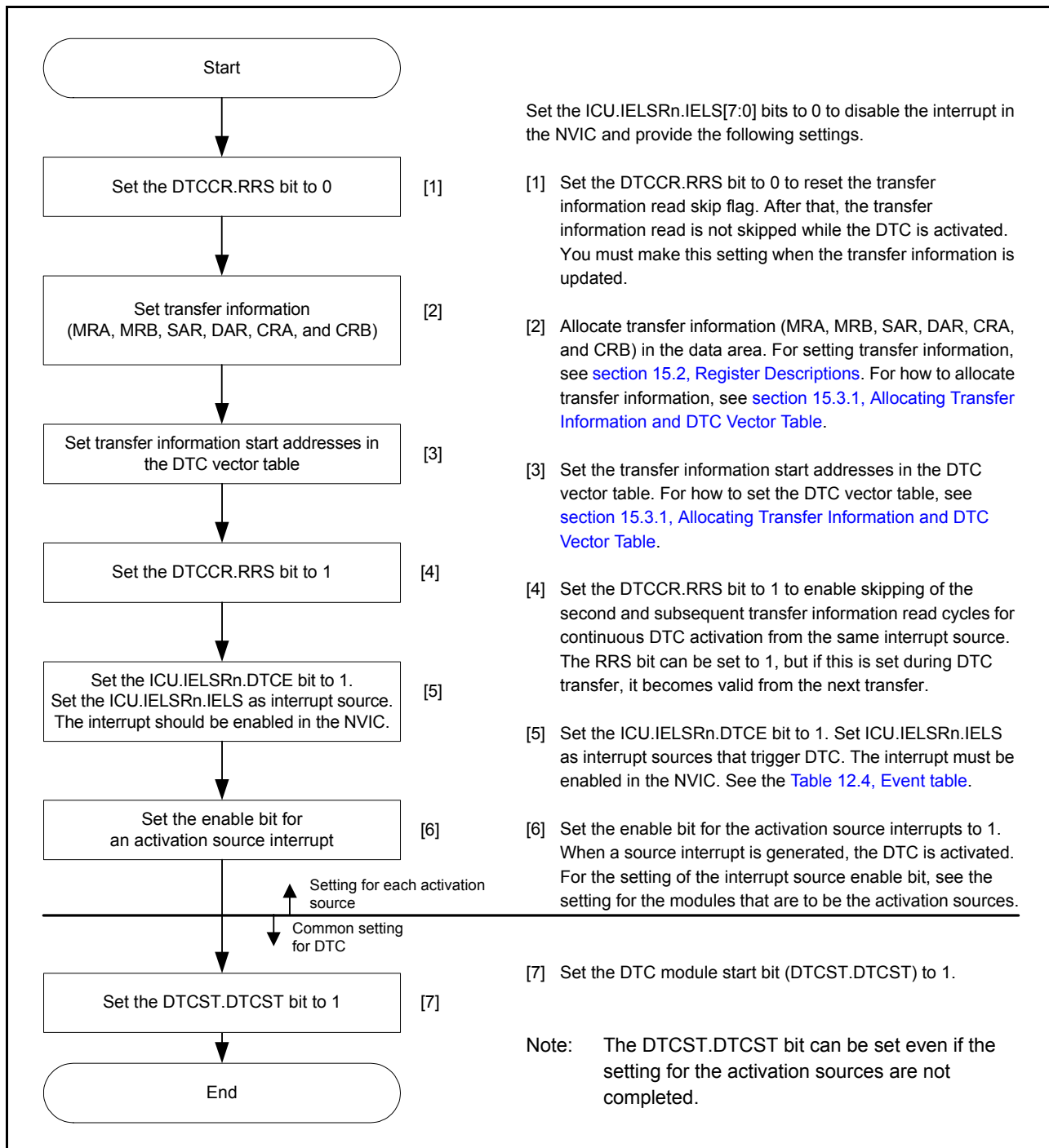
Figure 15.13 DTC setting procedure
