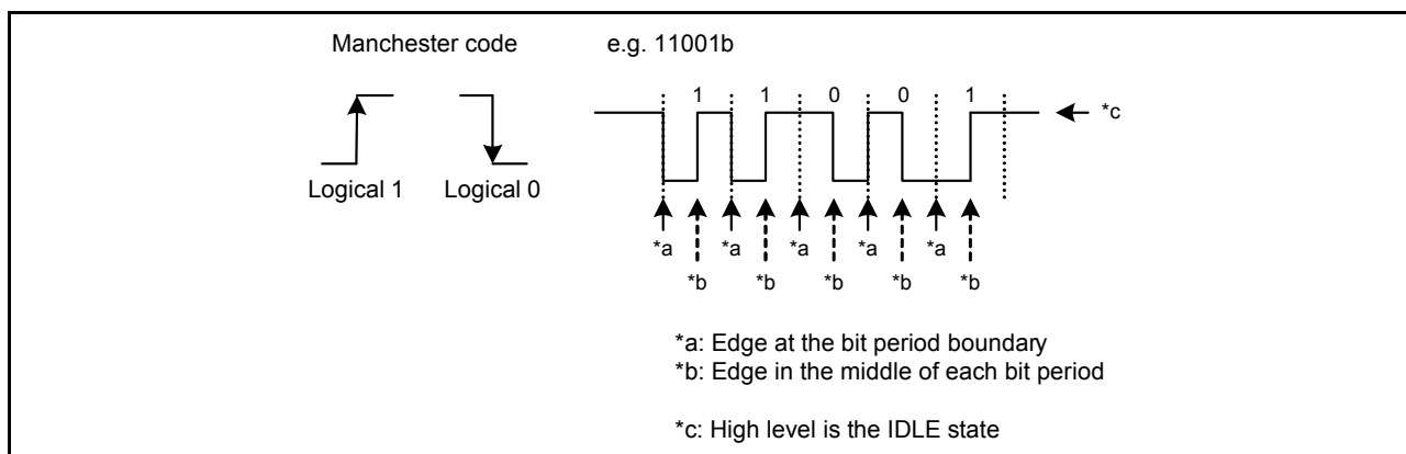
Figure 28.4 Manchester code
