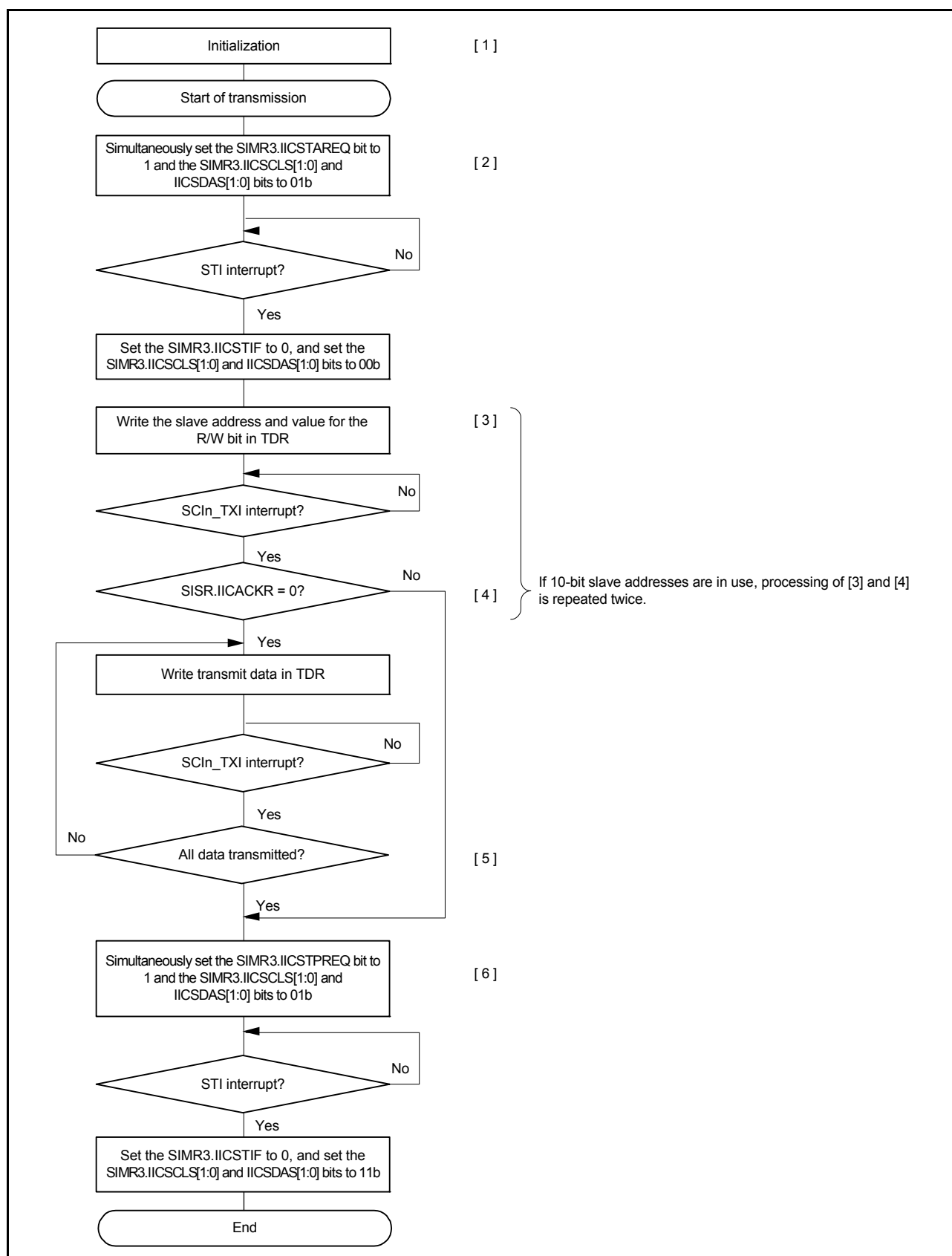
Figure 27.65 Example procedure for master transmission operations in simple IIC mode with transmission interrupts and reception interrupts
