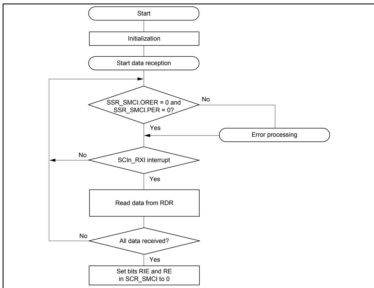
Figure 27.55 Example flow for smart card interface reception
