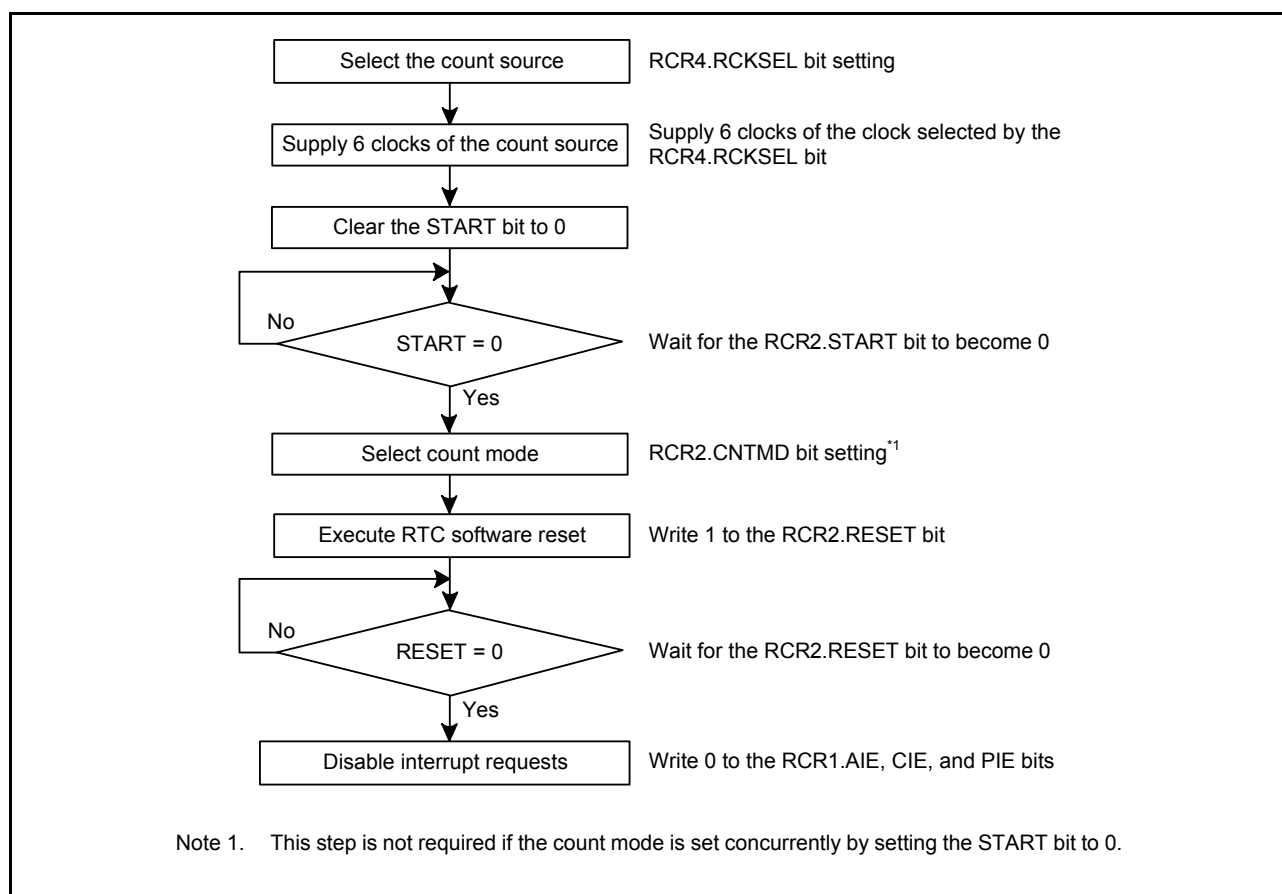
Figure 23.12 Initialization procedure
