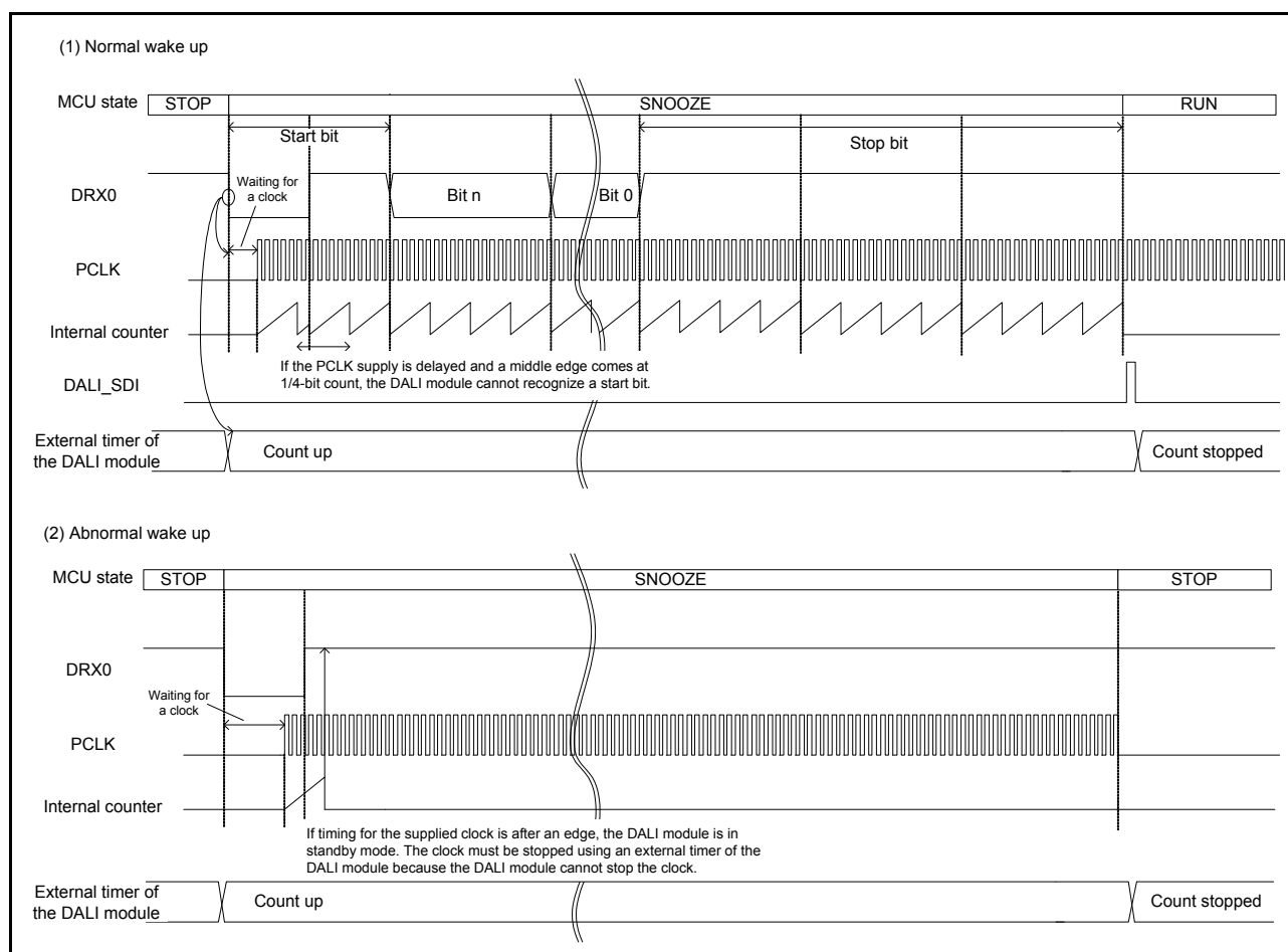
Figure 28.32 Startup from Snooze mode
