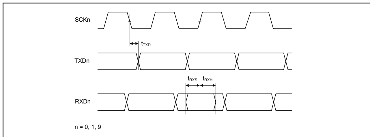
Figure 46.35 SCI input/output timing in clock synchronous mode
