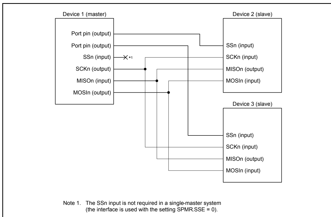
Figure 27.68 Example of connections using simple SPI mode in single master mode with SPMR.SSE bit = 0
