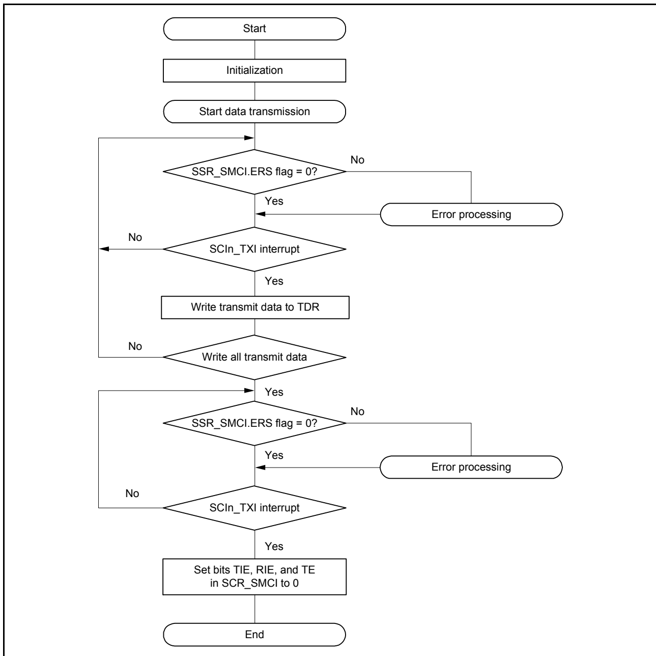
Figure 27.53 Example flow for smart card interface transmission
