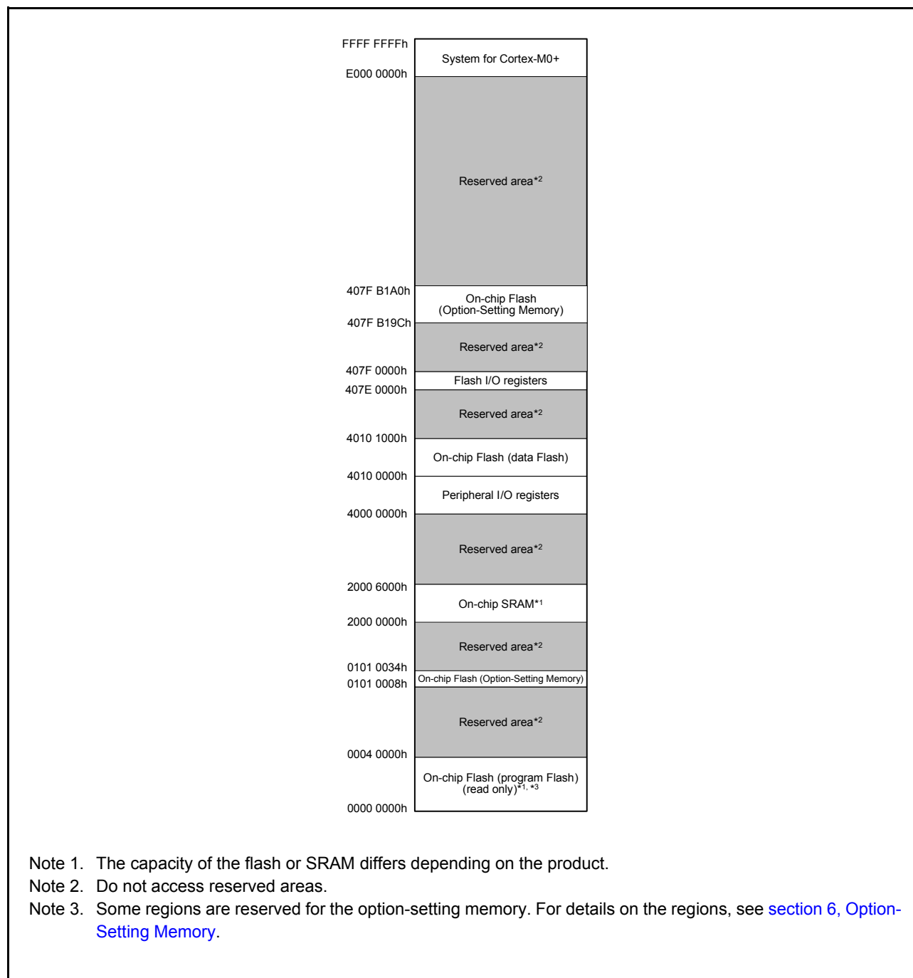
Figure 4.1 Memory map
