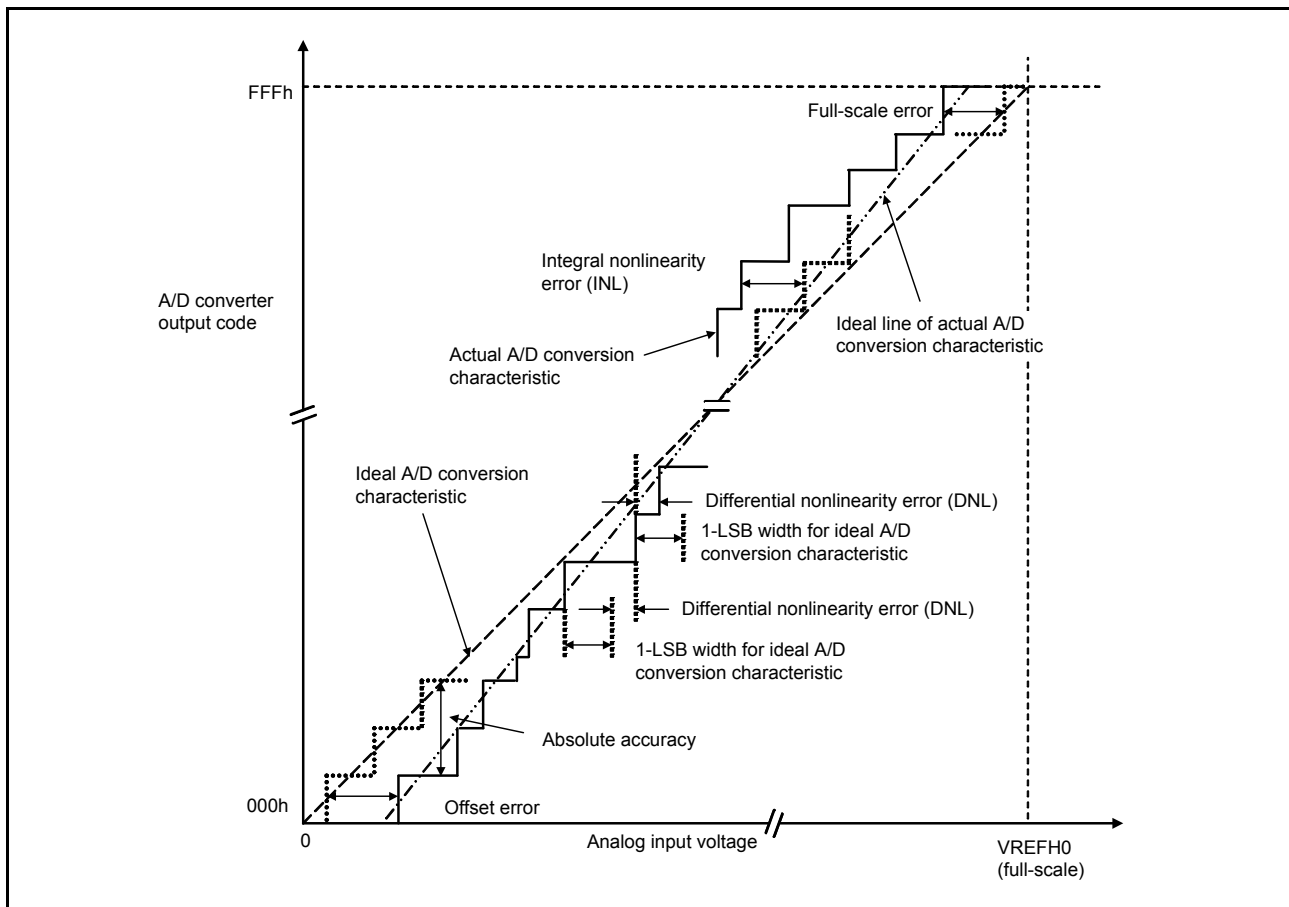
Figure 46.55 Illustration of 14-bit A/D converter characteristic terms
