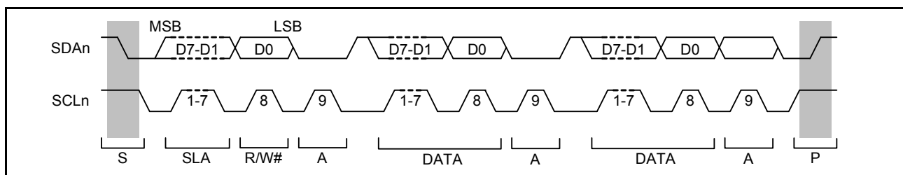
Figure 27.58 I 2 C bus timing when SLA is 7 bits
