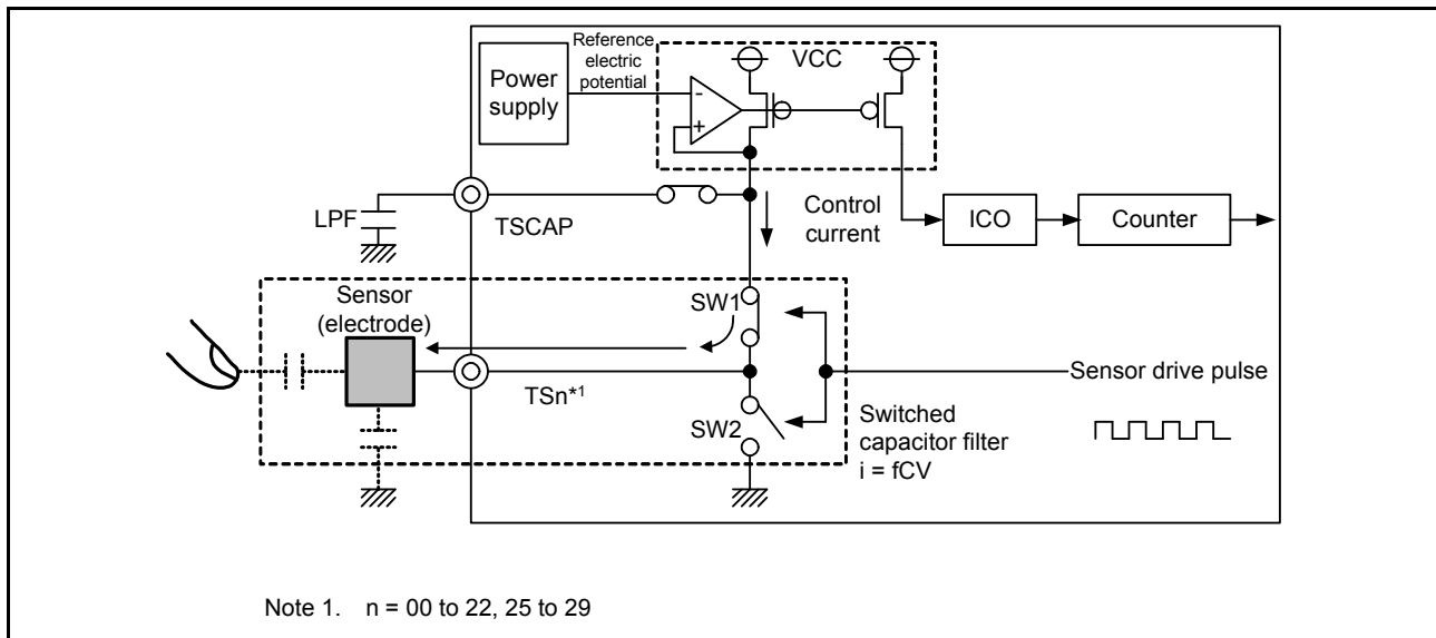
Figure 39.5 Charging operation
