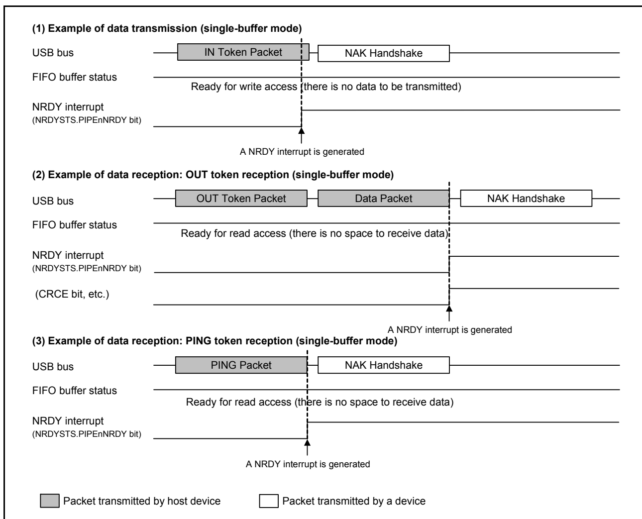
Figure 26.10 Timing of NRDY interrupt generation
