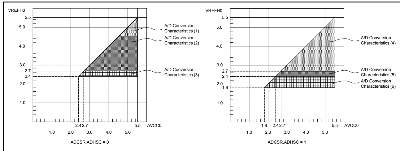
Figure 46.54 AVCC0 to VREFH0 voltage range
