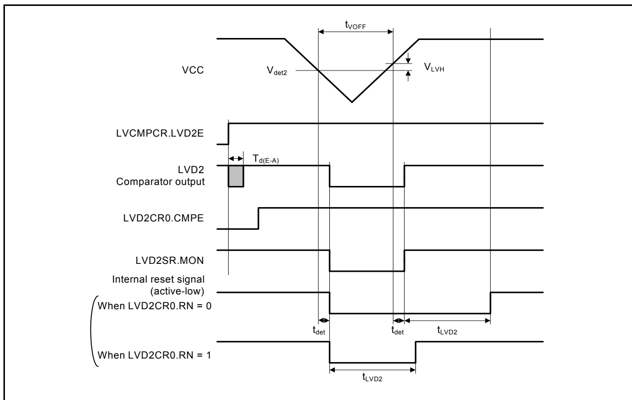
Figure 46.61 Voltage detection circuit timing ( V_{det2} )
