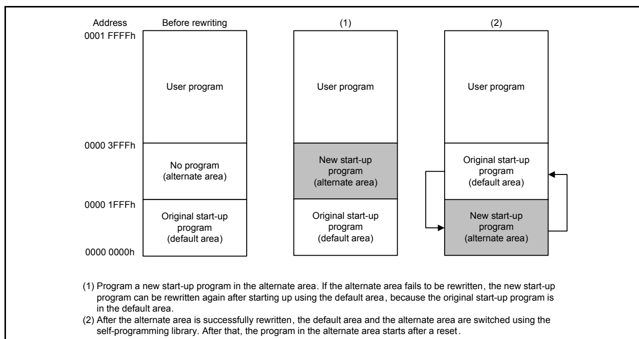
Figure 42.6 Overview of startup program protection
