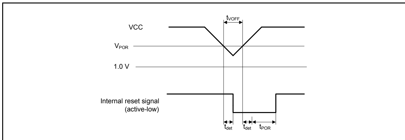
Figure 46.57 Voltage detection reset timing
