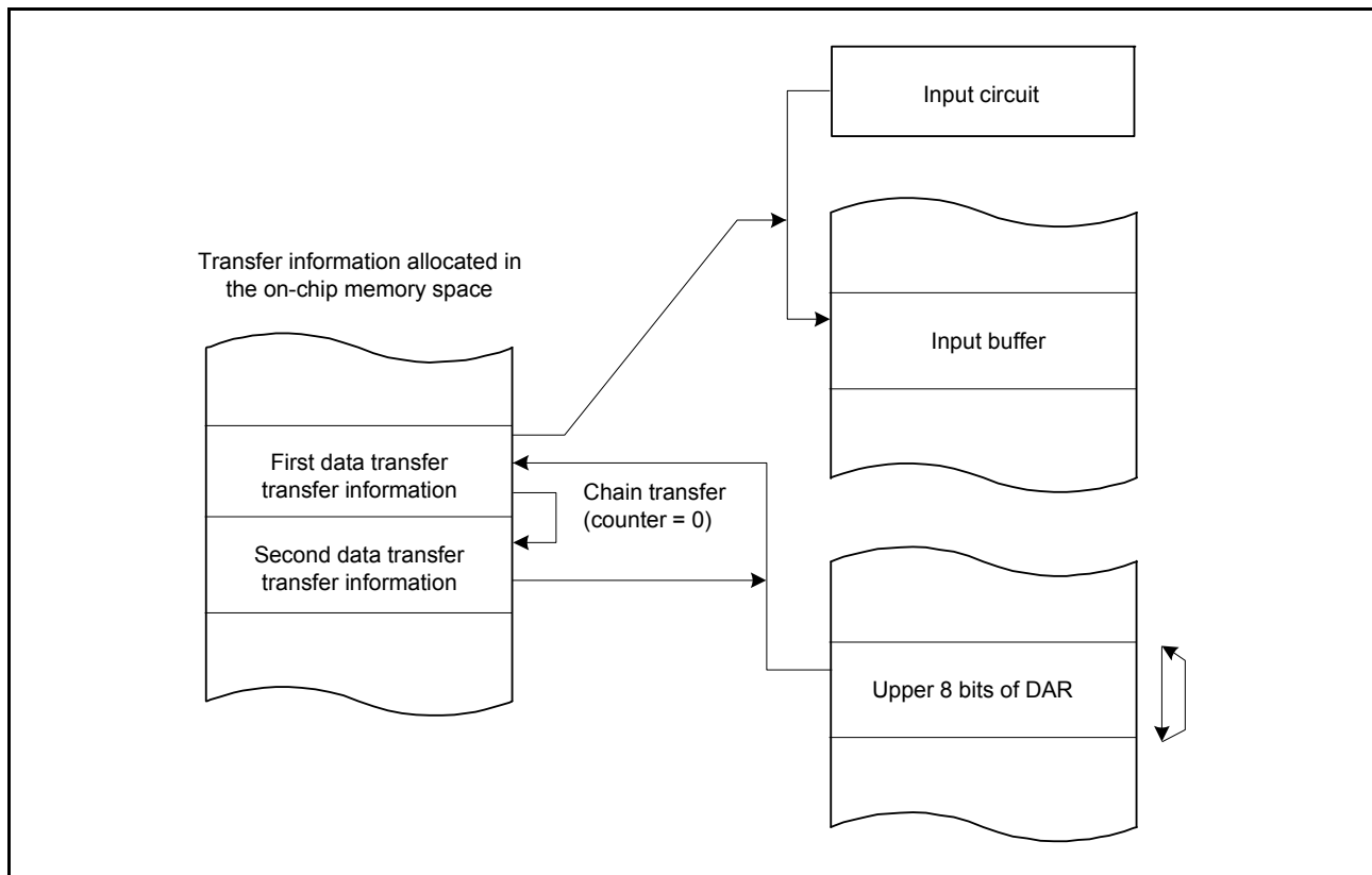
Figure 15.14 Chain transfer when counter = 0
