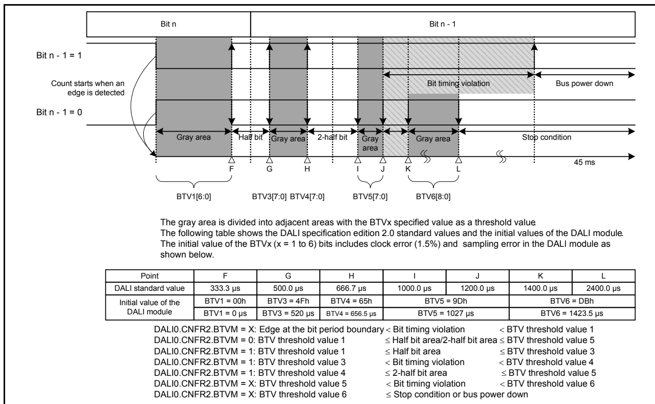
Figure 28.11 Bit timing violation 2
