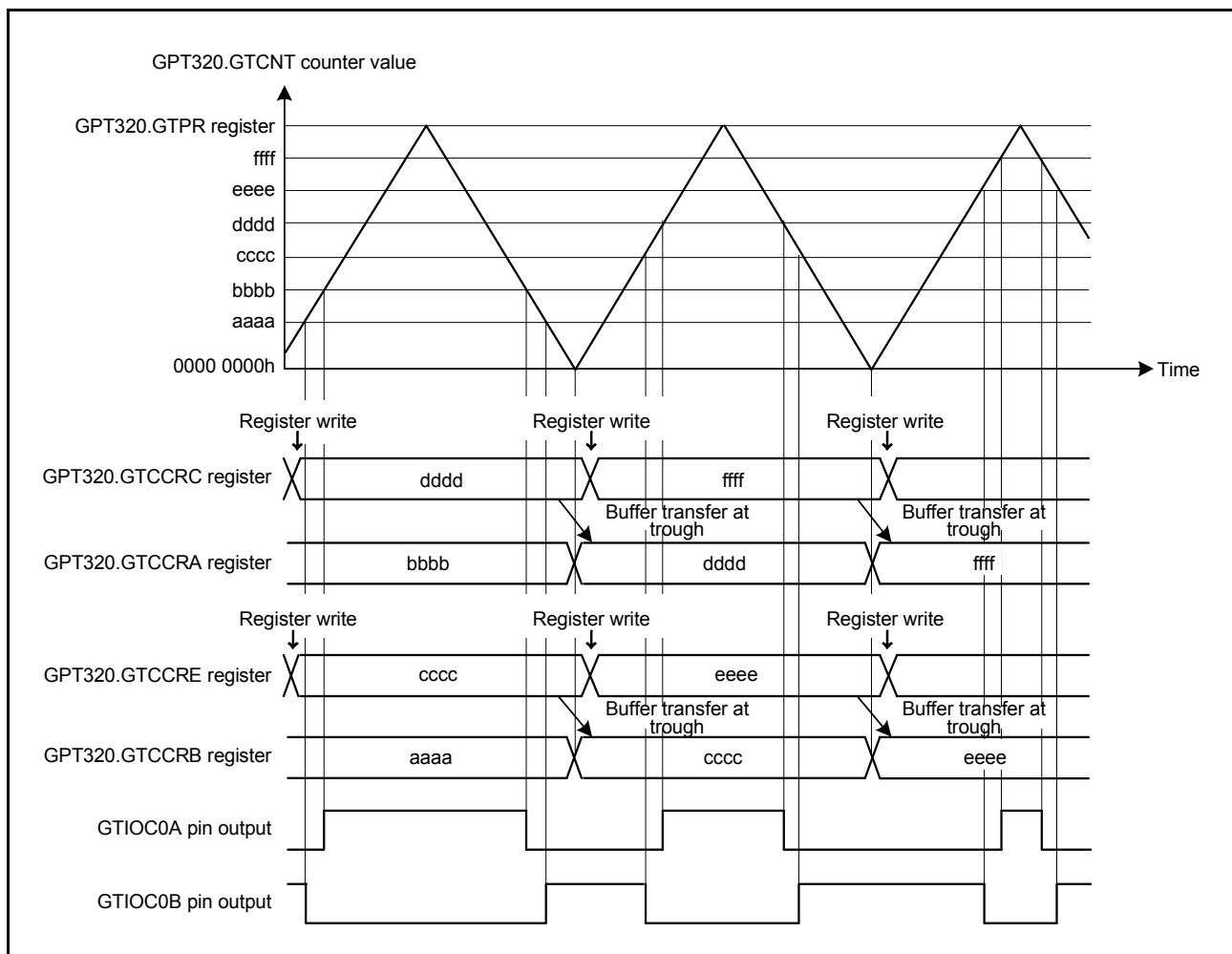
Figure 20.33 Example of triangle-wave PWM mode 1 operation with buffer operation, low output from the GTIOCA pin and high output from the GTIOCB pin at count start, output toggled at GTCCRA/ GTCCRB register compare match, and output retained at cycle end
