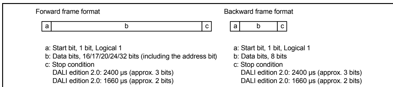
Figure 28.5 DALI data format
