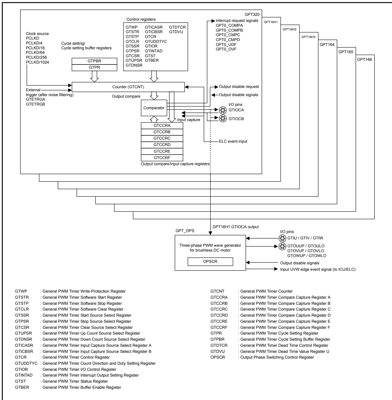
Figure 20.1 GPT block diagram
