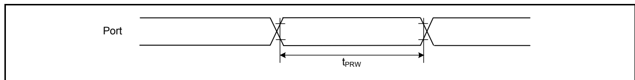
Figure 46.28 I/O ports input timing
