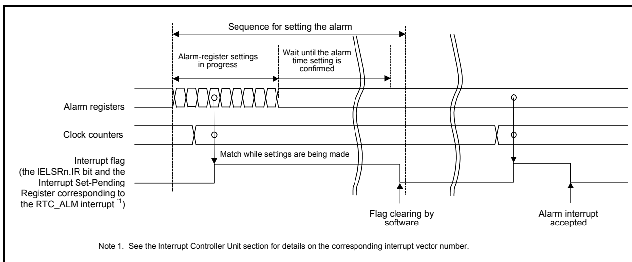
Figure 23.9 Timing for the alarm interrupt (RTC_ALM)
