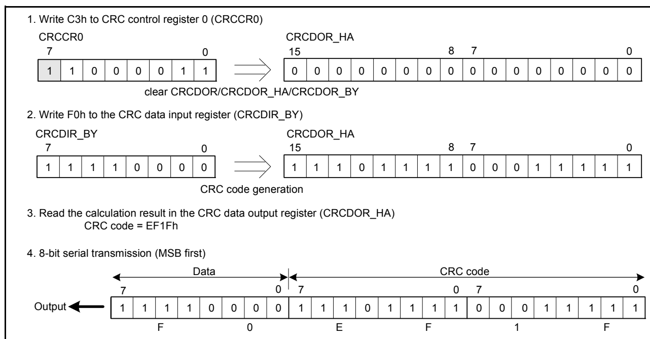
Figure 32.3 MSB-first data transmission
