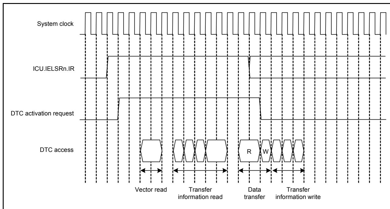
Figure 15.9 Example (1) of DTC operation timing in normal transfer and repeat transfer modes
