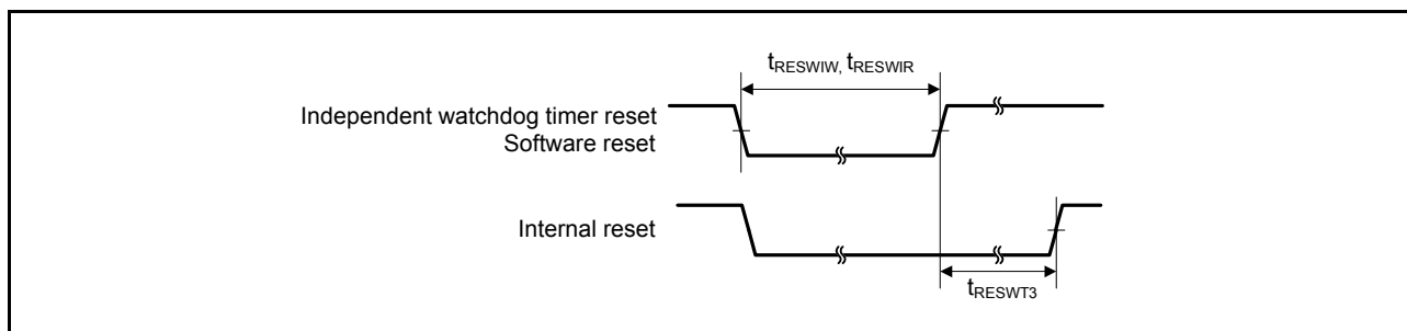
Figure 46.24 Reset input timing (2)
