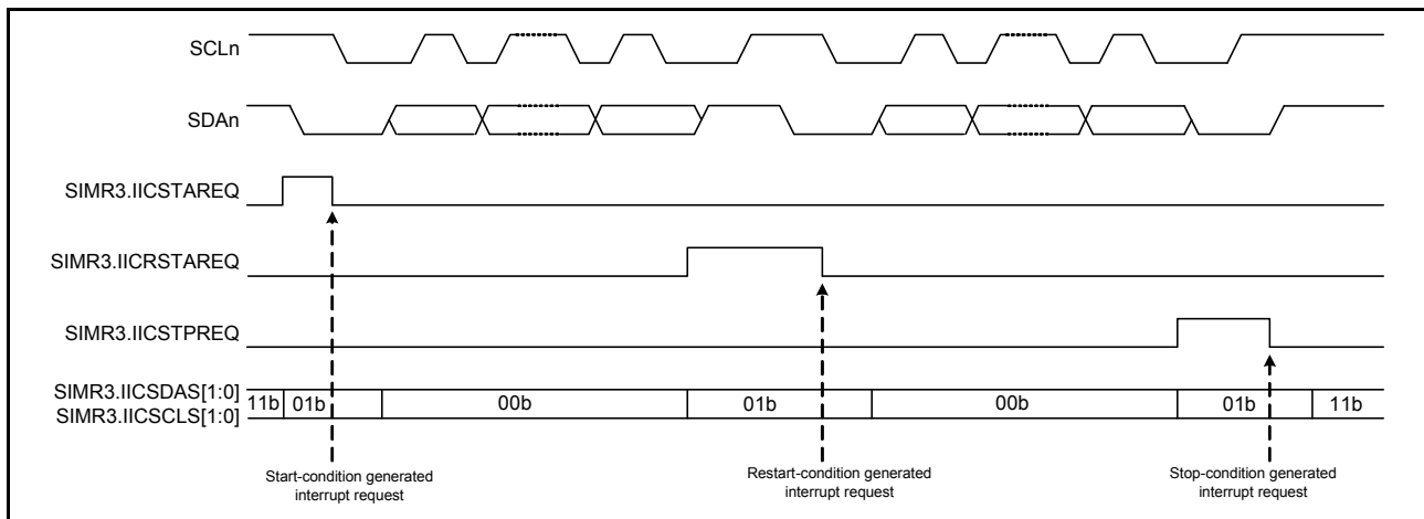
Figure 27.59 Timing operations in generation of start, restart, and stop conditions
