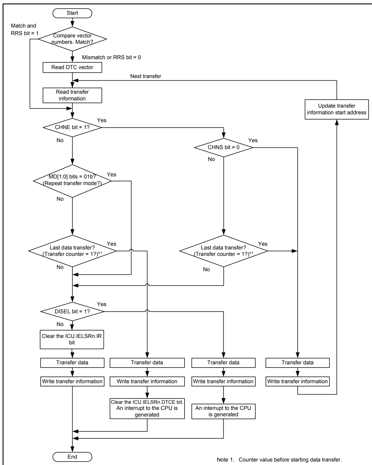
Figure 15.4 DTC operation flow
