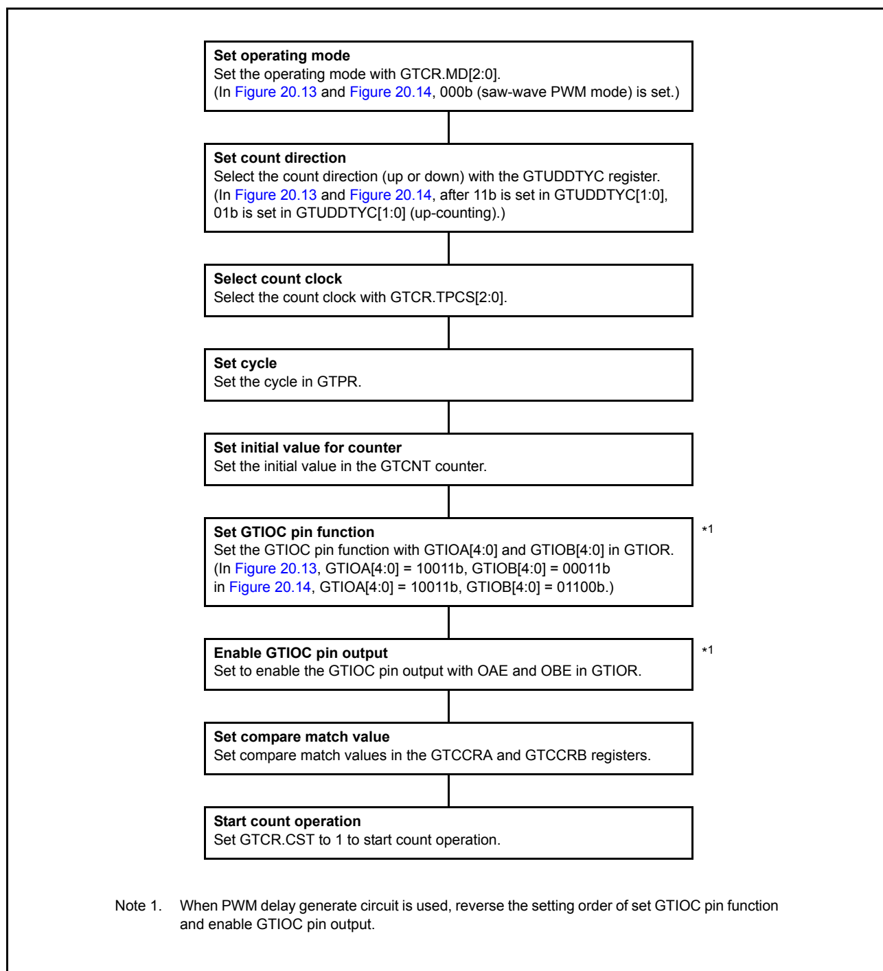
Figure 20.15 Example for setting toggled output operation
