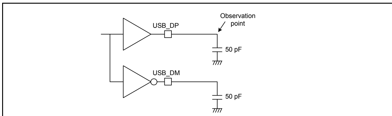
Figure 46.52 Test circuit for Full-Speed (FS) connection
