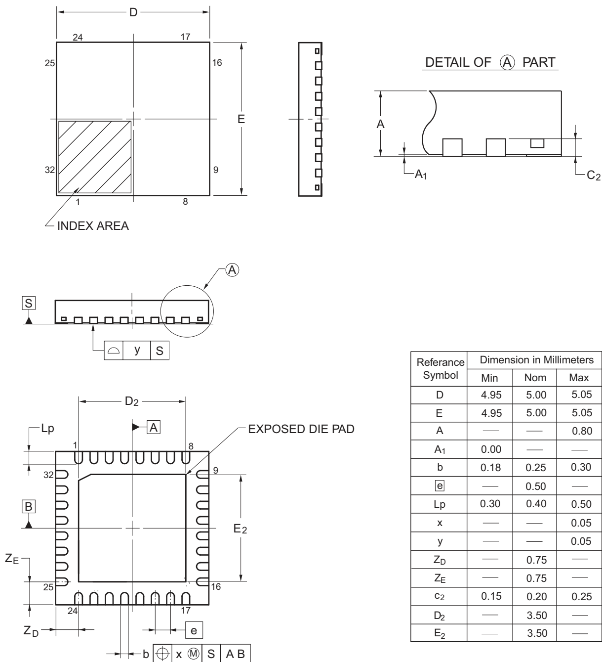
Figure 2.6 QFN 32-pin
