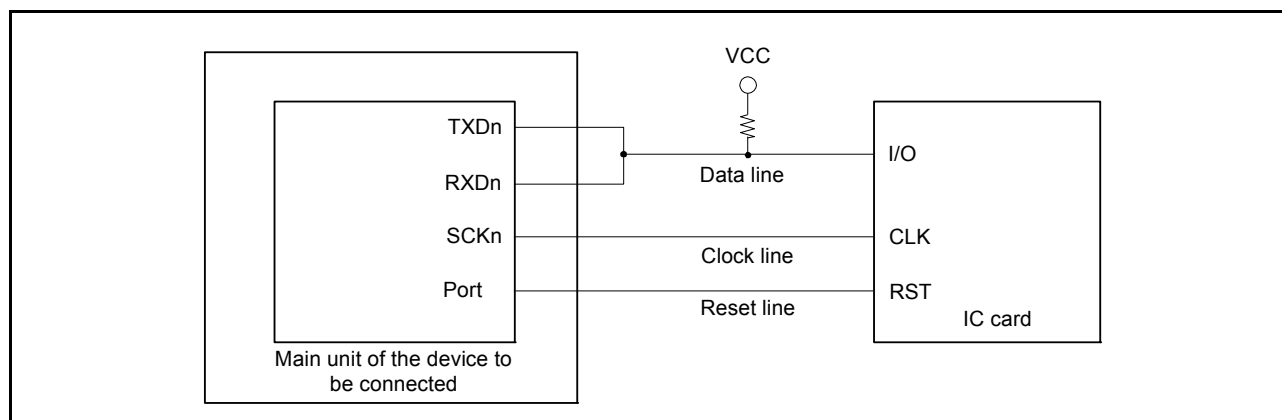
Figure 27.45 Example connection with a smart card (IC Card)
