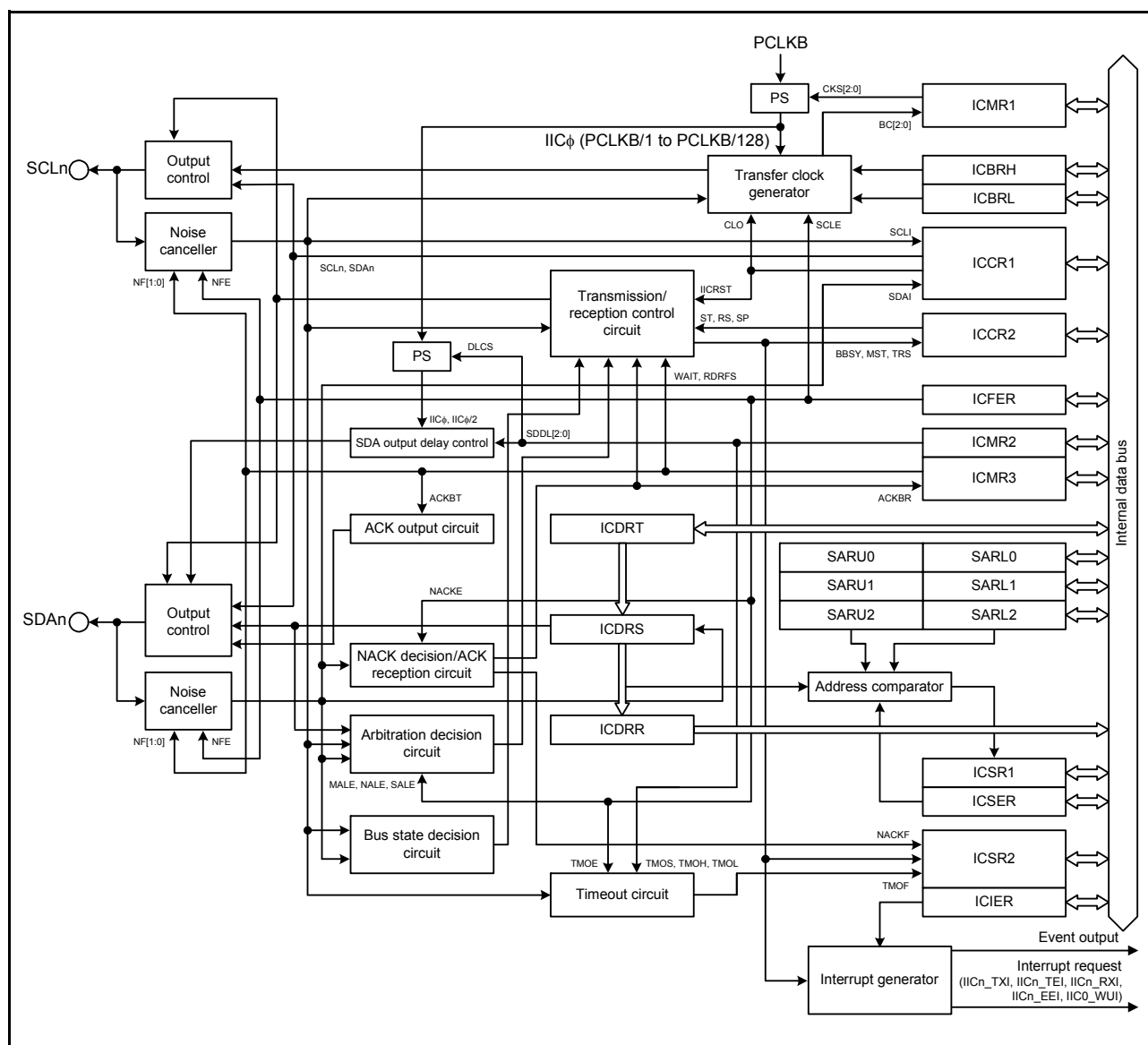
Figure 29.1 IIC block diagram
