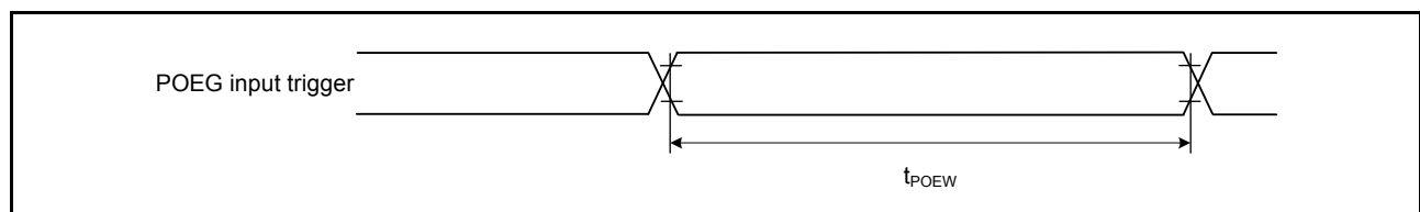
Figure 46.29 POEG input trigger timing
