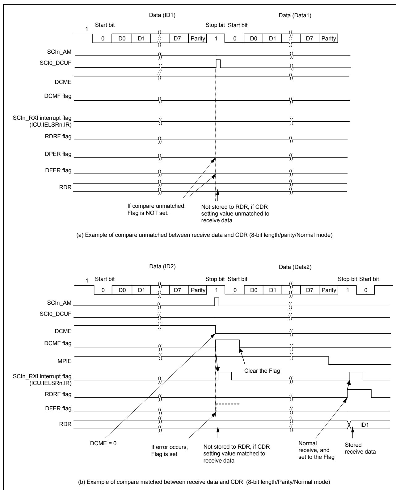
Figure 27.5 Example of address match (1) normal mode
