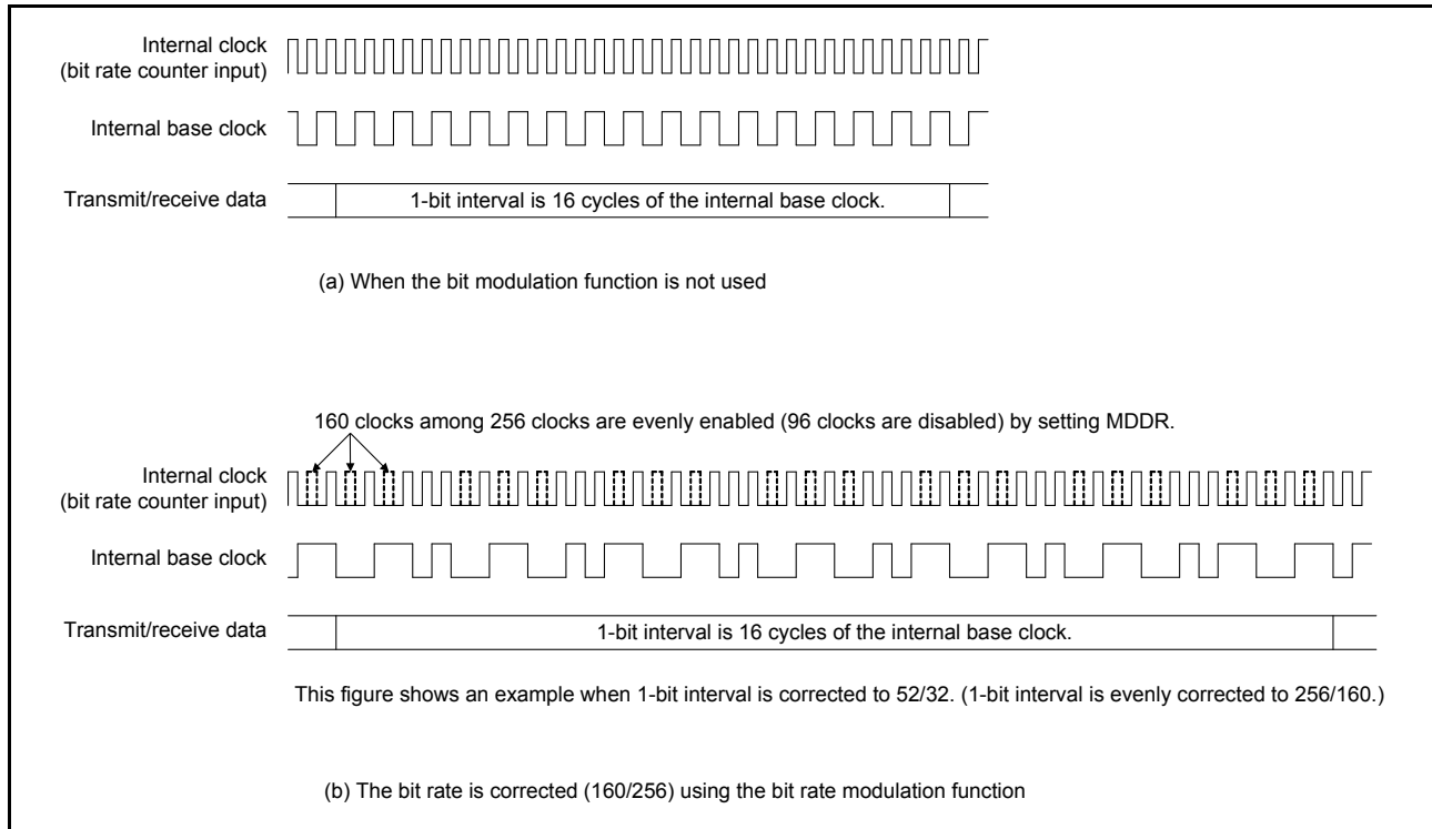
Figure 27.70 Example of internal base clock when bit rate modulation function is used
