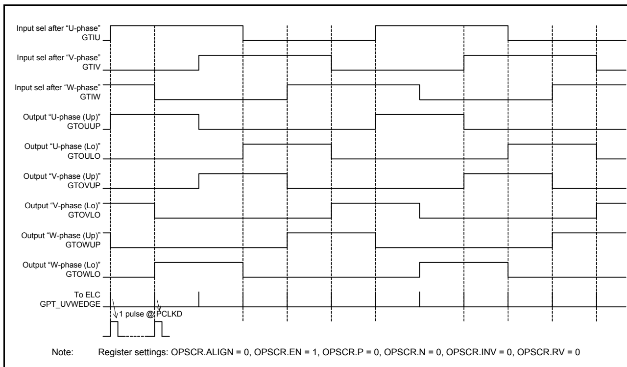
Figure 20.78 6-phase level output operation example
