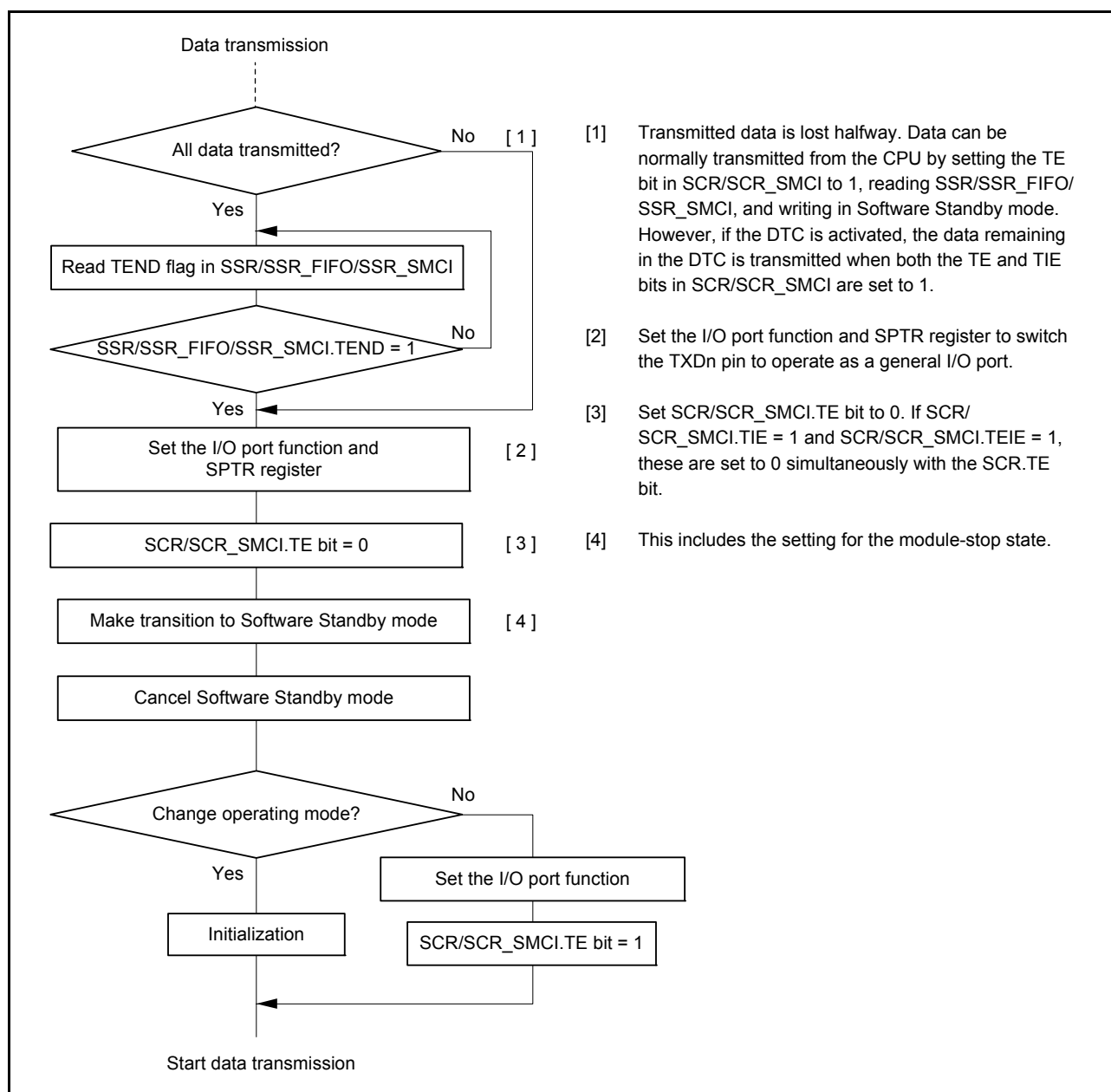
Figure 27.72 Example flow for transition to Software Standby mode during transmission
