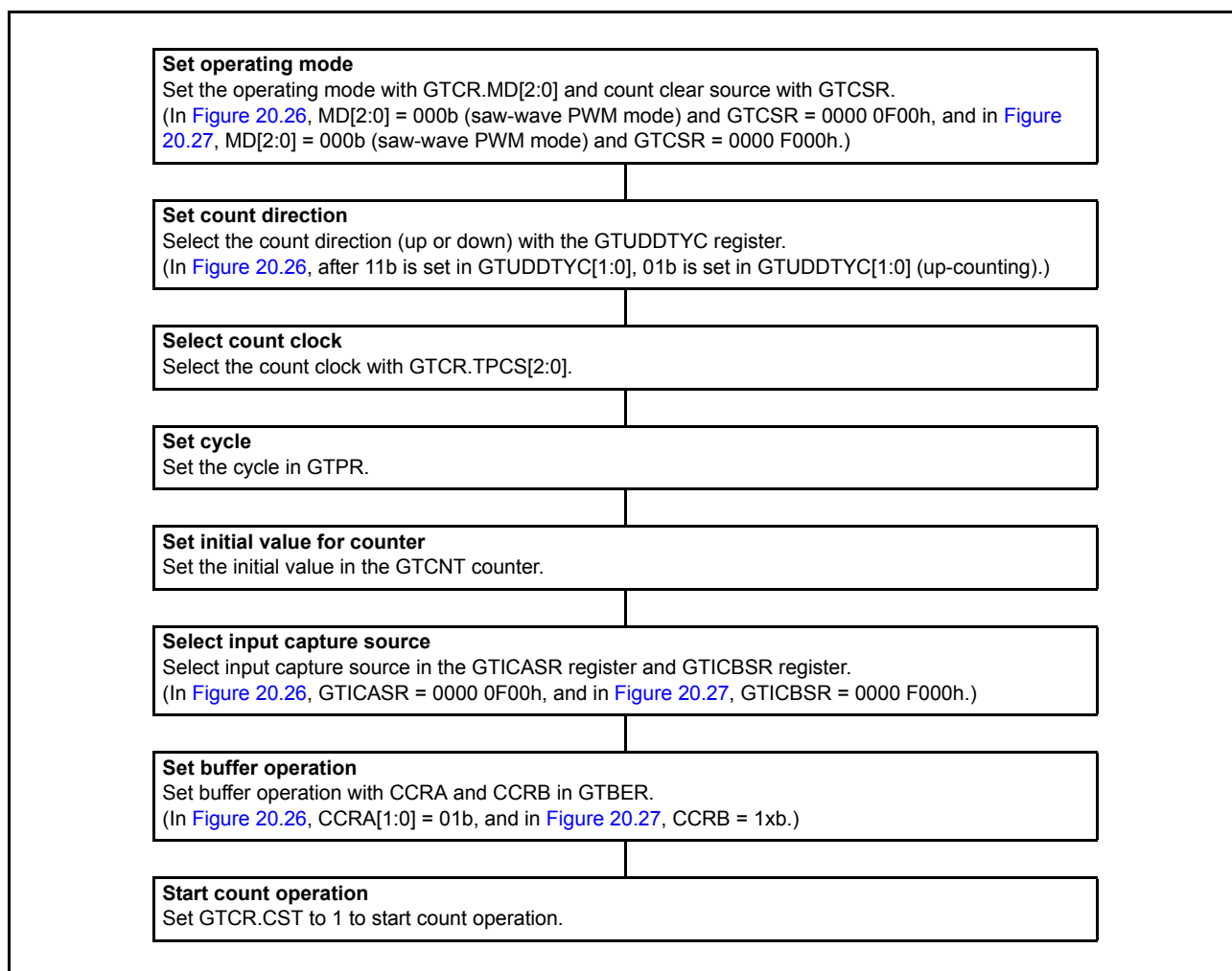
Figure 20.28 Example for setting GTCCRA and GTCCRB buffer operation for input capture
