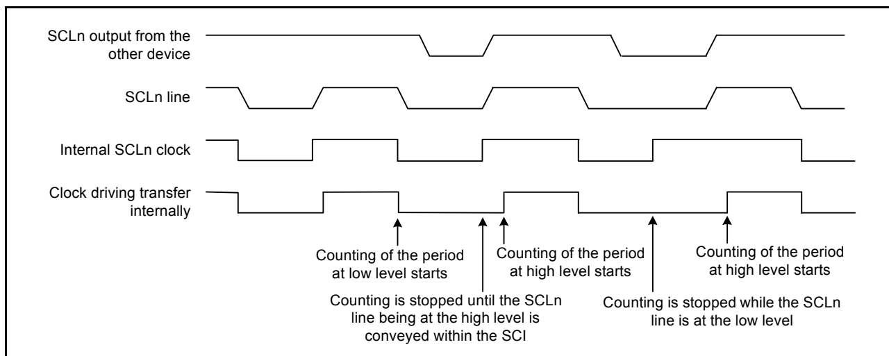
Figure 27.60 Example operations for clock synchronization
