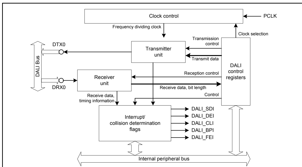
Figure 28.1 DALI block diagram
