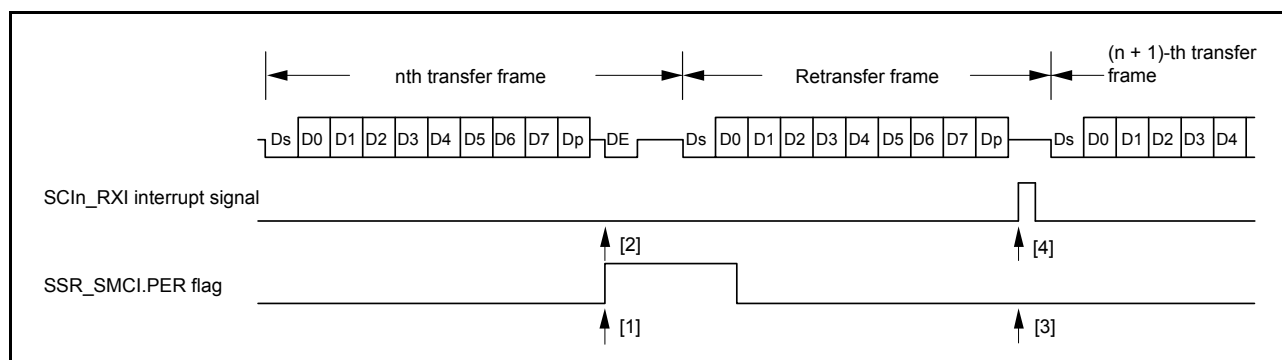
Figure 27.54 Data retransfer operation in SCI reception mode with data retransfer operation during reception
