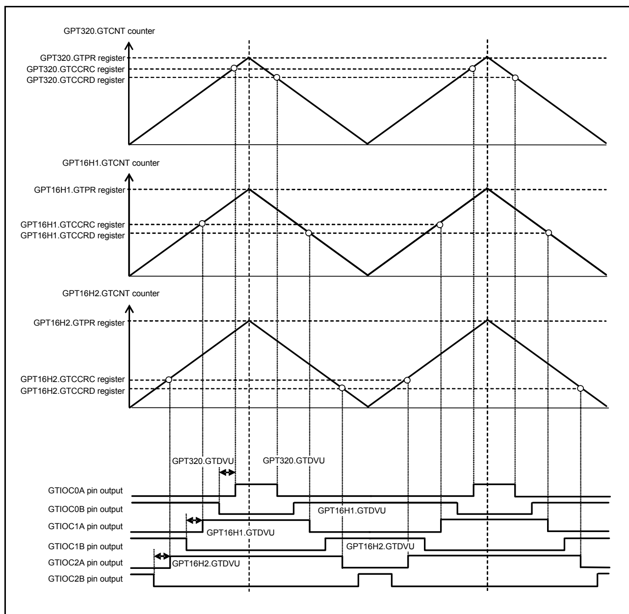
Figure 20.66 Example of 3-phase asymmetric triangle-wave complementary PWM output with automatic dead time setting
