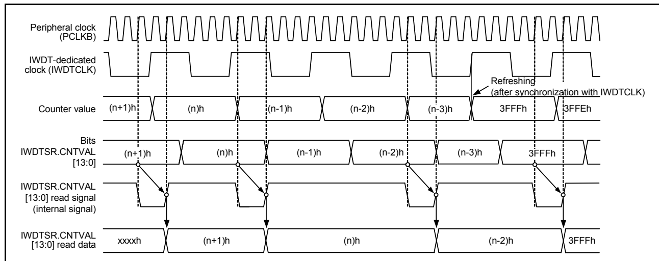
Figure 25.5 Processing for reading IWDT counter value when OFS0.IWDTCKS[3:0] = 0000b, OFS0.IWDTTOPS[1:0] = 11b
