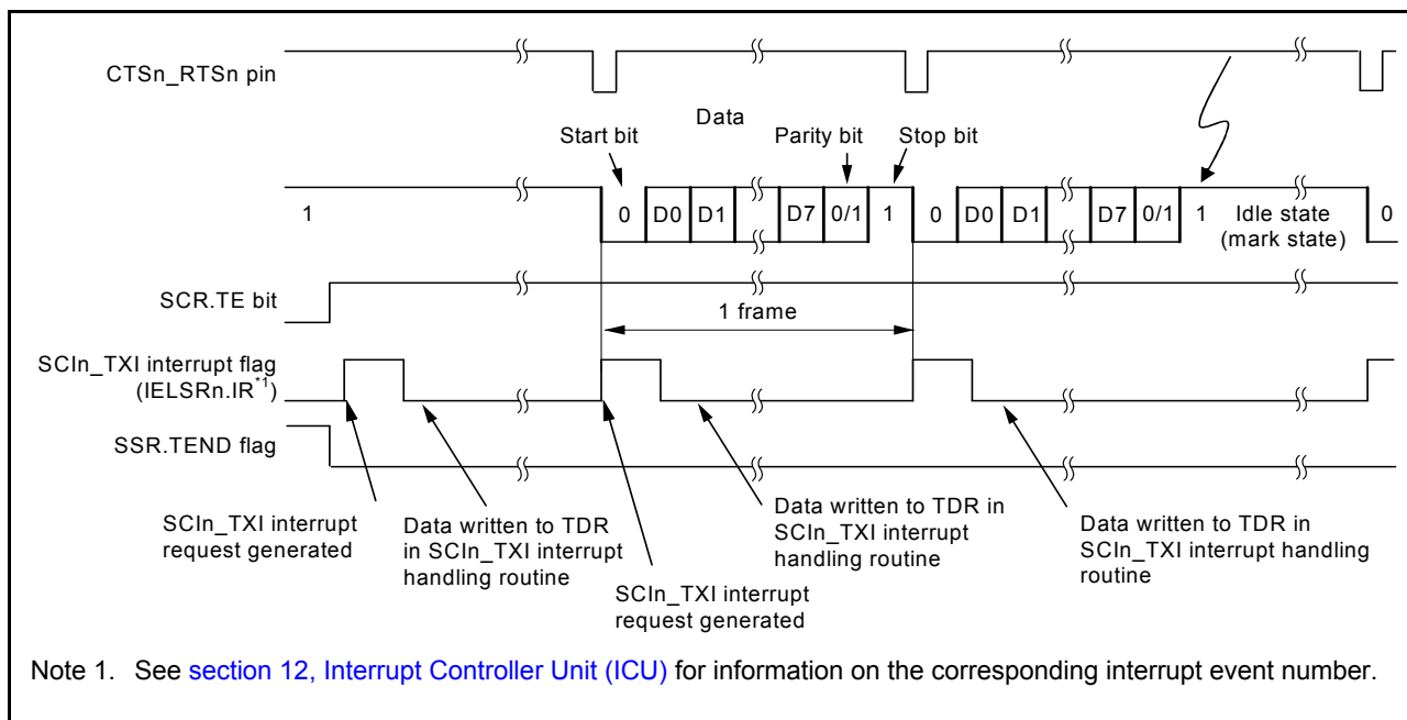
Figure 27.10 Example of operation for serial transmission in asynchronous mode (2) with 8-bit data, parity, 1 stop bit, CTS function used, at the beginning of transmission
