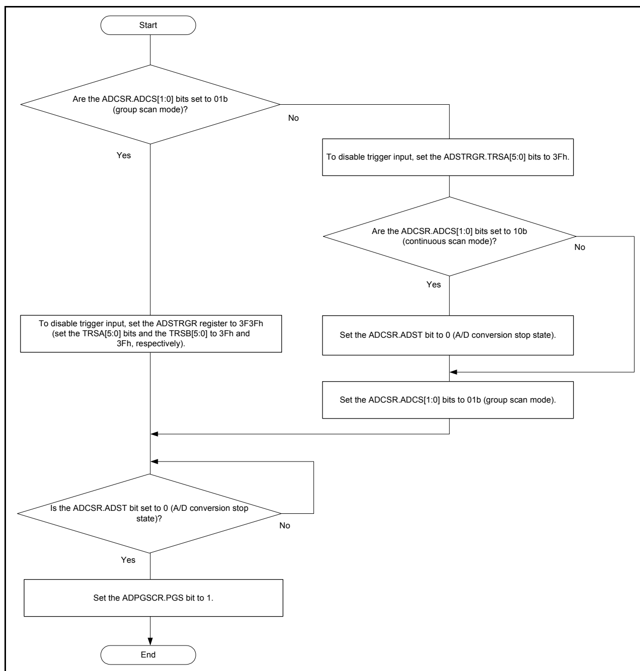
Figure 33.15 Flow of setting ADPGSCR.PGS bit
