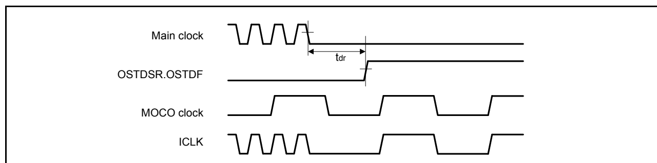
Figure 46.56 Oscillation stop detection timing
