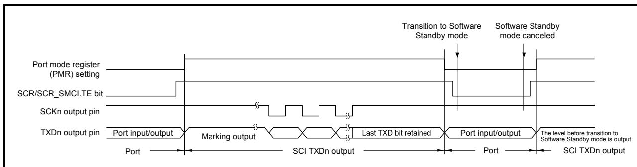
Figure 27.74 Port pin states during transition to Software Standby mode with internal clock and clock synchronous transmission
