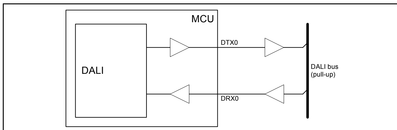
Figure 28.33 Example of external device connection
