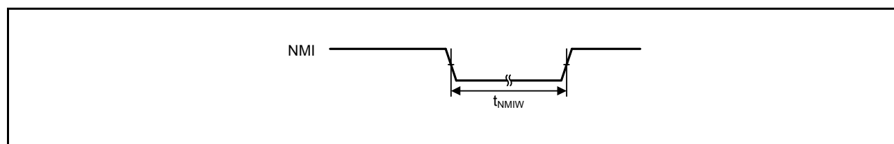
Figure 46.26 NMI interrupt input timing
