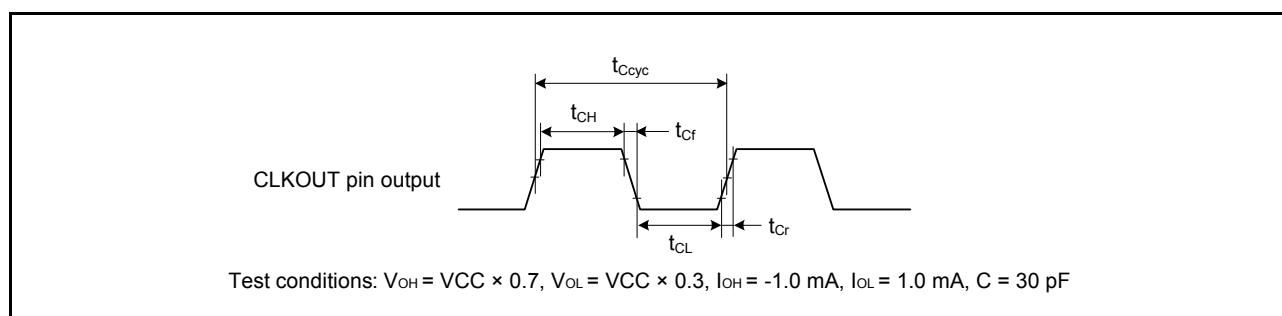
Figure 46.50 CLKOUT output timing
