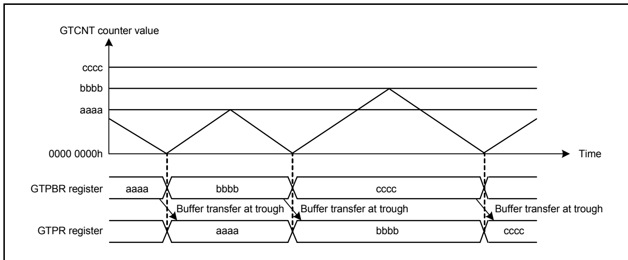
Figure 20.20 Example of GTPR buffer operation (triangle waves)
