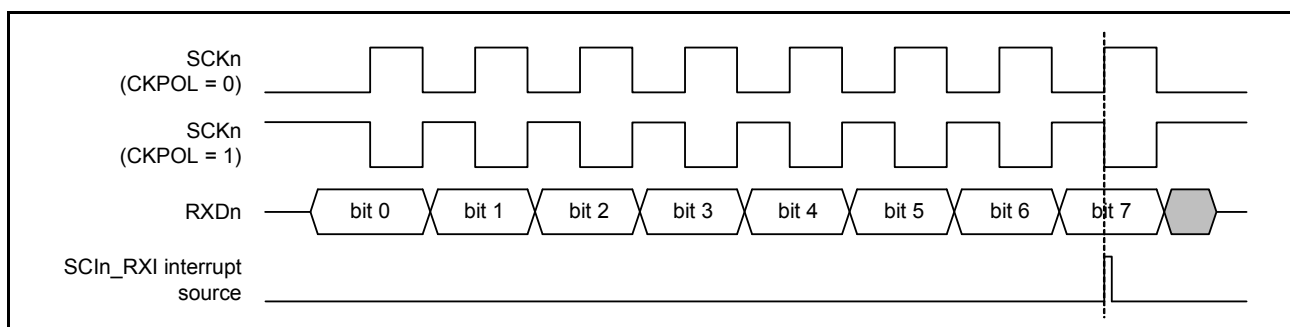
Figure 27.78 Timing of SCIn_RXI interrupt in simple SPI mode with clock delay
