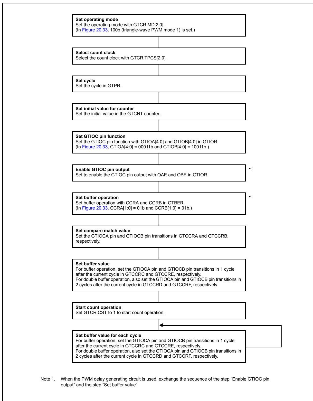
Figure 20.34 Example for setting triangle-wave PWM mode 1
