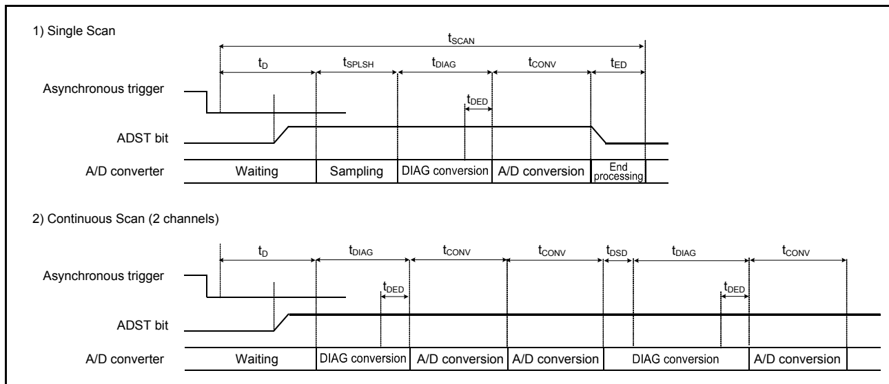
Figure 33.25 Scan conversion timing when activated by asynchronous trigger input (in case of ADTRG0)
