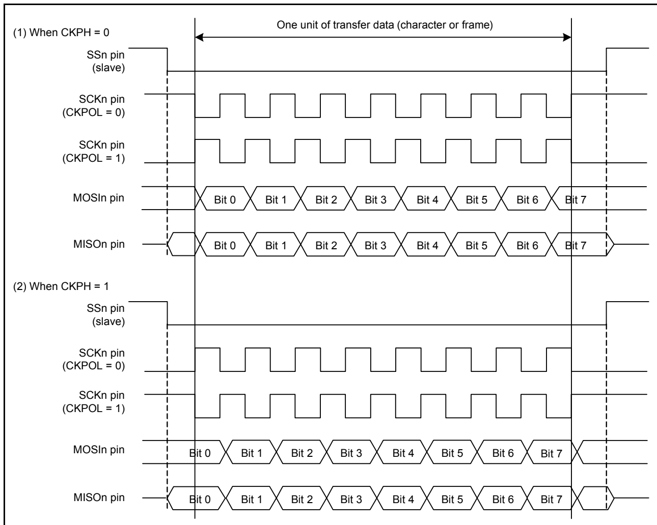
Figure 27.69 Relation between clock signal and transmit/receive data in simple SPI mode
