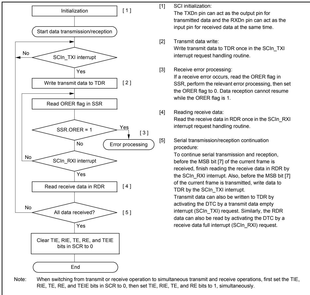
Figure 27.43 Example flow of simultaneous serial transmission and reception in clock synchronous mode
