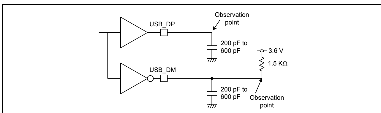
Figure 46.53 Test circuit for Low-Speed (LS) connection
