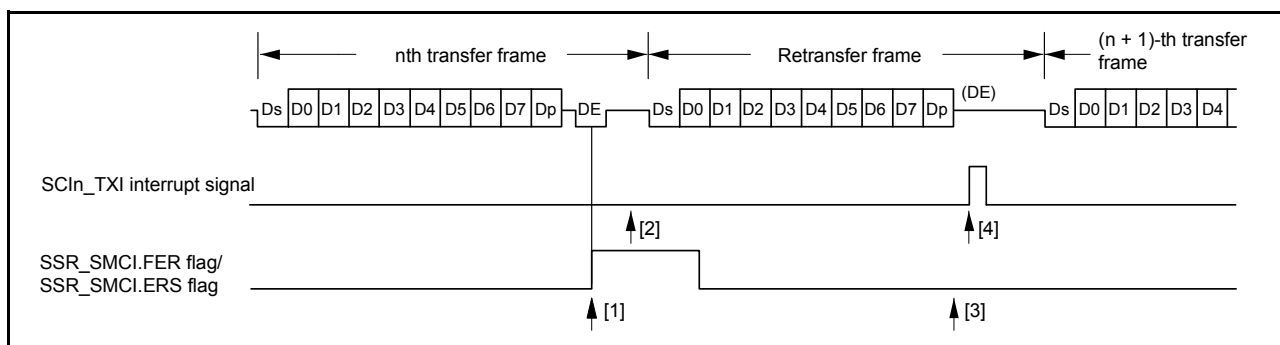
Figure 27.51 Data retransfered operation in SCI transmission mode
