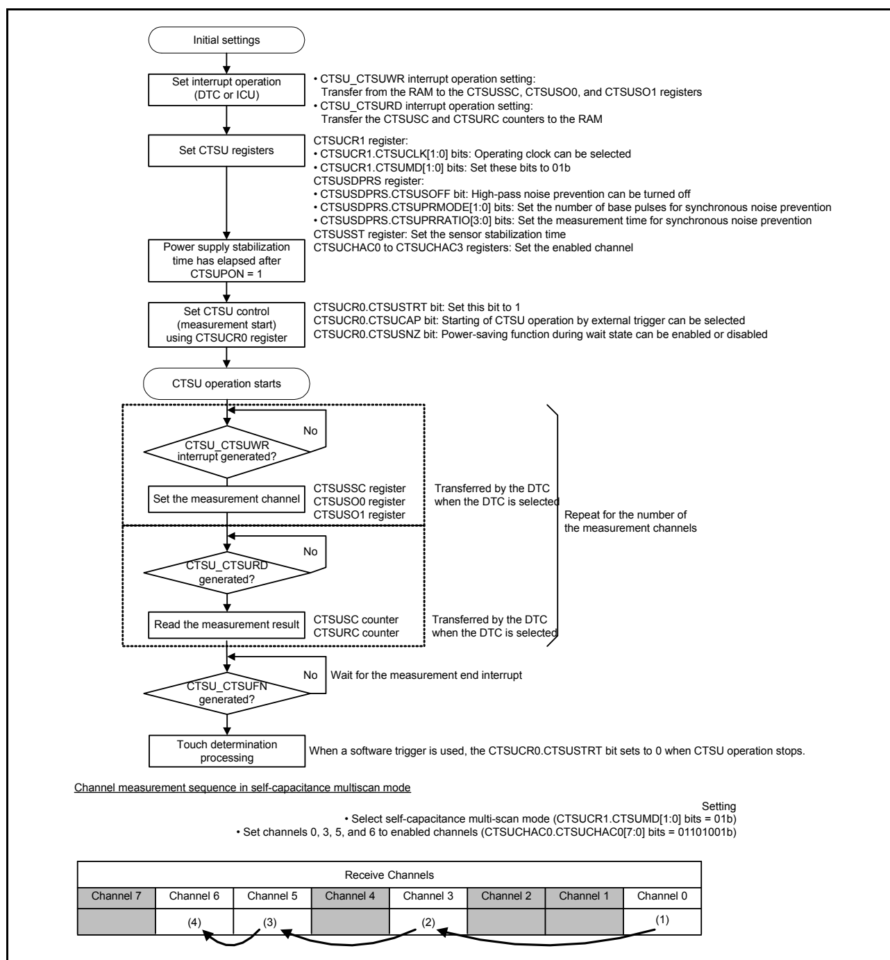
Figure 39.14 Software flow and operation example of self-capacitance multi-scan mode
