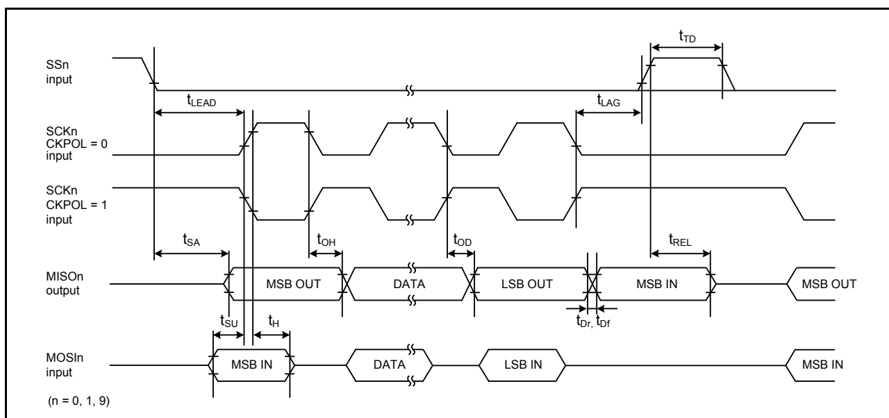
Figure 46.39 SCI simple SPI mode timing (slave, CKPH = 1)
