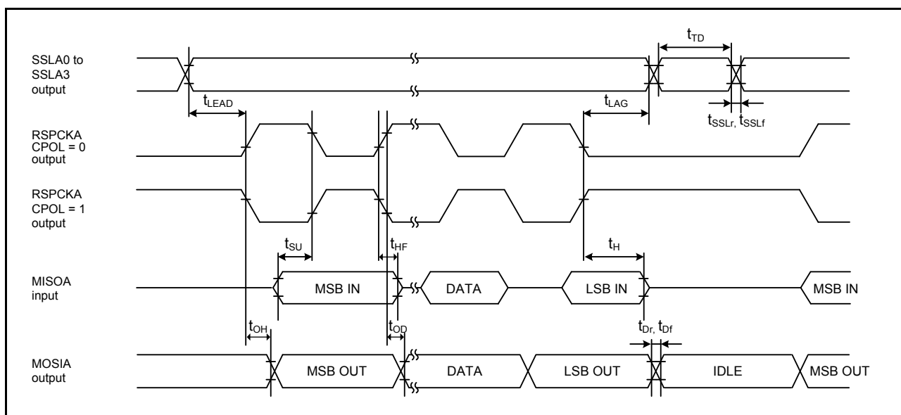
Figure 46.46 SPI timing (master, CPHA = 1) (bit rate: PCLKB division ratio is set to 1/2)
