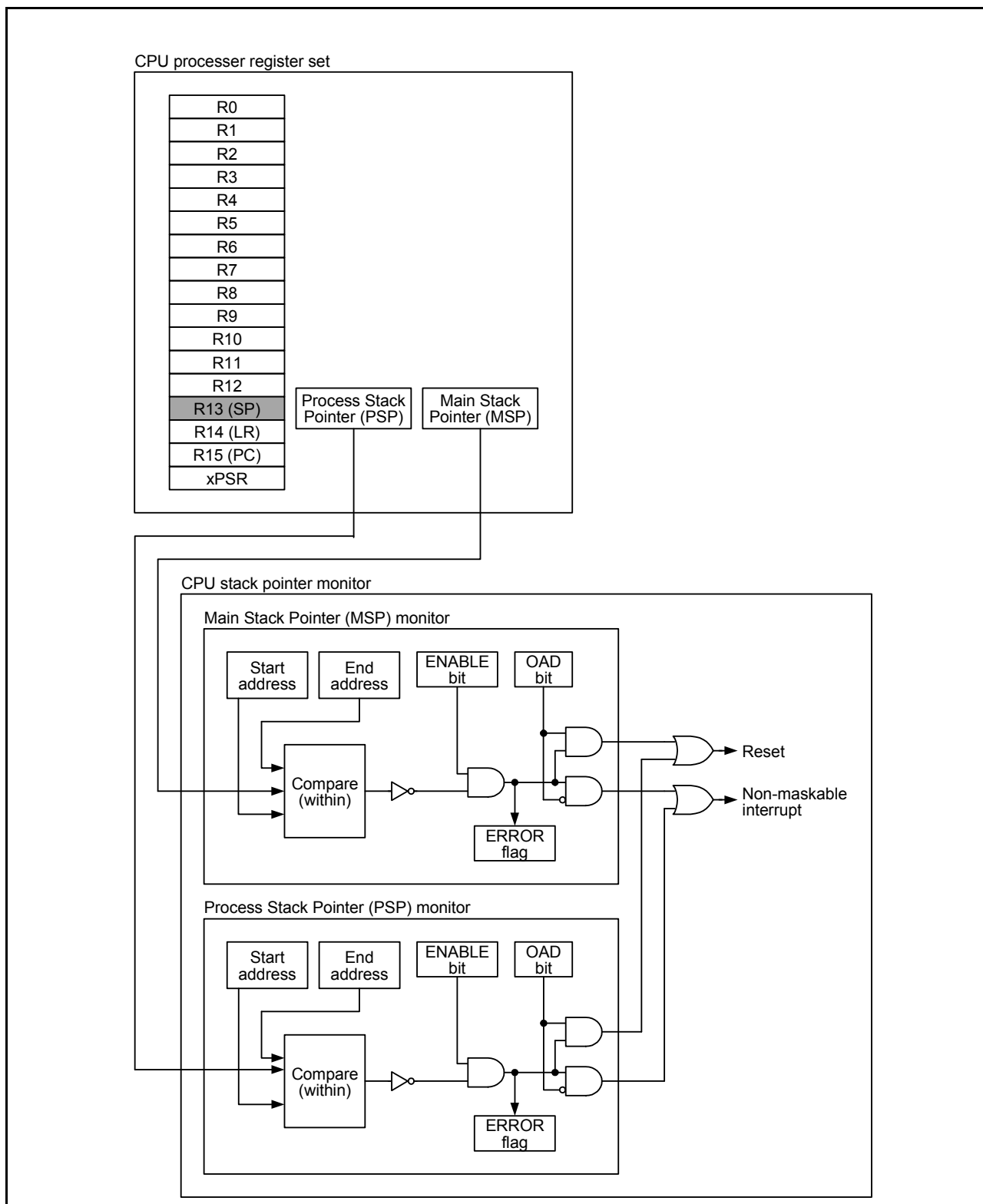
Figure 14.1 CPU Stack Pointer Monitor block diagram
