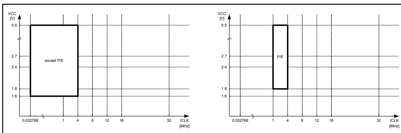
Figure 10.4 Operating voltages and frequencies in Low-voltage mode
