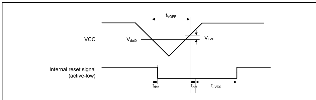
Figure 46.59 Voltage detection circuit timing ( V_{det0} )
