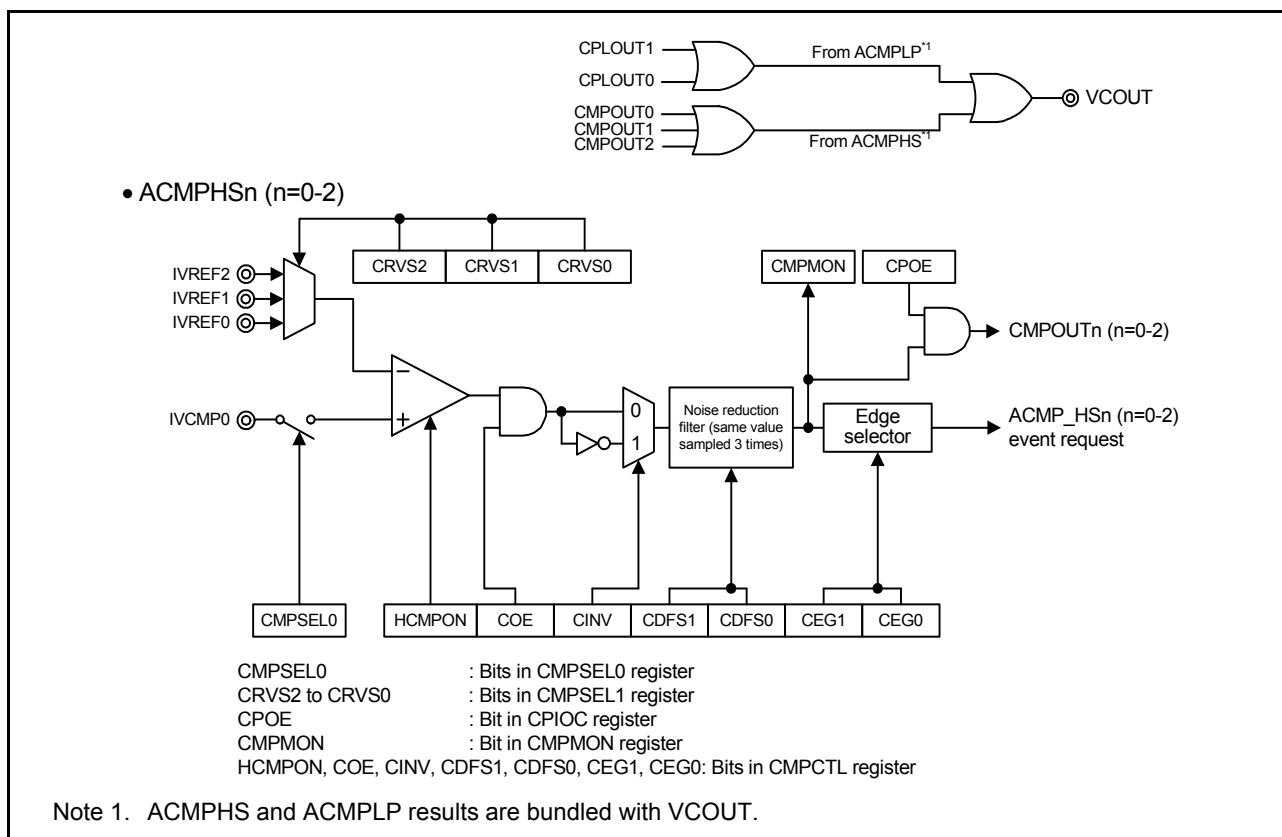
Figure 37.1 ACMPHS block diagram
