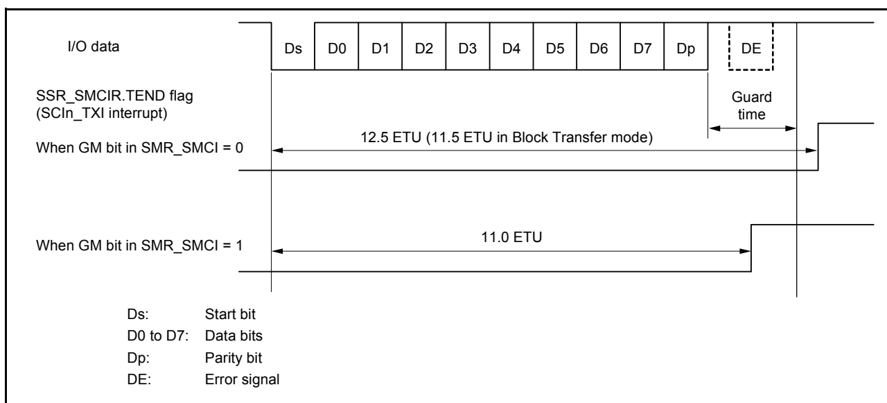
Figure 27.52 SSR.TEND flag generation timing during transmission
