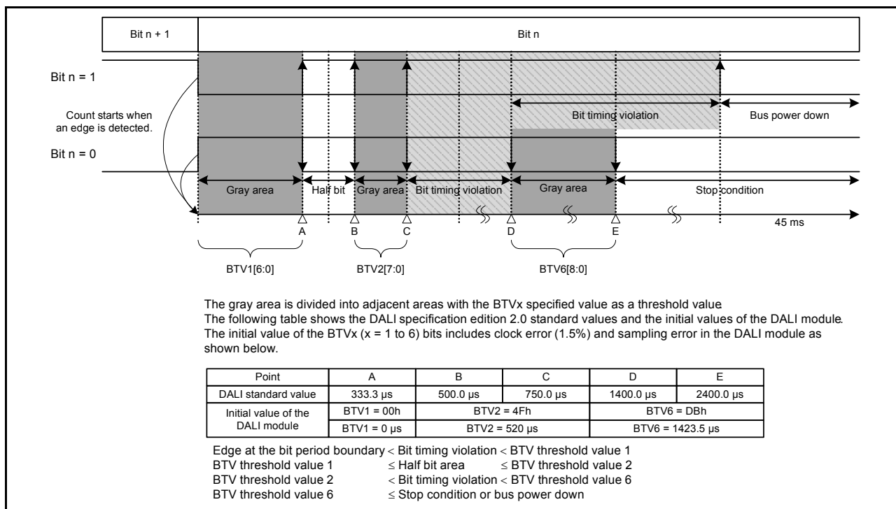
Figure 28.10 Bit timing violation 1
