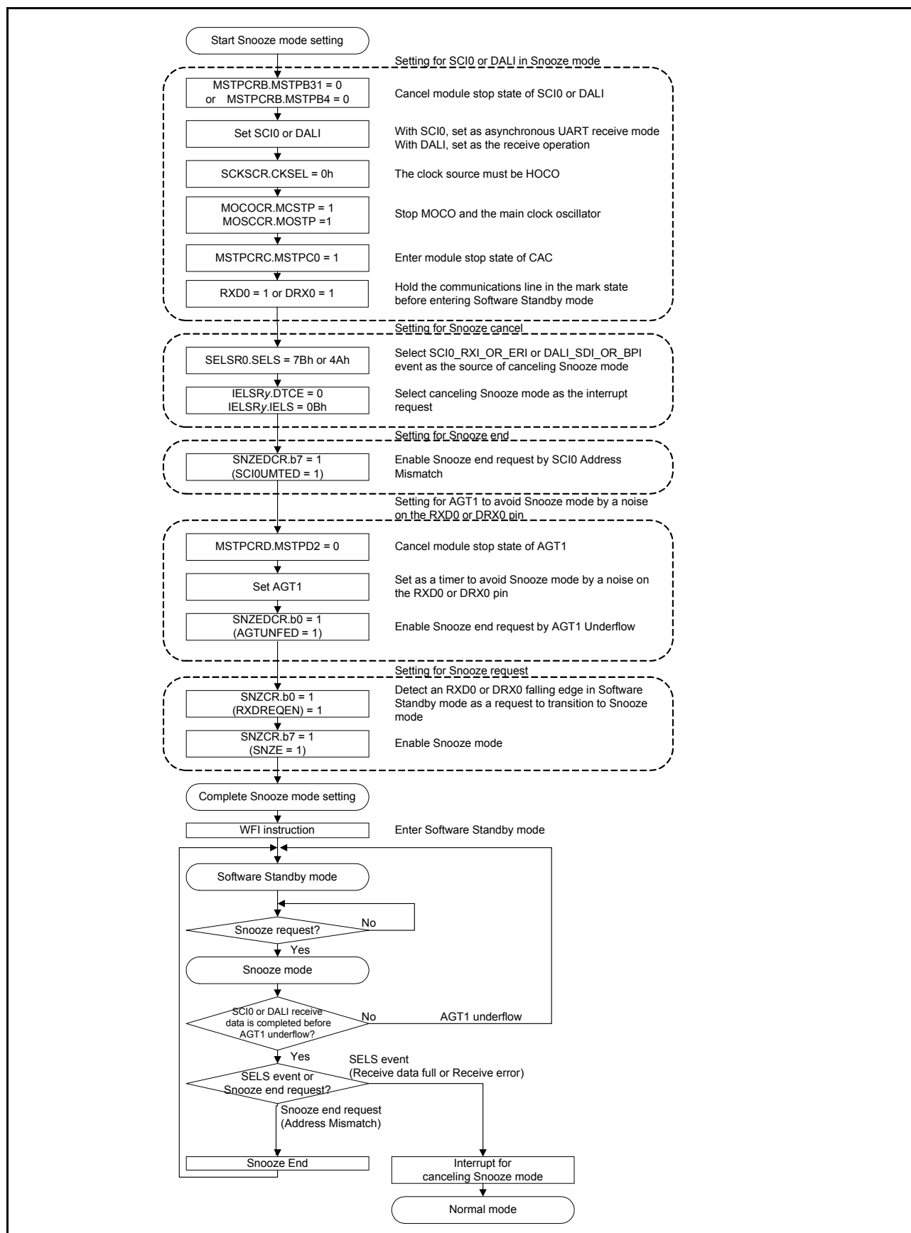
Figure 10.12 Setting example of using SCI0 or the DALI in Snooze mode entry
