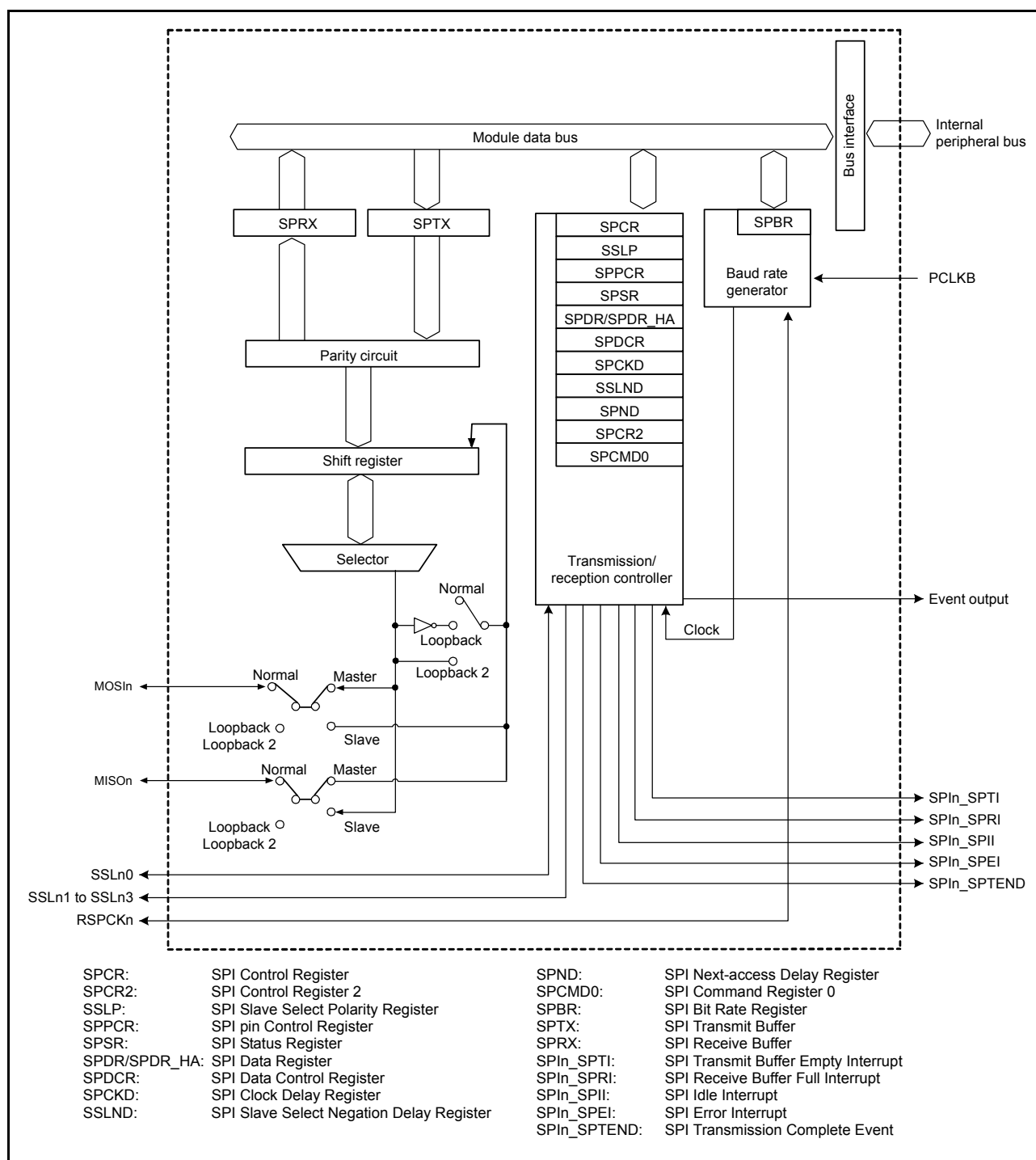
Figure 31.1 SPI block diagram
