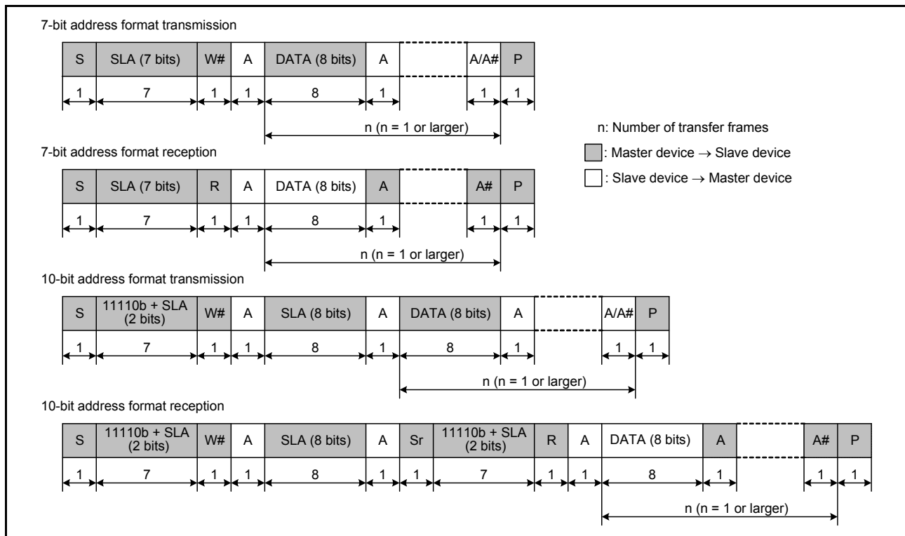
Figure 27.57 I 2 C bus format
