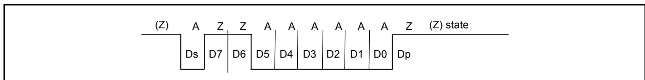
Figure 27.48 Inverse convention with SDIR in SCMR = 1, SINV in SCMR = 1, and PM in SMR_SMCI = 1
