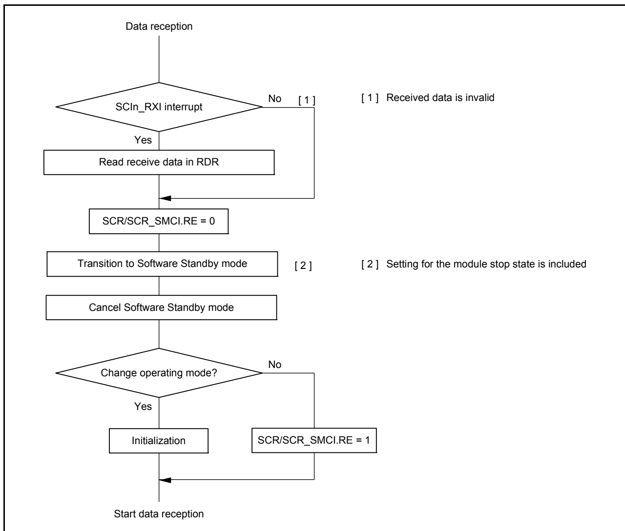
Figure 27.75 Example flow for transition to Software Standby mode during reception
