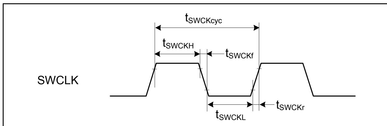
Figure 46.62 SWD SWCLK timing
