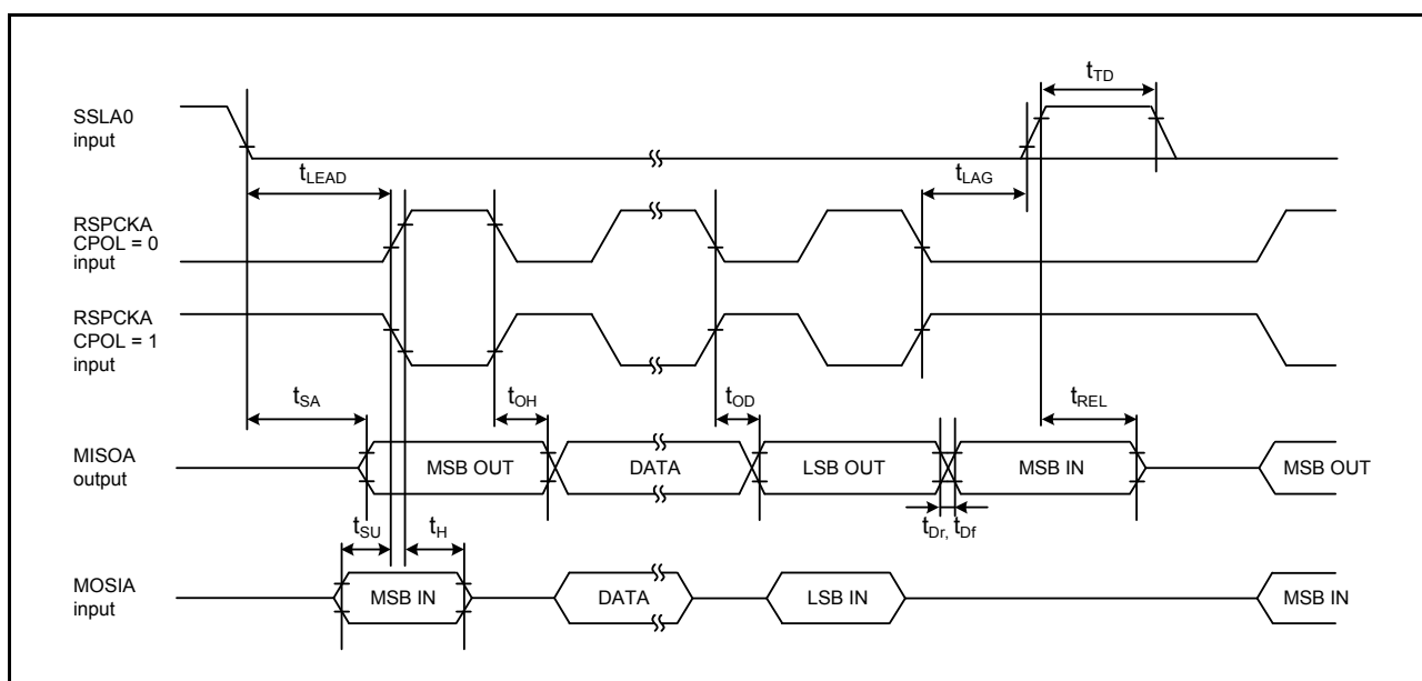
Figure 46.47 SPI timing (slave, CPHA = 0)
