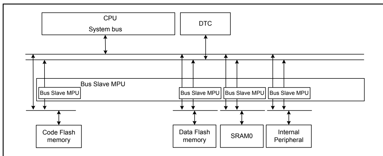
Figure 14.9 Block diagram of the Bus Slave MPU
