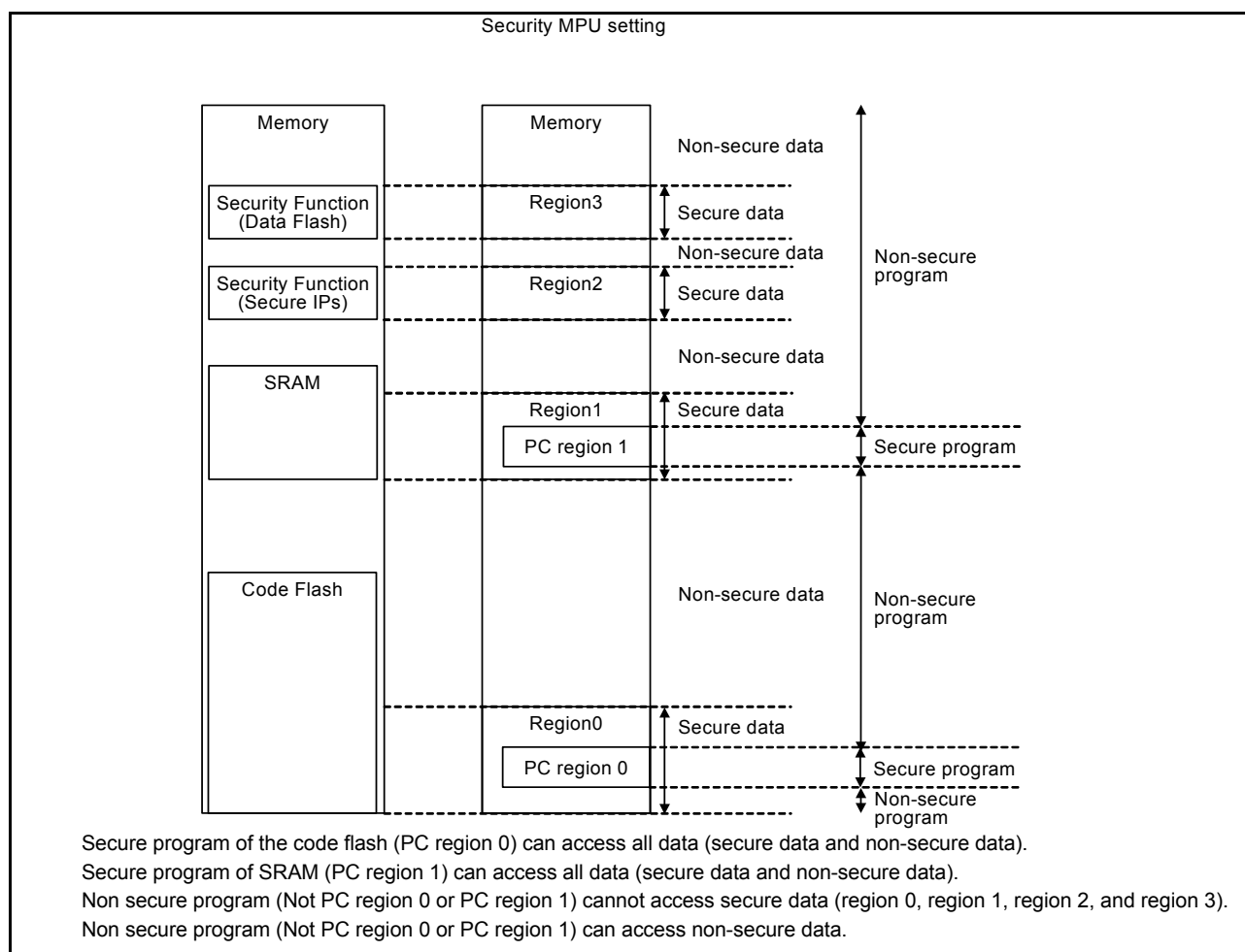
Figure 14.11 Use case of Security MPU
