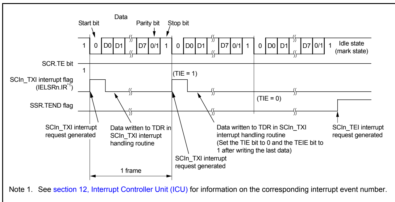
Figure 27.11 Example of operation for serial transmission in asynchronous mode (3) with 8-bit data, parity, 1 stop bit, CTS function not used, from the middle of transmission until transmission completion
