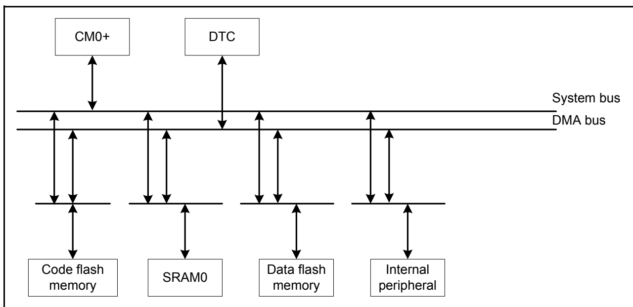
Figure 13.1 Bus configuration
