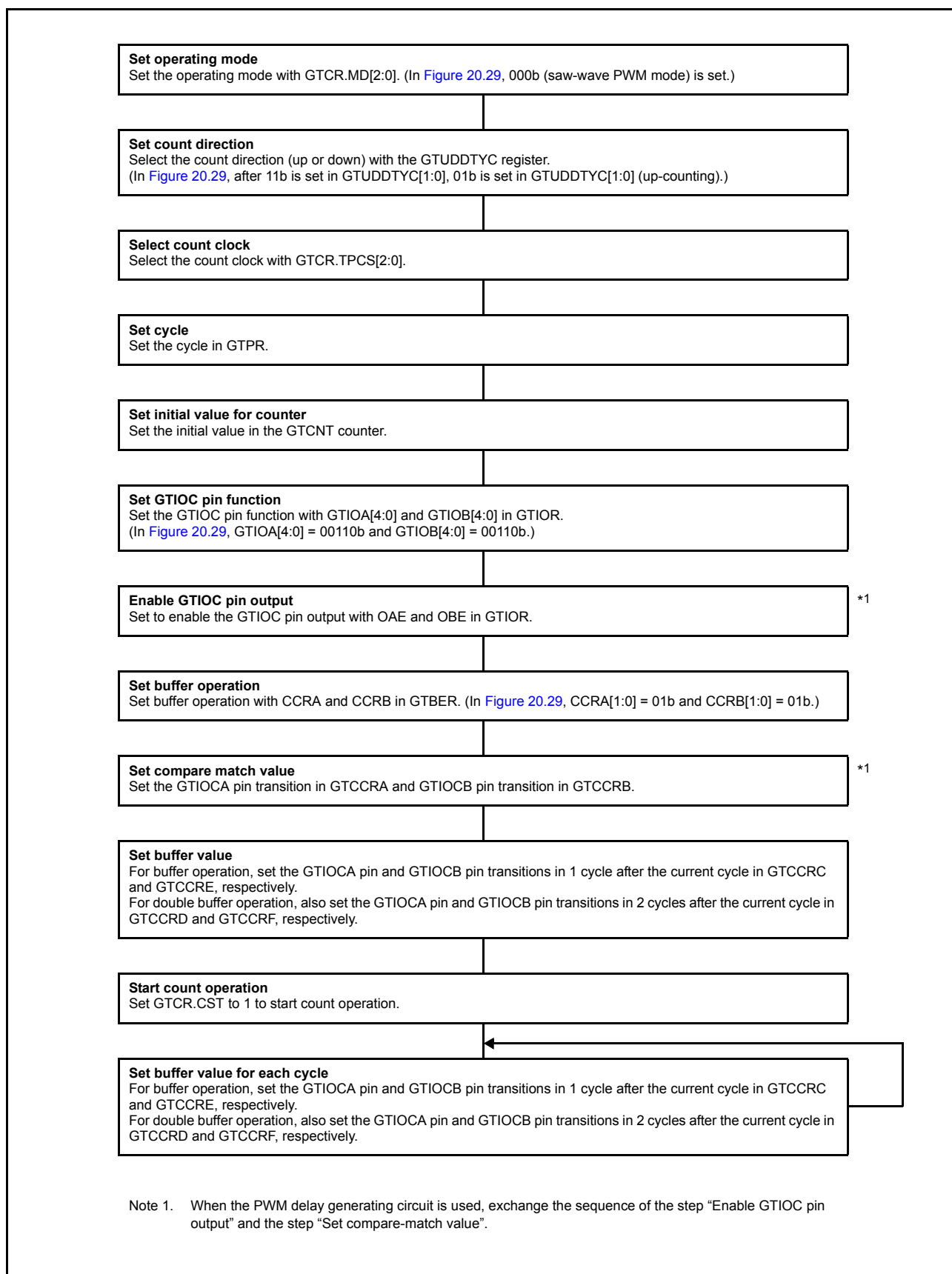
Figure 20.30 Example for setting saw-wave PWM mode
