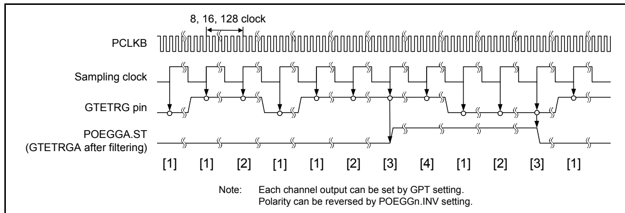
Figure 19.4 External trigger output timing to GPT
