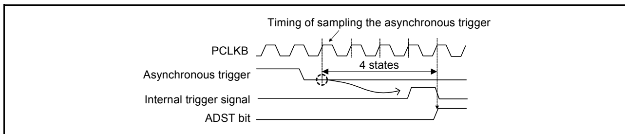
Figure 33.29 Asynchronous trigger input timing
