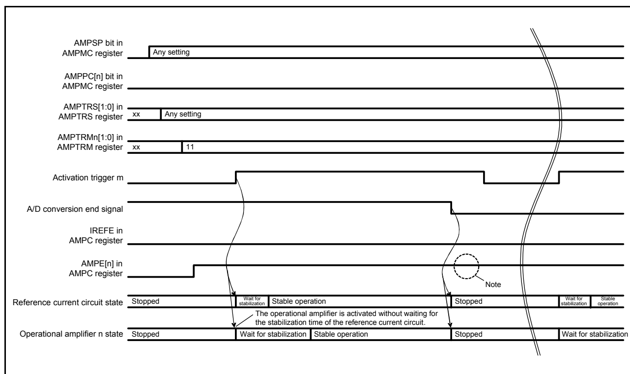
Figure 36.5 Operational amplifier control operation with activation and A/D trigger mode (1) and when the reference current circuit and operational amplifier are activated by an activation trigger and stopped by an A/D conversion end (trigger)
