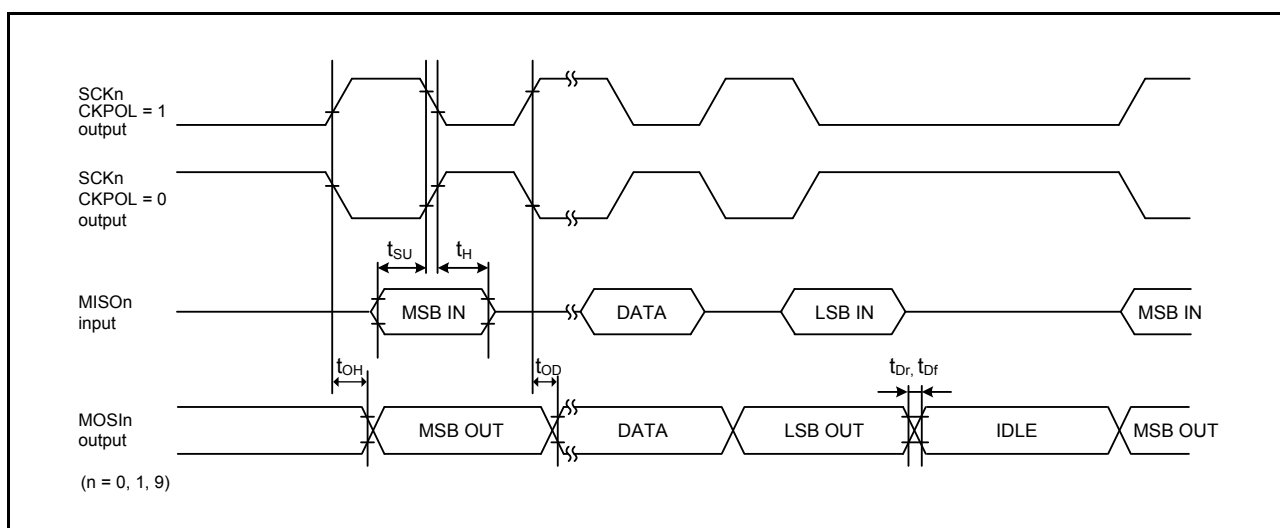
Figure 46.38 SCI simple SPI mode timing (master, CKPH = 0)
