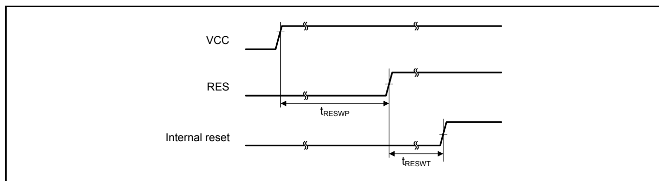
Figure 46.22 Reset input timing at power-on
