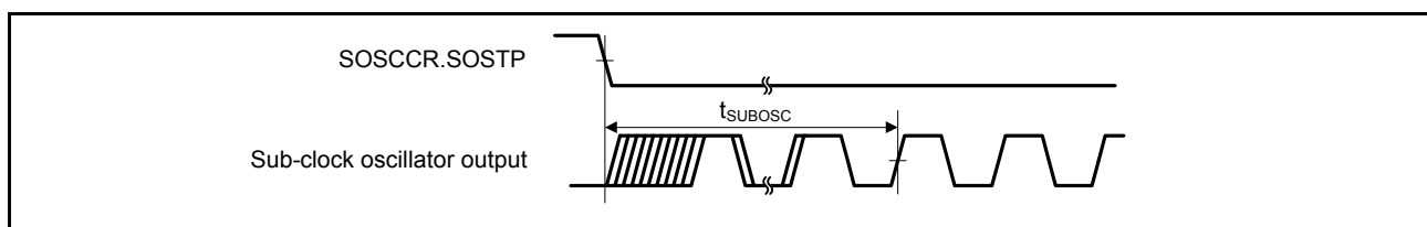
Figure 46.21 Sub-clock oscillation start timing
