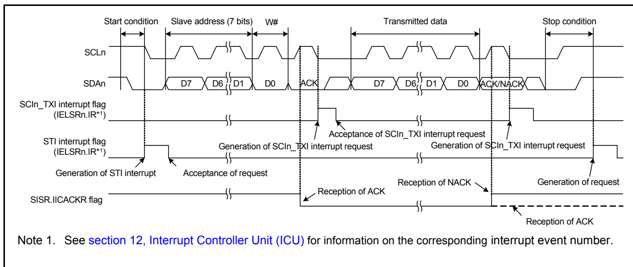
Figure 27.63 Example 1 of operations for master transmission in simple IIC bus mode with 7-bit slave addresses, transmission interrupts, and reception interrupts
