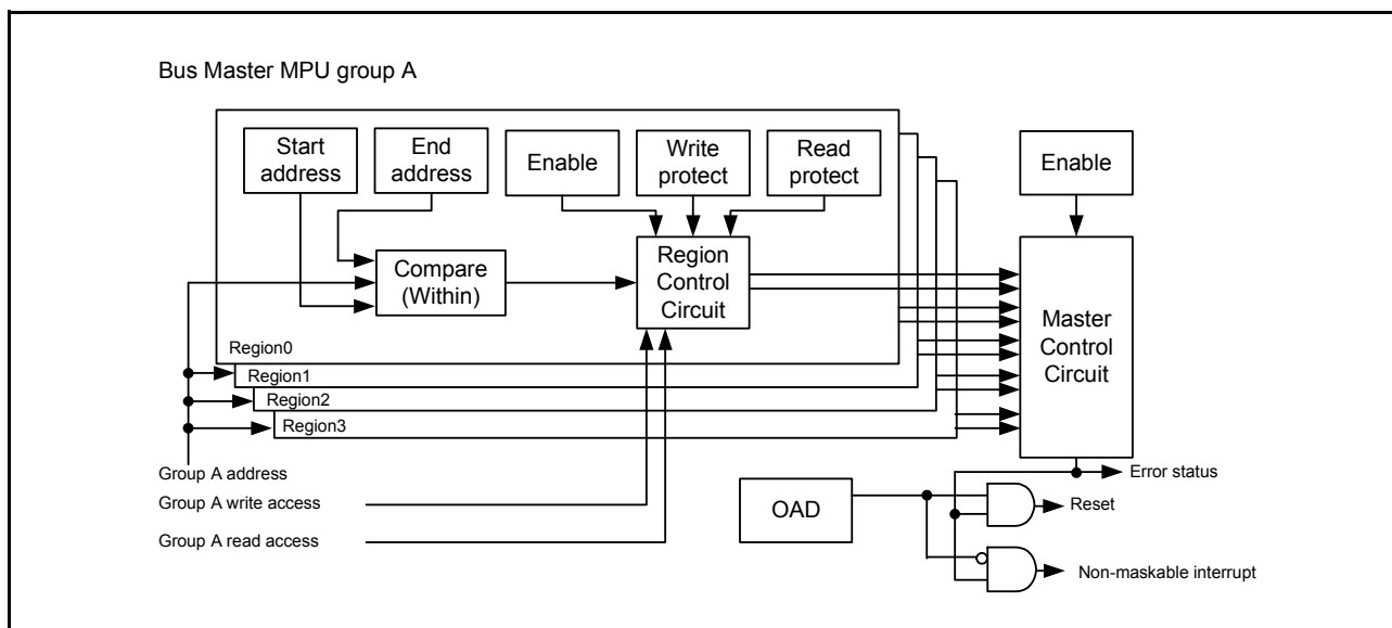
Figure 14.4 MPU bus master group A
