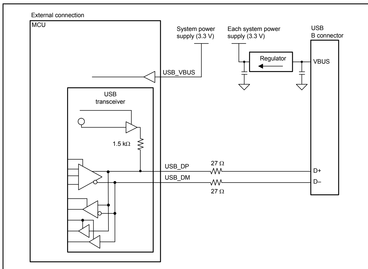
Figure 26.6 Functional connection sample of USB connector in bus-powered state
