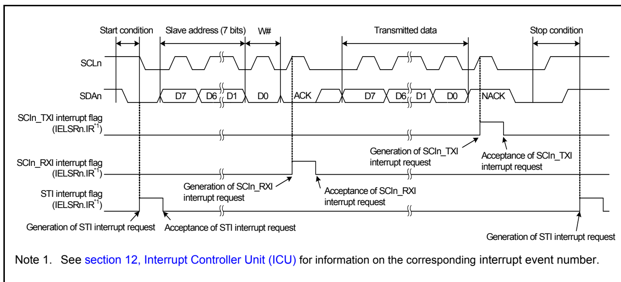
Figure 27.64 Example 2 of operations for master transmission in simple IIC bus mode with 7-bit slave addresses, ACK interrupts, and NACK interrupts
