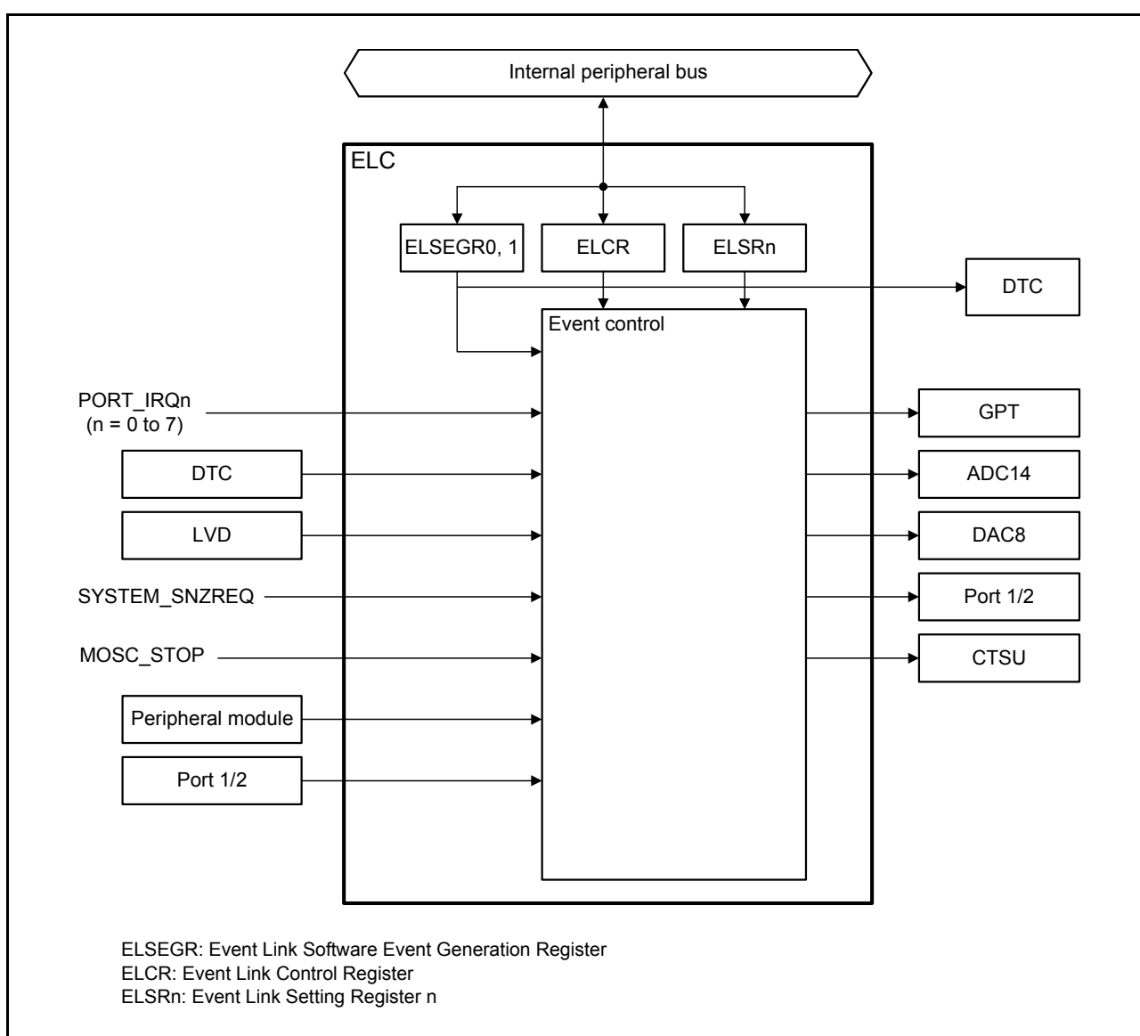
Figure 16.1 ELC block diagram when n = 0 to 3, 8, 9, 14, 15, 18 to 21
