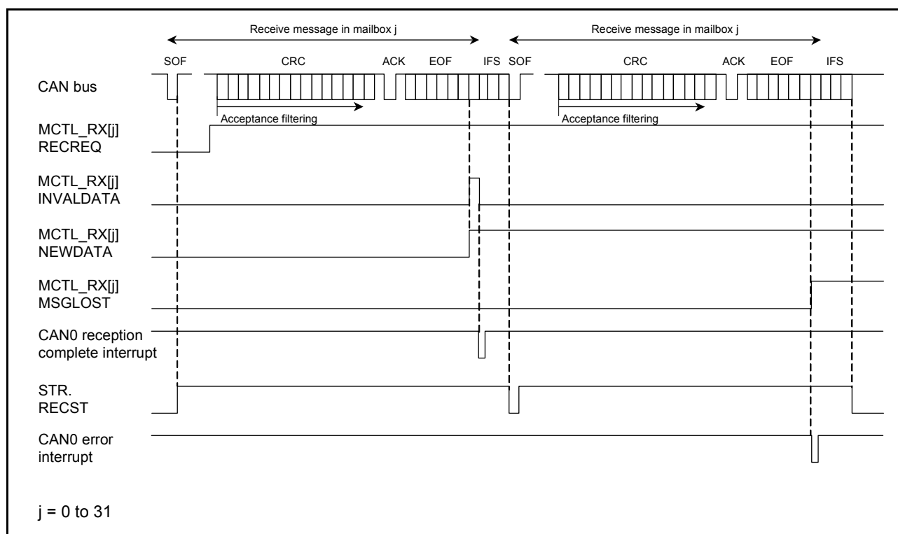
Figure 30.19 Operation example of data frame reception in overrun mode
