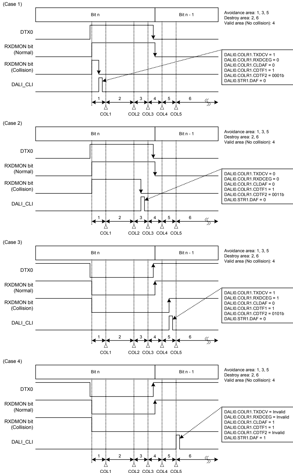
Figure 28.18 Usage example of collision detection information 2
