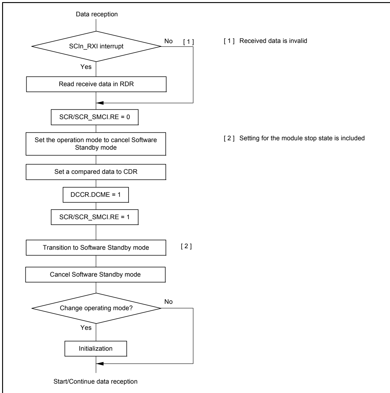
Figure 27.76 Example flow for transition to Software Standby mode during reception with address match
