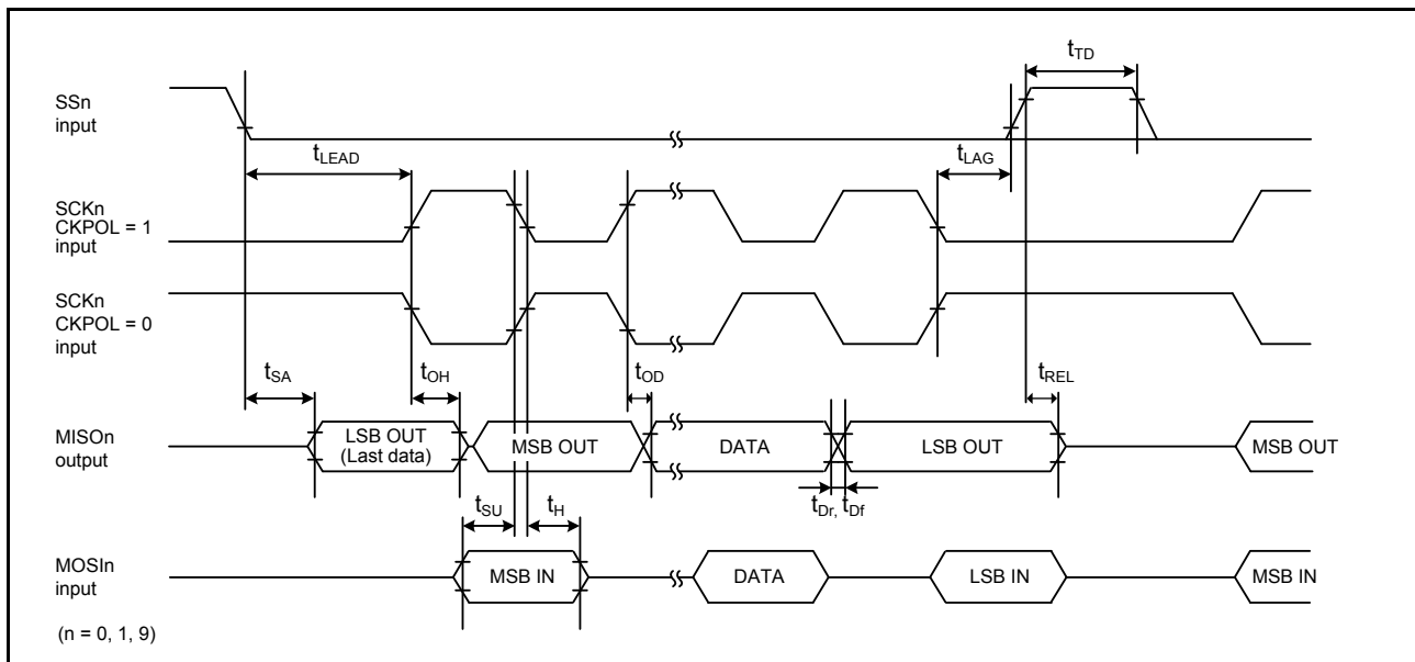
Figure 46.40 SCI simple SPI mode timing (slave, CKPH = 0)
