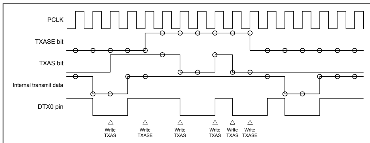
Figure 28.2 DTX0 pin level control
