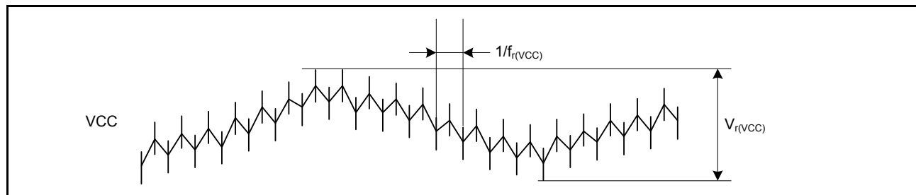
Figure 46.17 Ripple waveform
