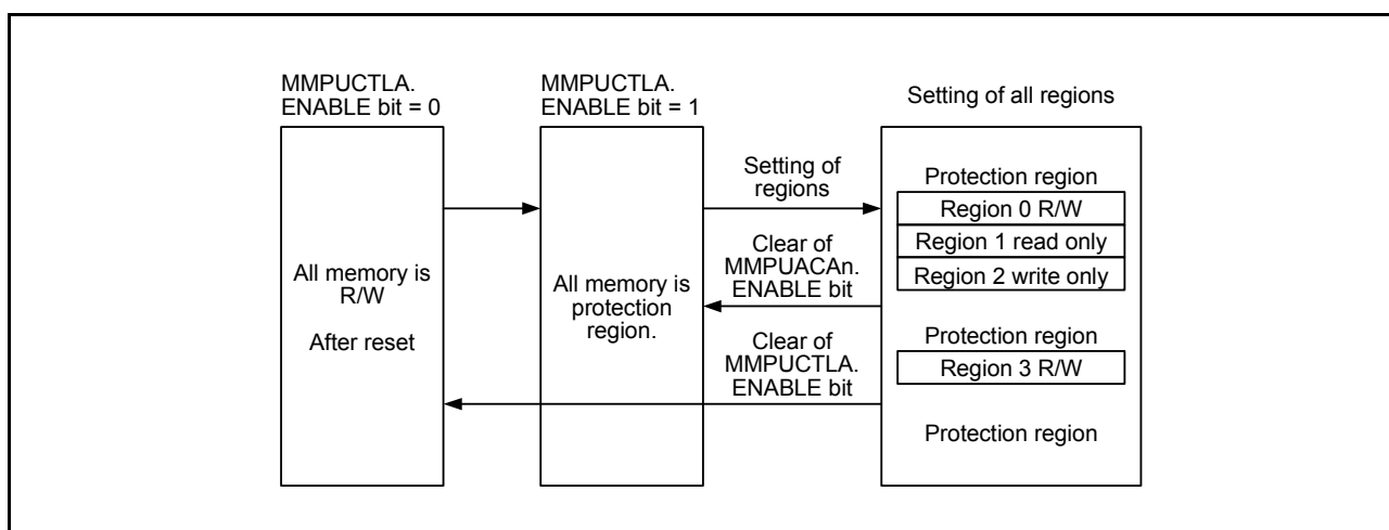
Figure 14.5 Use case of Bus Master MPU
