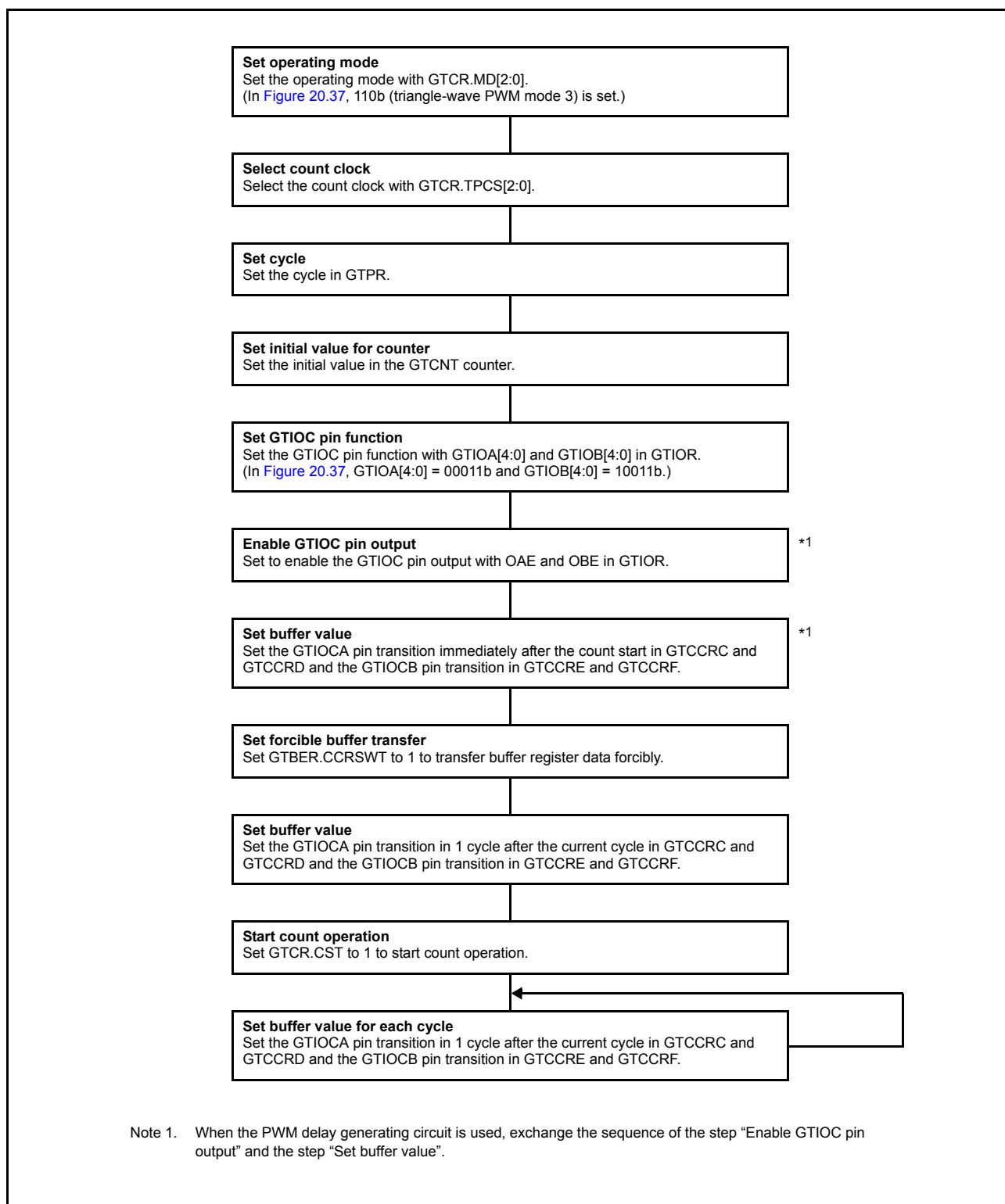
Figure 20.38 Example for setting triangle-wave PWM mode 3
