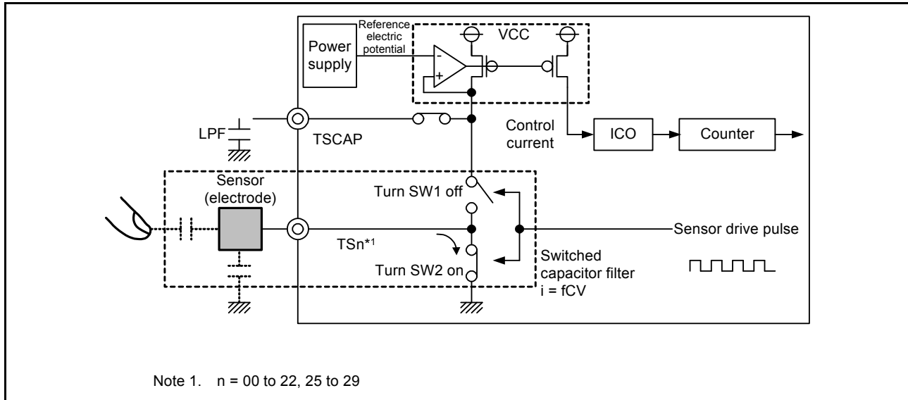
Figure 39.6 Discharging operation
