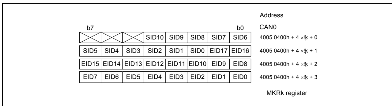
Figure 30.14 Structure of the MKRk registers (k = 0 to 7)
