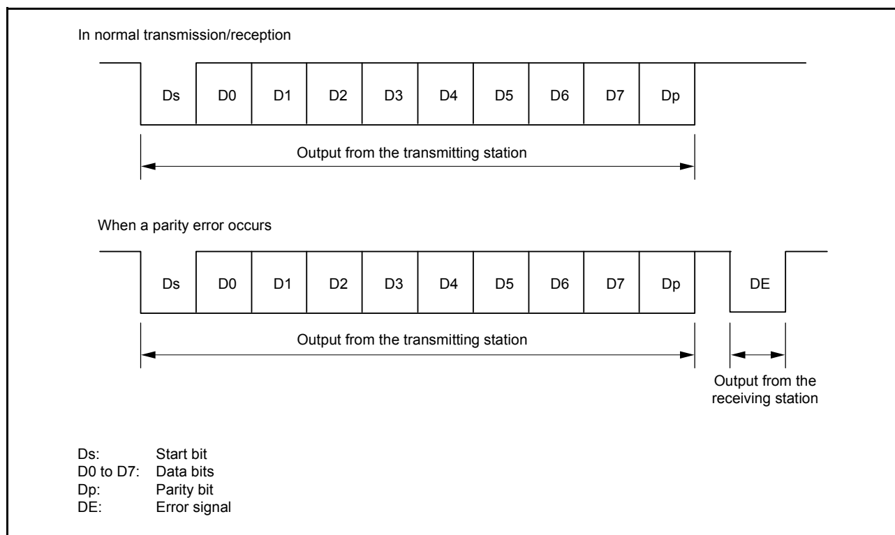
Figure 27.46 Data formats in smart card interface mode
