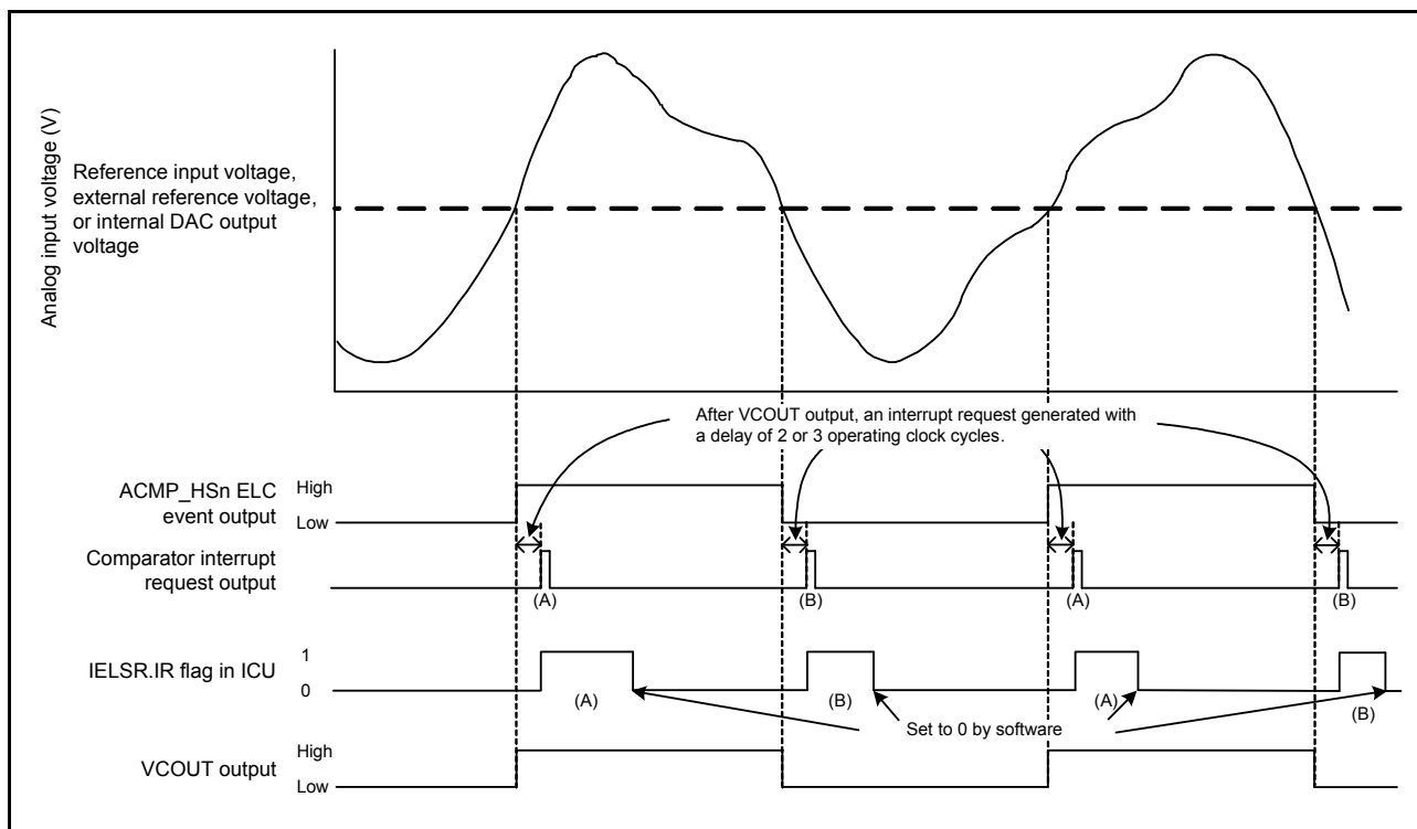
Figure 37.2 ACMPHS operation example
