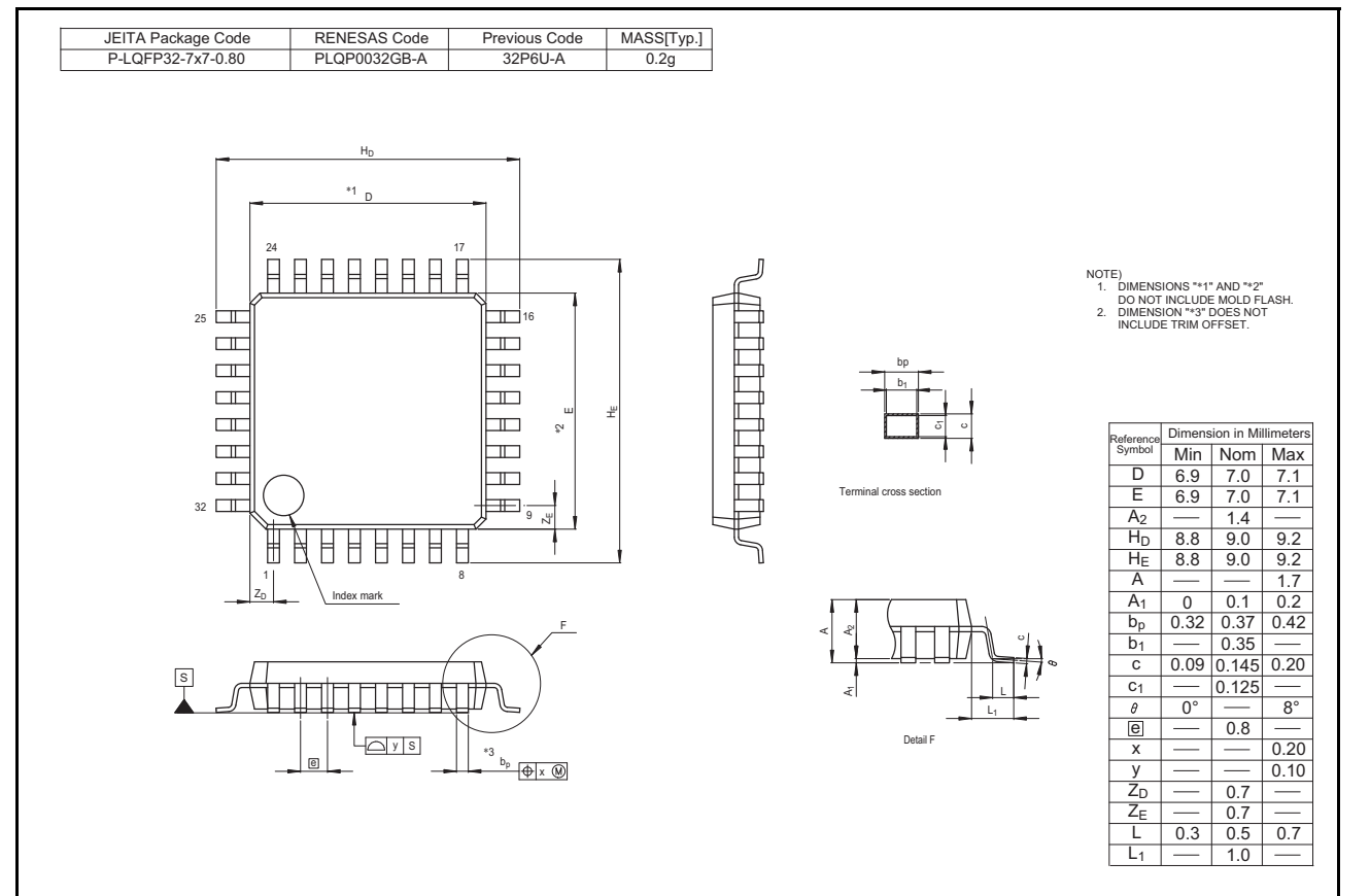
Figure 2.3 LQFP 32-pin
