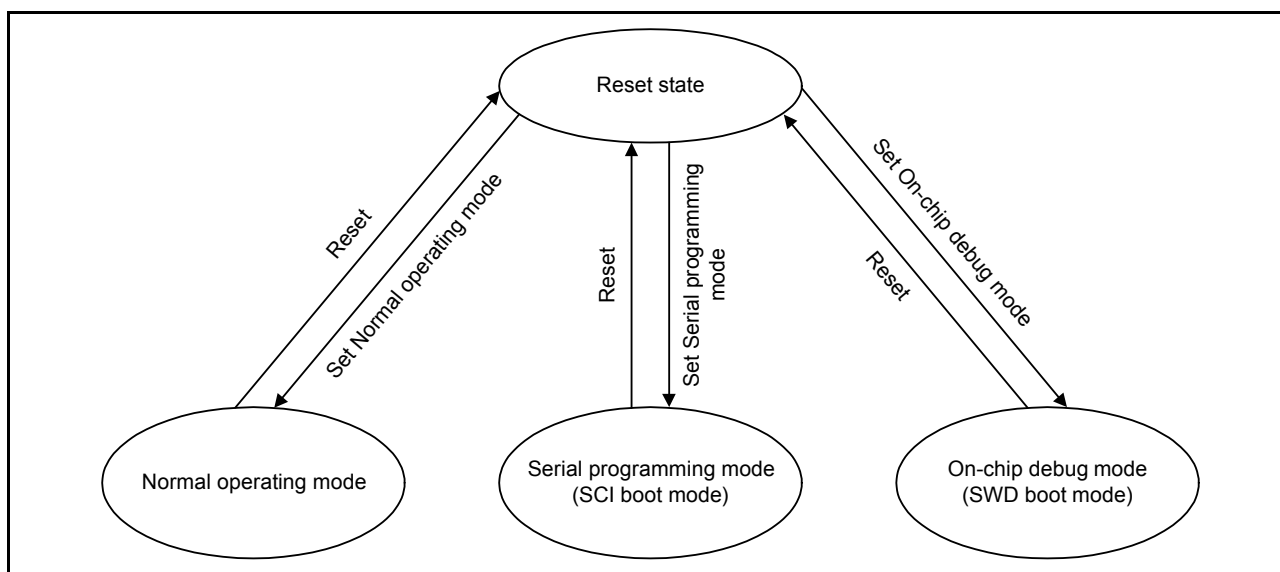
Figure 42.4 Mode transitions associated with the flash memory
