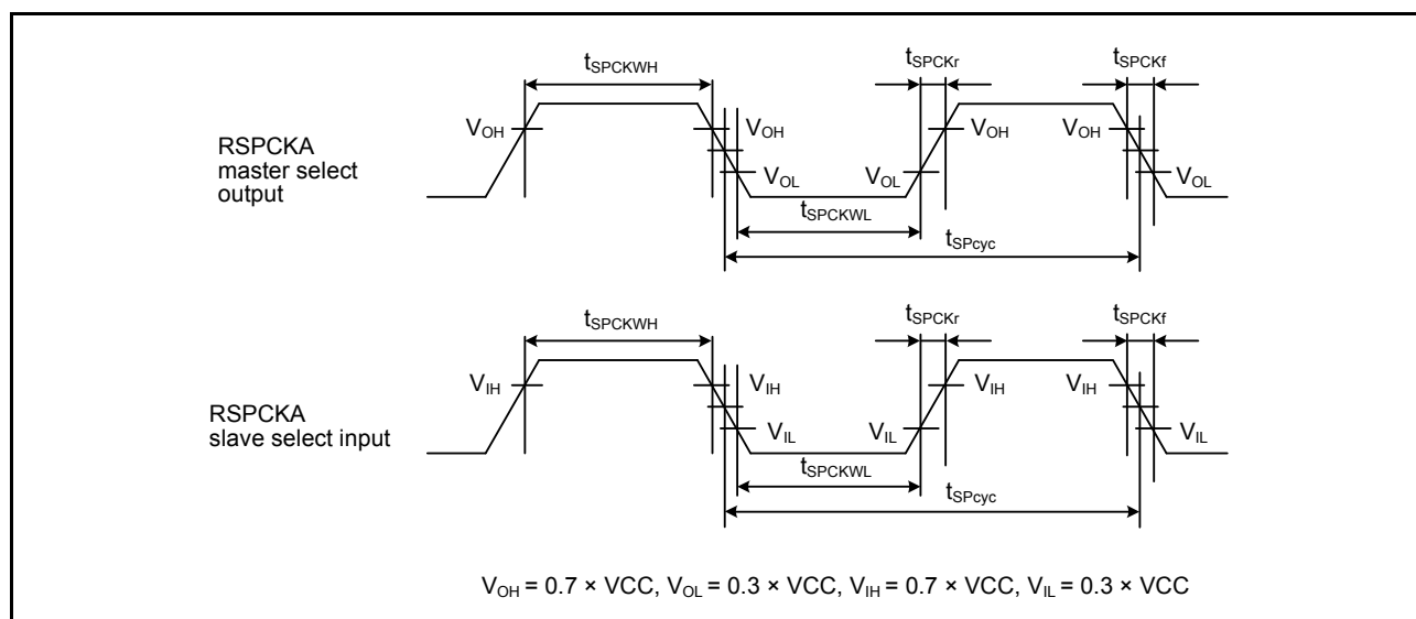
Figure 46.42 SPI clock timing
