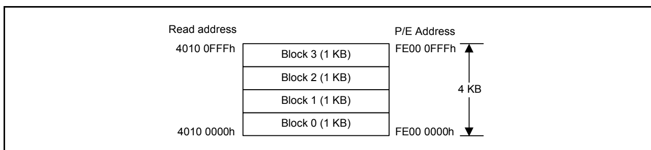
Figure 42.3 Mapping of data flash memory
