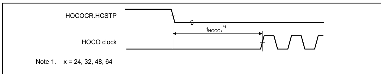
Figure 46.20 HOCO clock oscillation start timing (started by setting the HOCOCCR.HCSTP bit)
