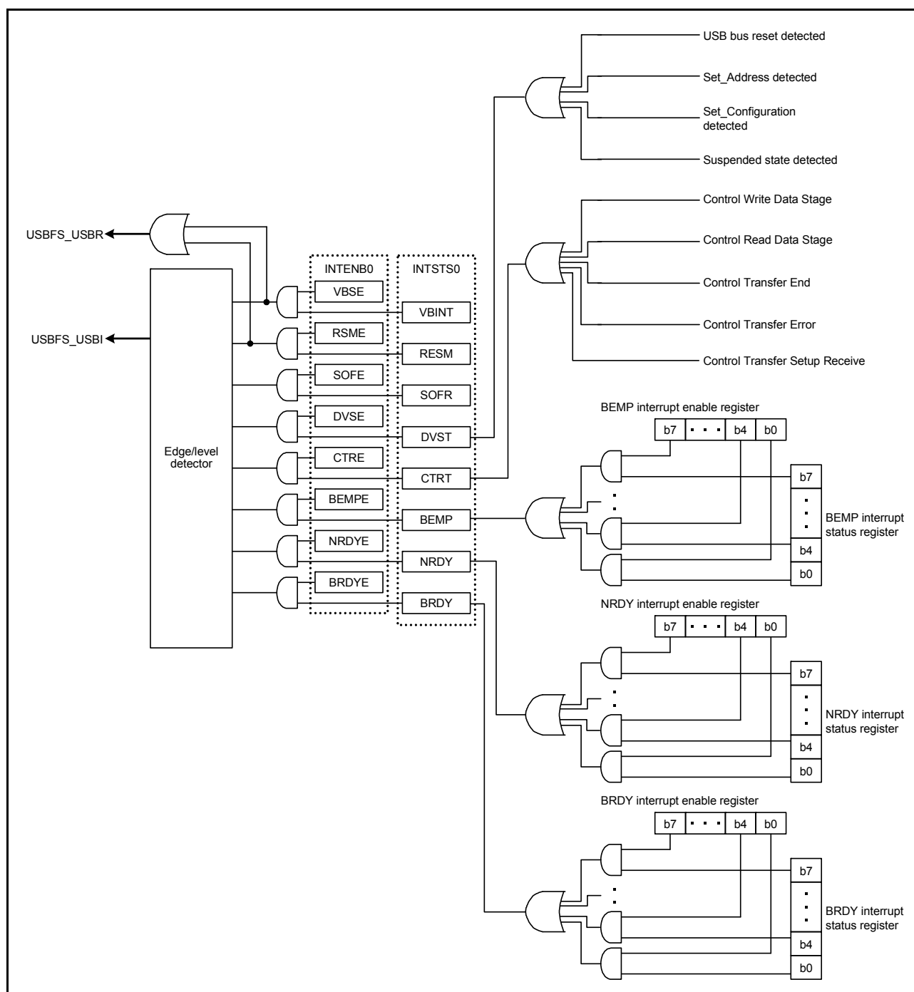
Figure 26.8 Circuits related to interrupts in USBFS
