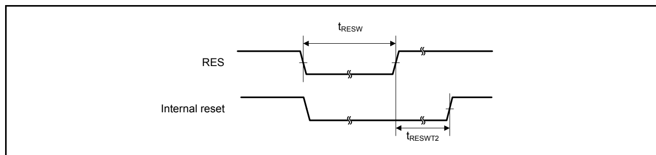
Figure 46.23 Reset input timing (1)
