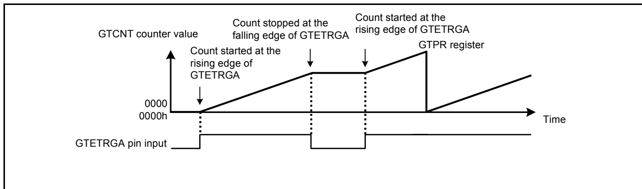
Figure 20.51 Example of count start/stop operation by hardware source started at rising edge of GTETRG pin input, and stopped at falling edge of GTETRG pin input
