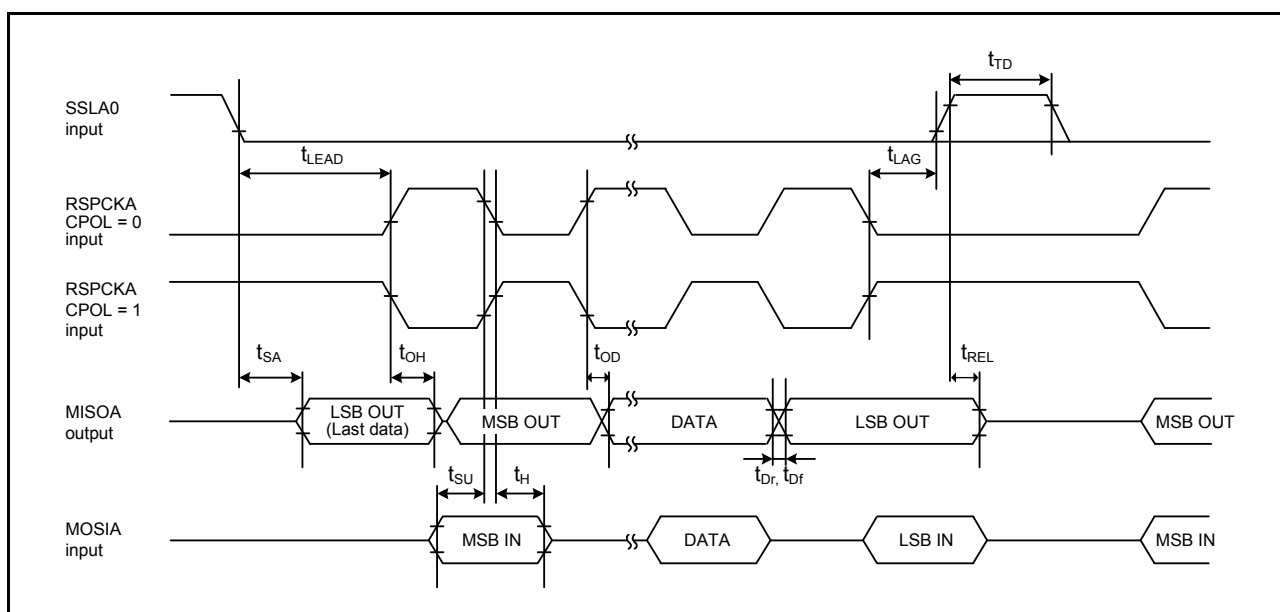
Figure 46.48 SPI timing (slave, CPHA = 1)
