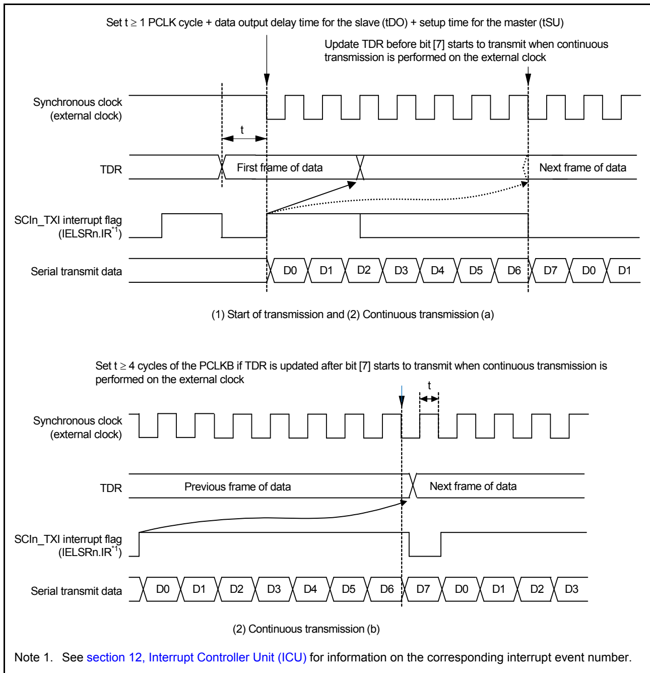
Figure 27.77 Restrictions on the use of external clock in clock synchronous transmission
