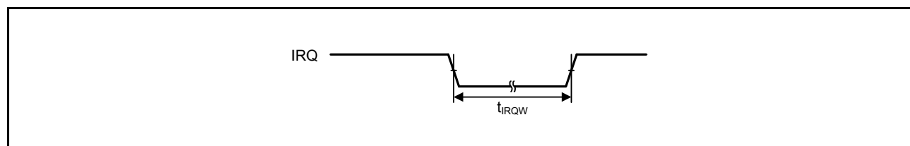
Figure 46.27 IRQ interrupt input timing
