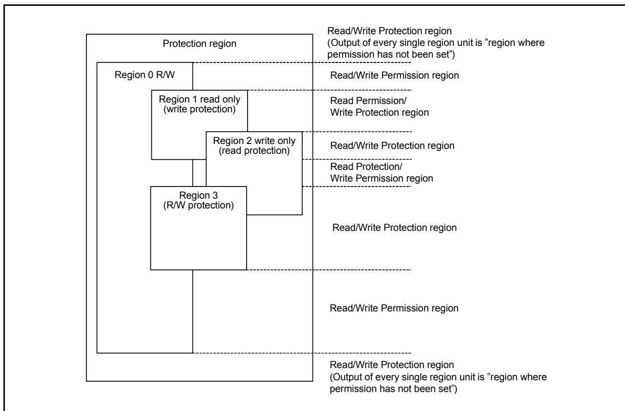
Figure 14.6 Access permission or protection by overlap of the Bus Master MPU region
