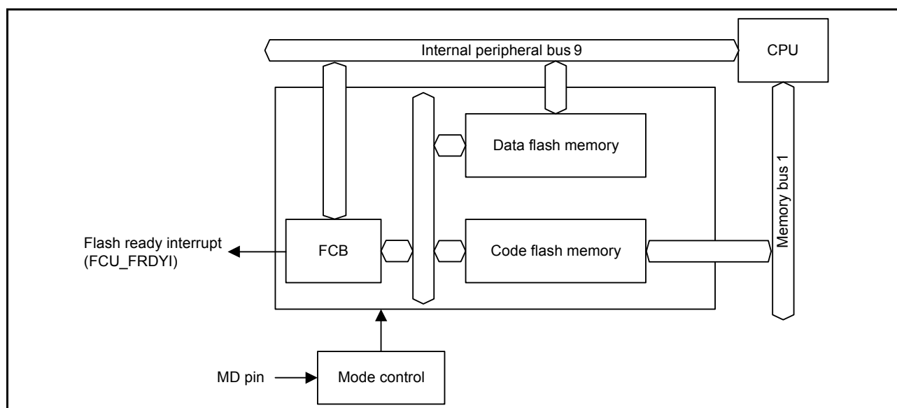
Figure 42.1 Block diagram of flash memory-related modules
