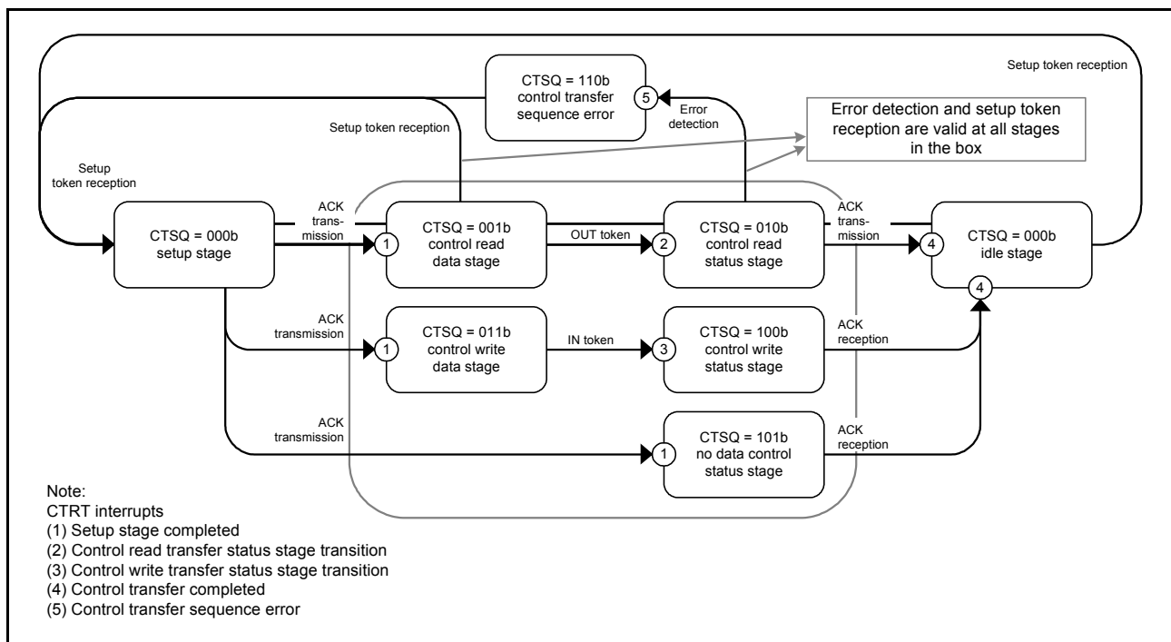
Figure 26.13 Control transfer stage transitions
