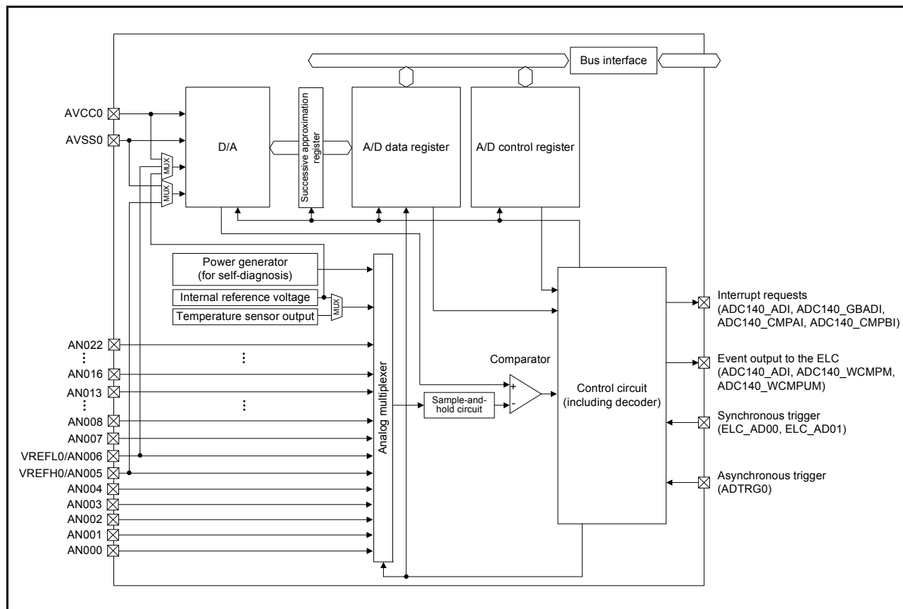
Figure 33.1 ADC14 block diagram
