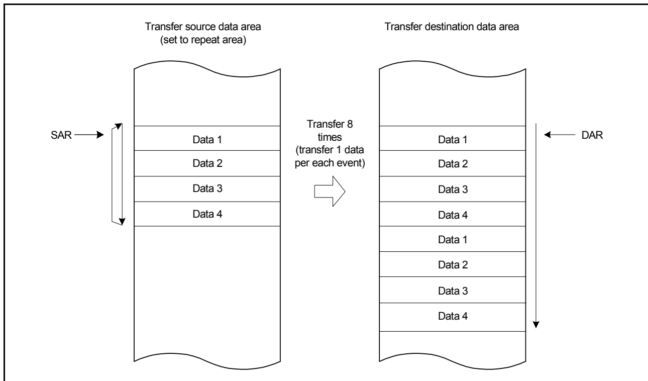
Figure 15.6 Memory map of repeat transfer mode when the transfer source is a repeat area (MRA.SM[1:0] = 10b, MRB.DM[1:0] = 10b, CRAH=04h)
