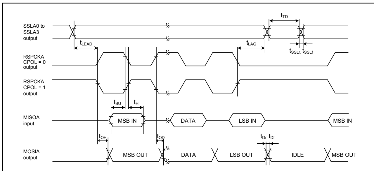
Figure 46.45 SPI timing (master, CPHA = 1) (bit rate: PCLKB division ratio is set to any value other than 1/2)
