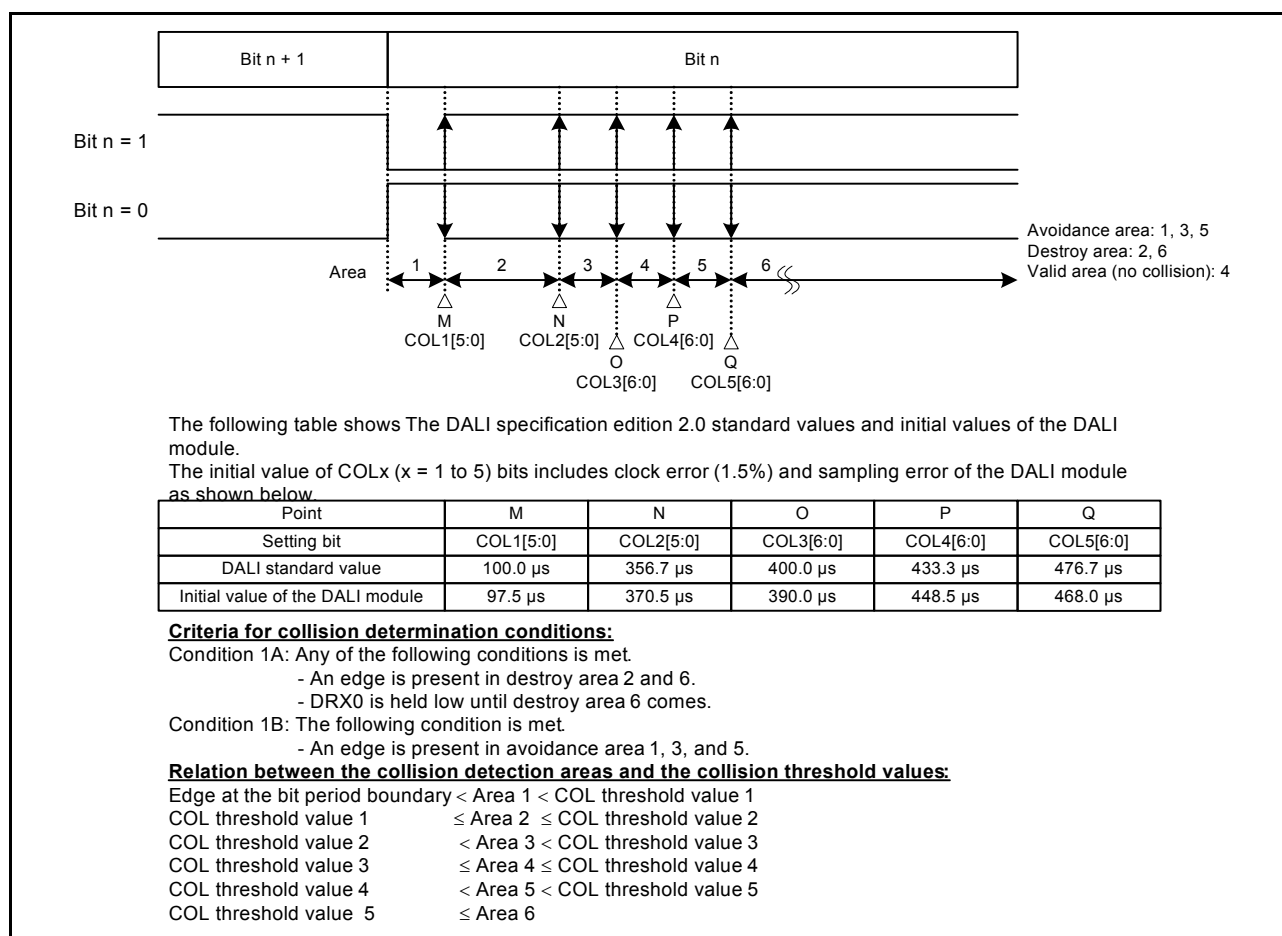
Figure 28.14 Collision detection timing 1
