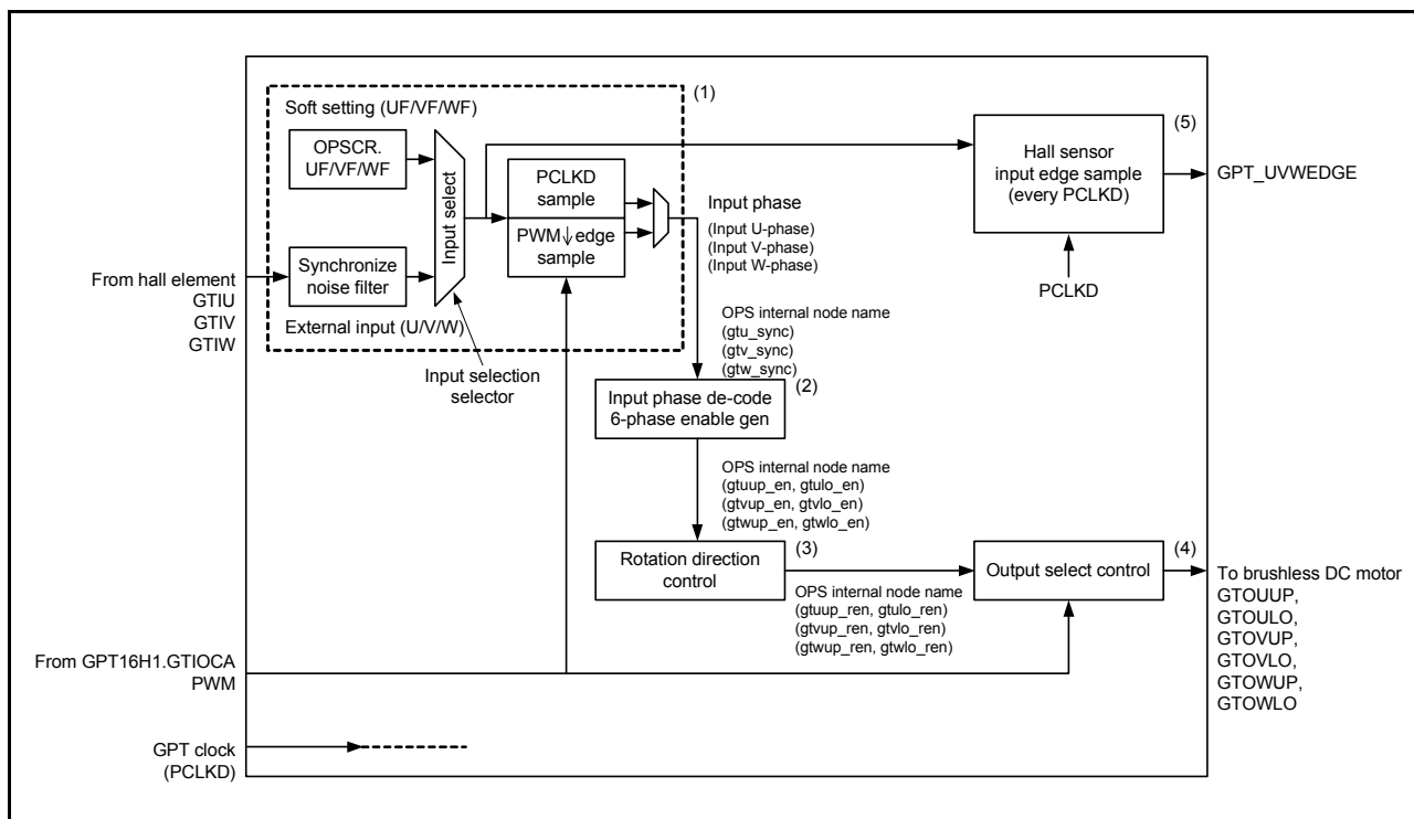
Figure 20.77 GPT_OPS control flow conceptual diagram
