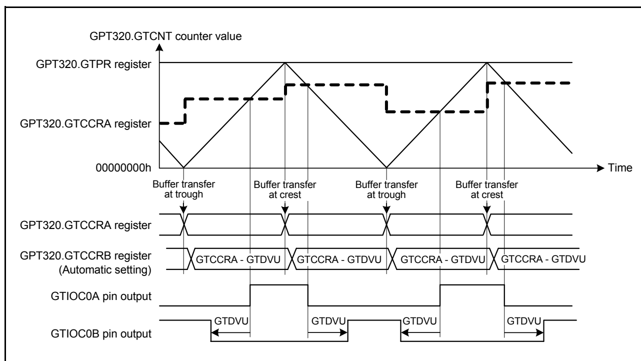
Figure 20.42 Example of automatic compare-match value setting function with dead time in triangle-wave PWM mode 2 or 3, and active-high
