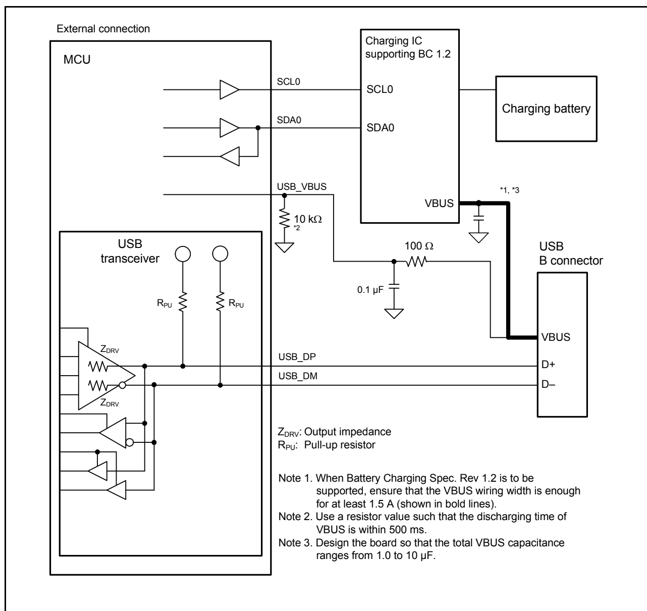
Figure 26.7 Functional connection sample of USB connector with Battery Charging Rev 1.2 supported
