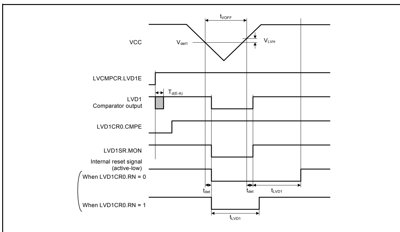
Figure 46.60 Voltage detection circuit timing ( V_{det1} )
