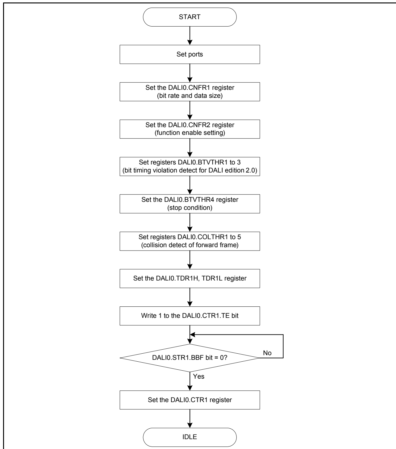
Figure 28.20 Initial setting flow
