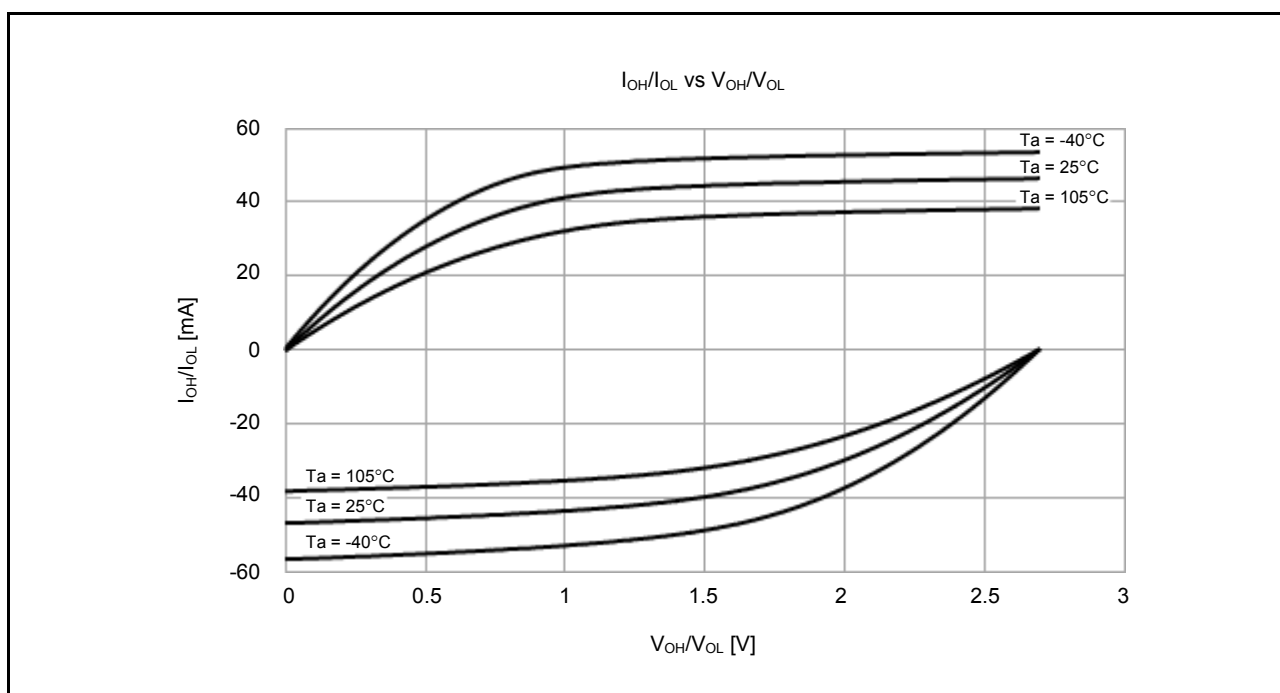
Figure 46.13 V_{OH}/V_{OL} and I_{OH}/I_{OL} temperature characteristics at V_{CC} = 2.7 V when low drive output is selected (reference data)
