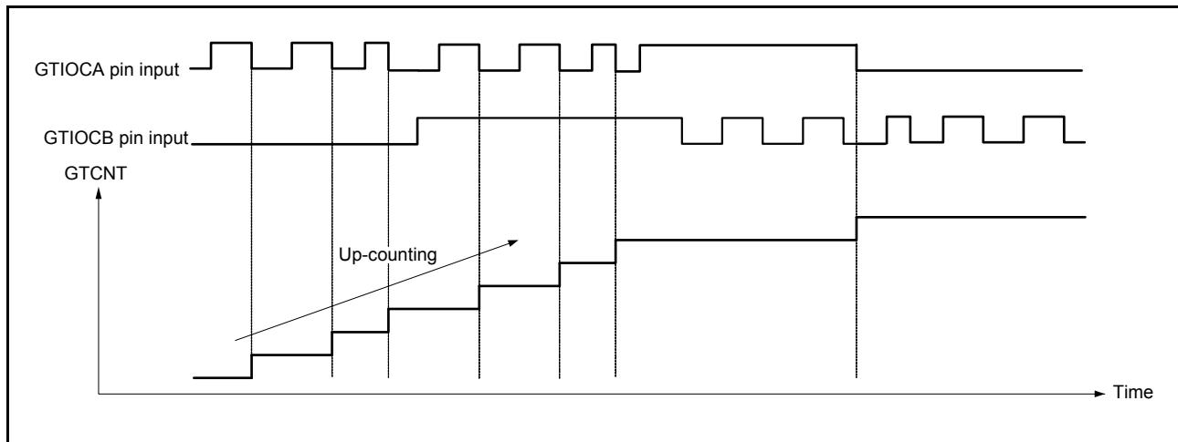
Figure 20.75 Example of phase counting mode 5 (A)
