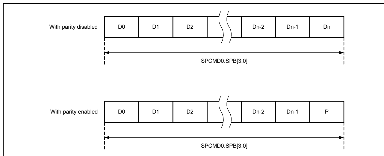
Figure 31.13 Data format with parity disabled and enabled
