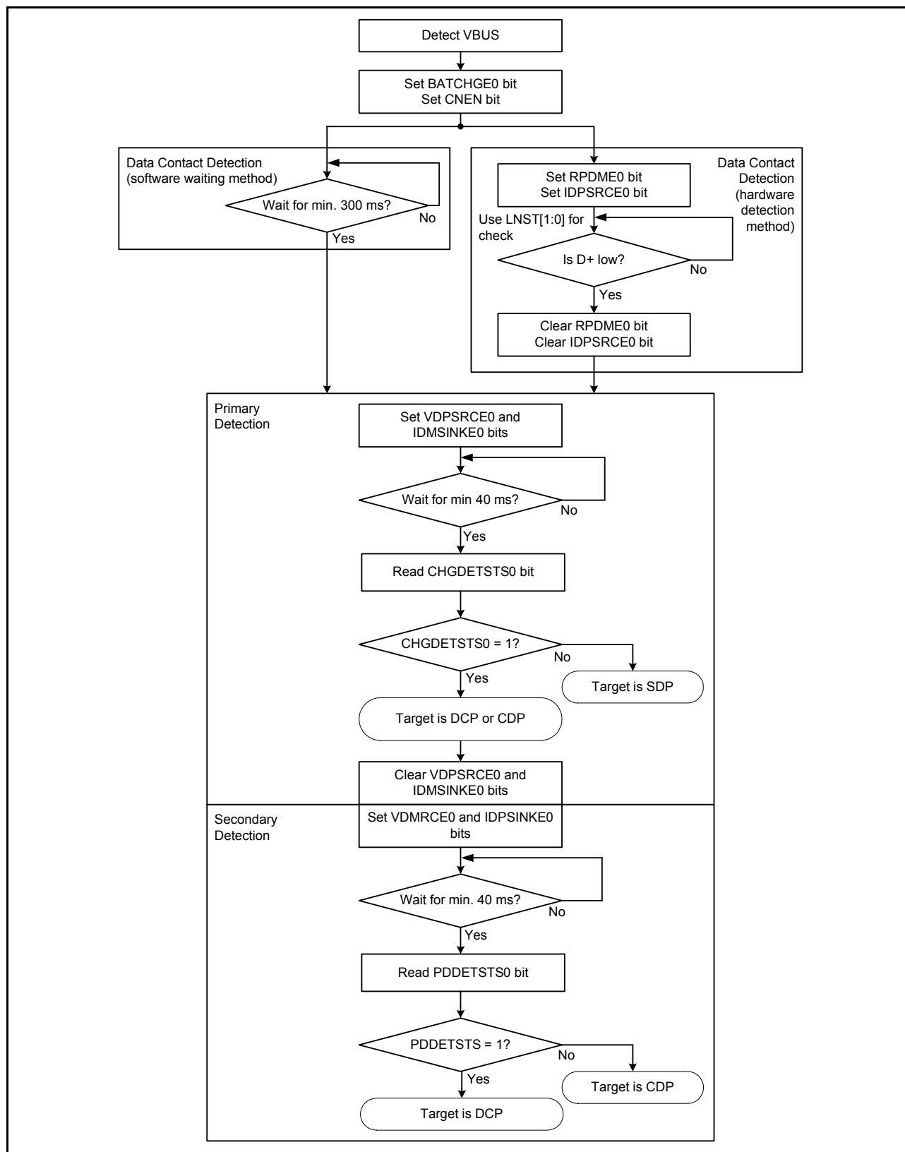
Figure 26.14 Process flow for operating as portable device
