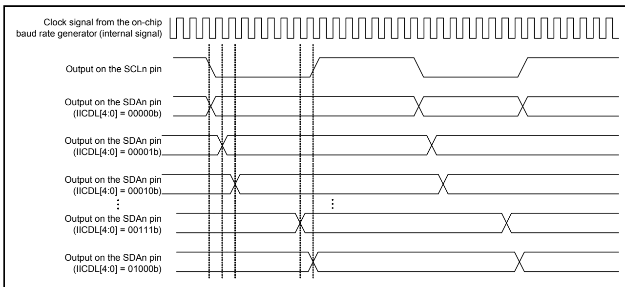
Figure 27.61 Timing of delays in SDAn output
