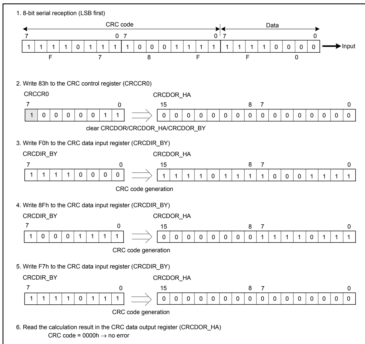
Figure 32.4 LSB-first data reception
