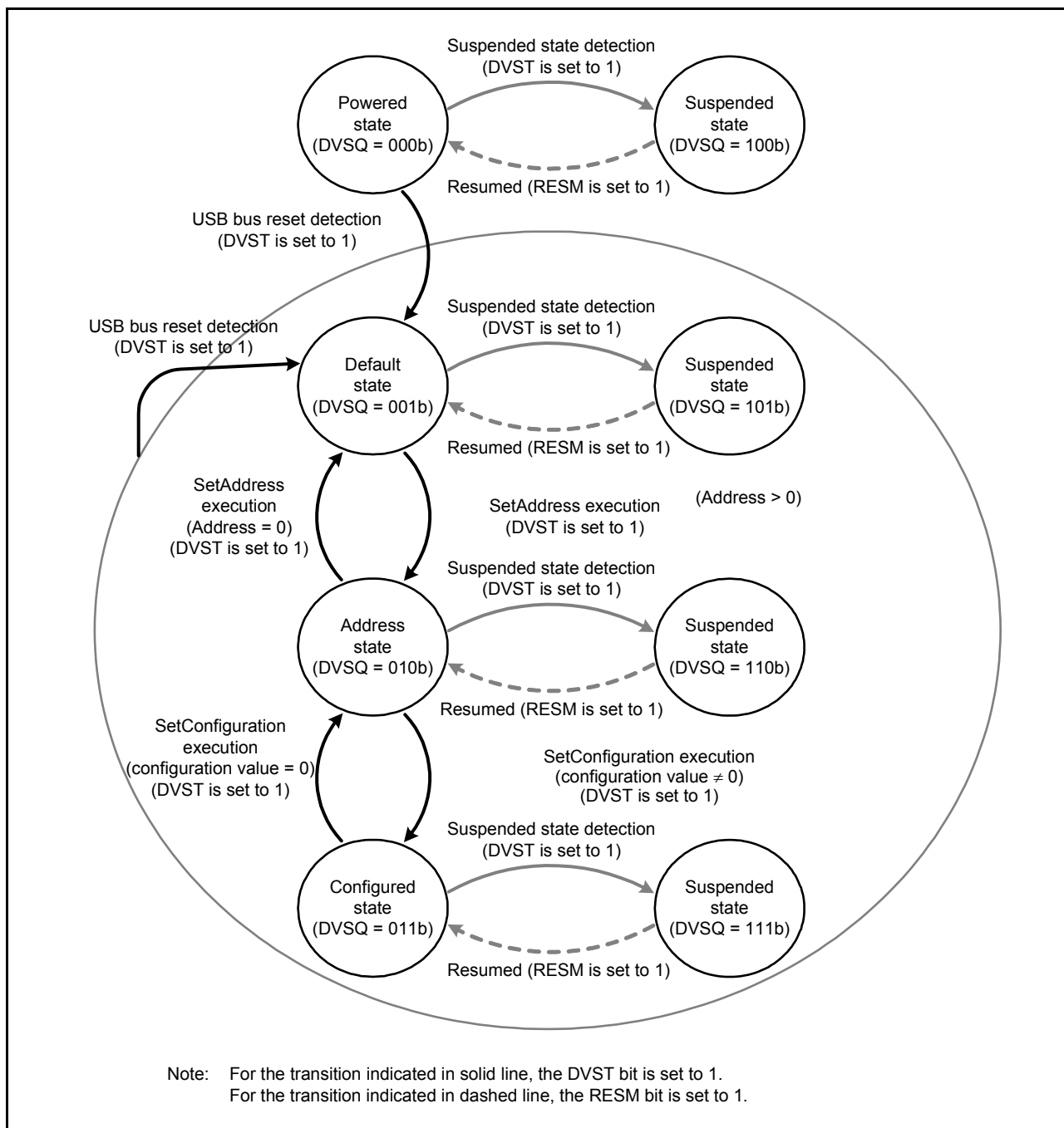
Figure 26.12 Device state transitions
