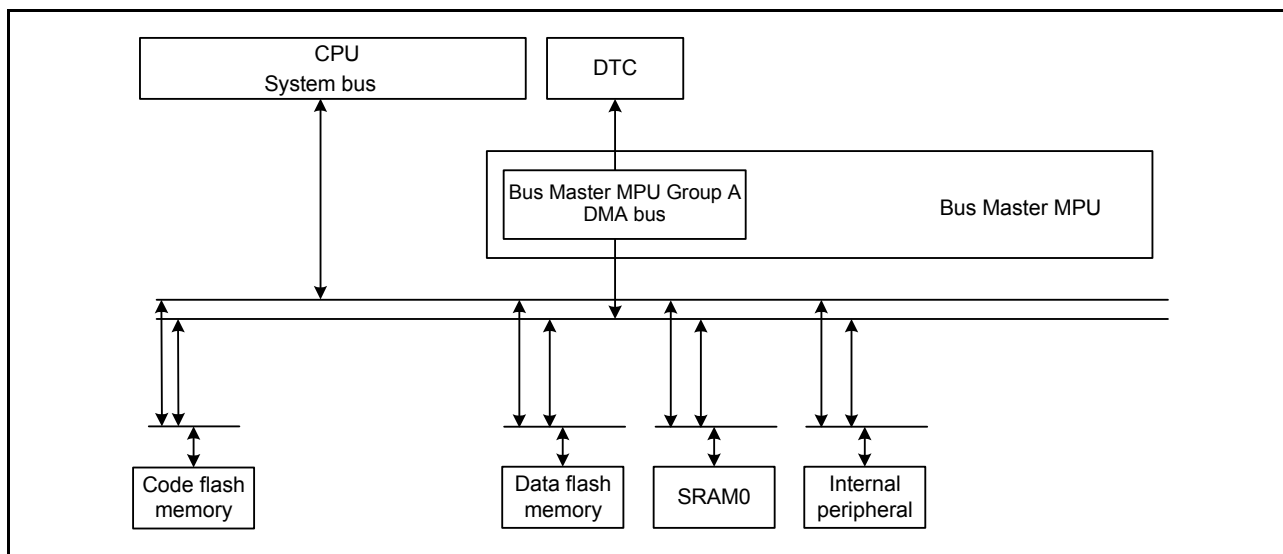
Figure 14.3 MPU bus master diagram
