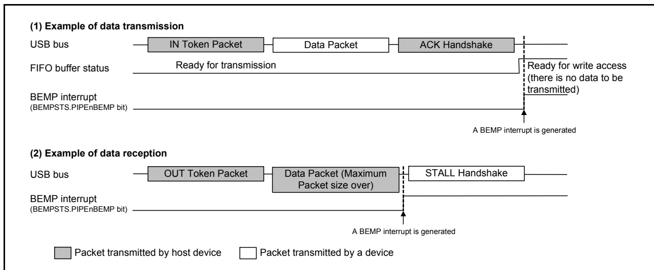
Figure 26.11 Timing of BEMP interrupt generation
