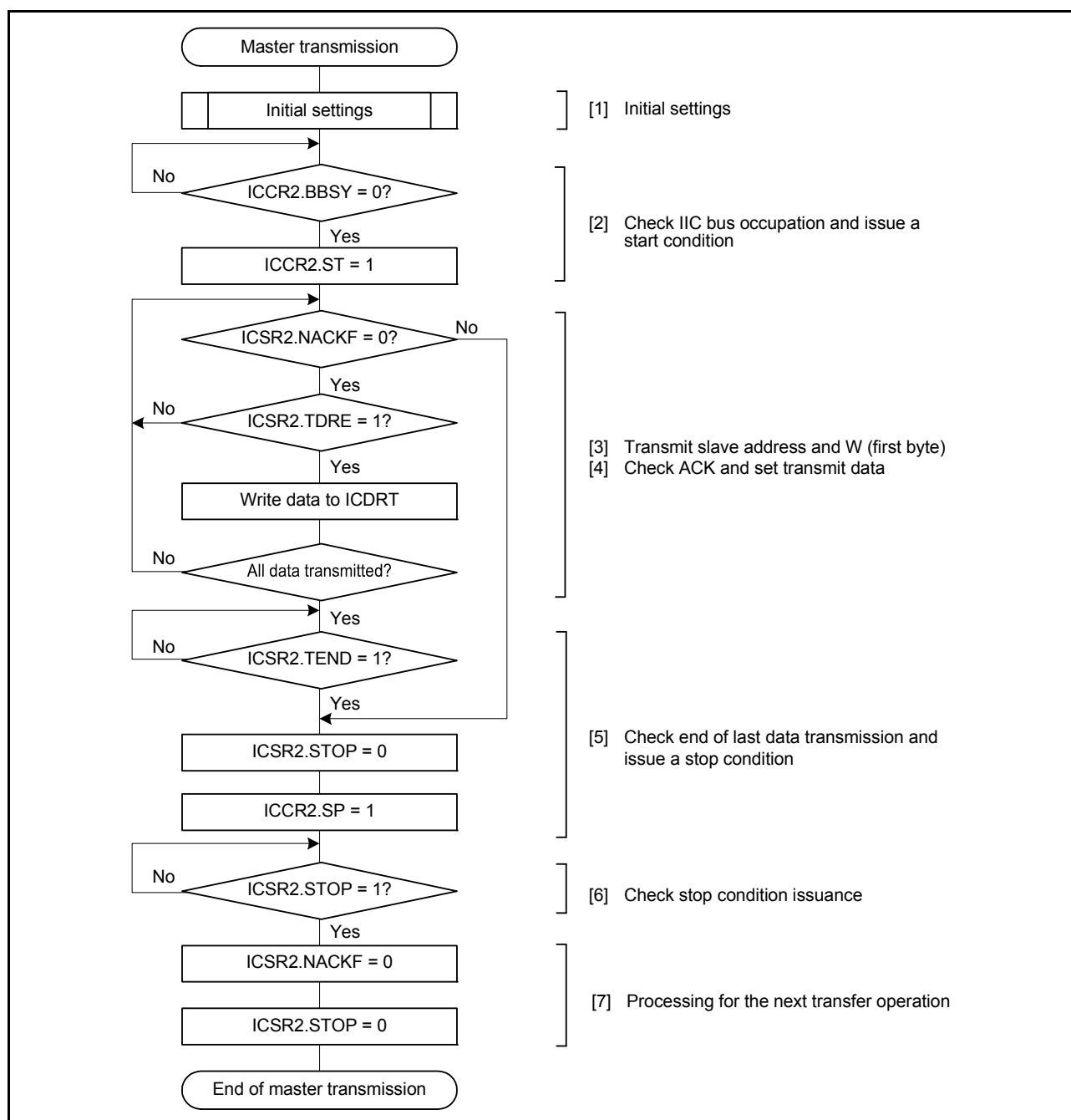
Figure 29.6 Example master transmission flow
