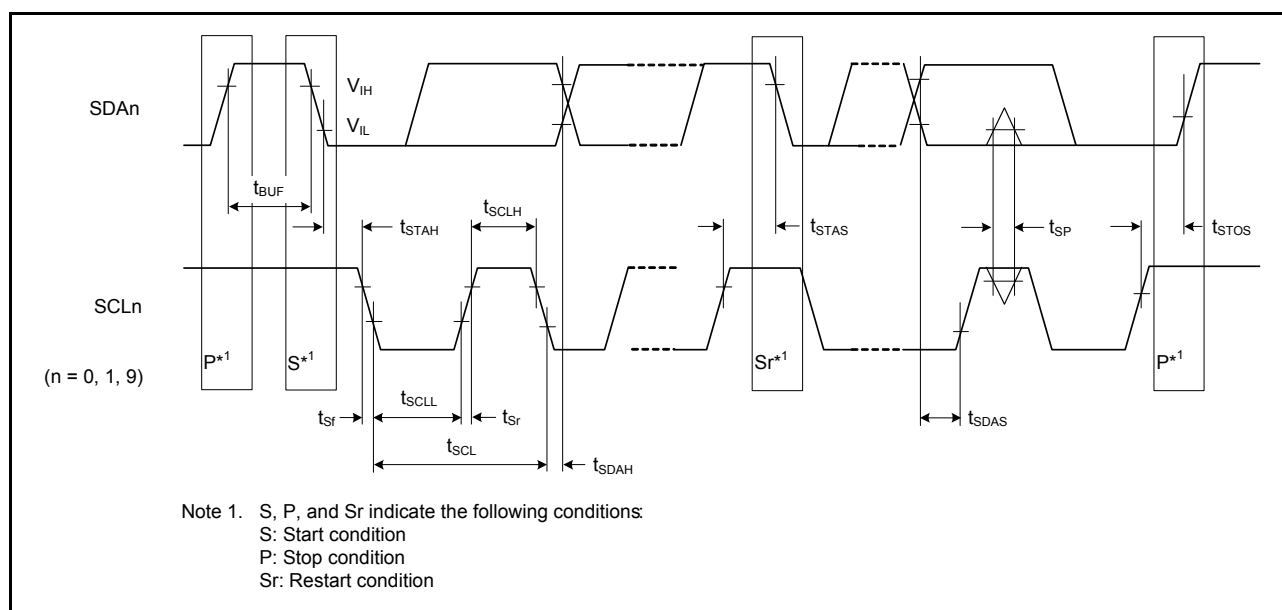
Figure 46.41 SCI simple IIC mode timing
