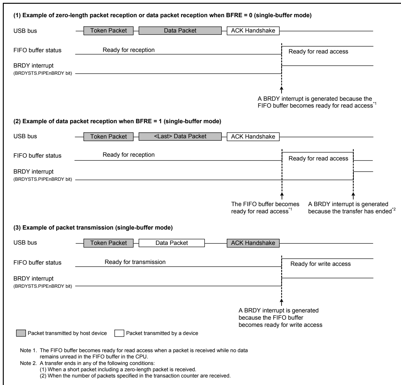
Figure 26.9 Timing of BRDY interrupt generation
