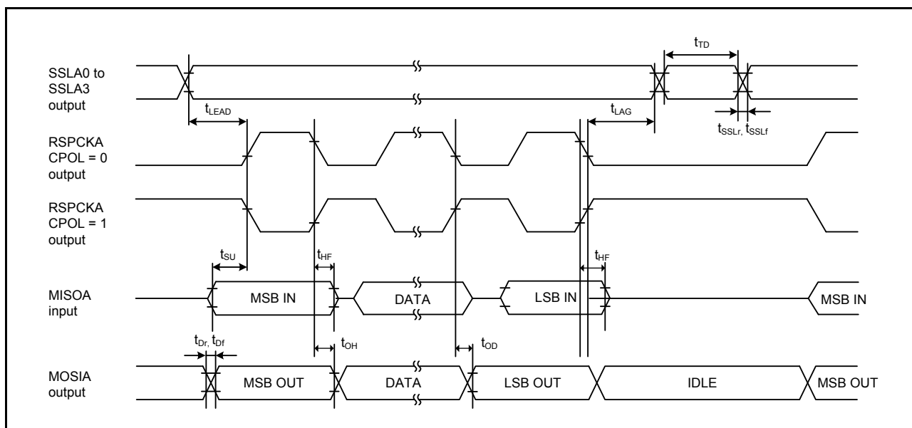
Figure 46.44 SPI timing (master, CPHA = 0) (bit rate: PCLKB division ratio is set to 1/2)
