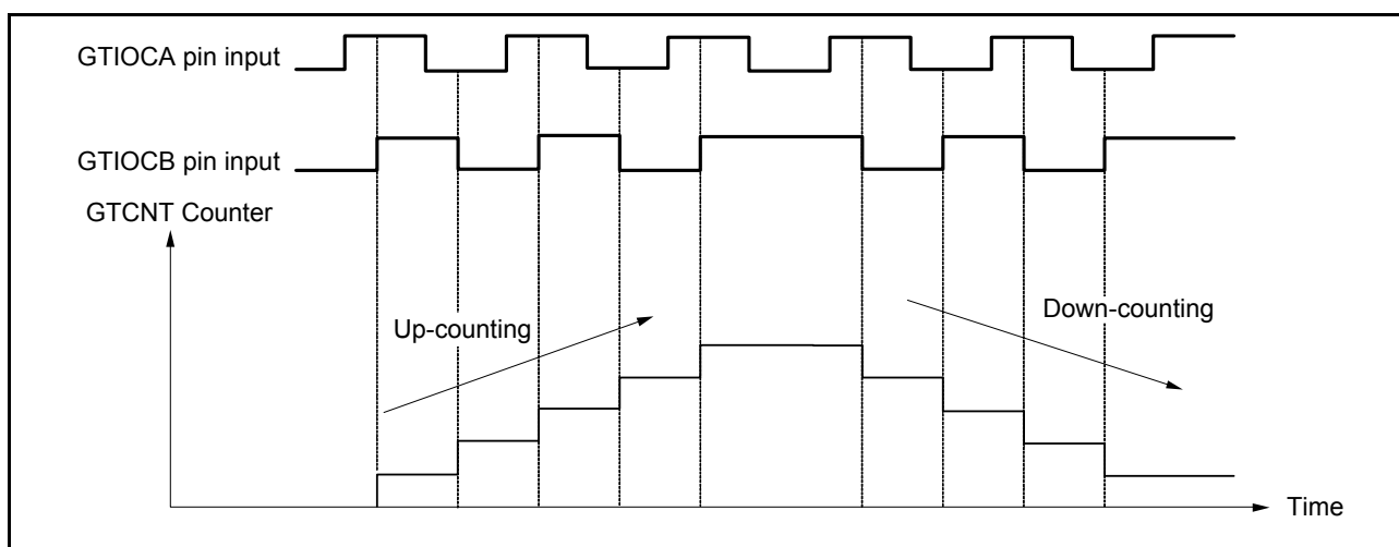
Figure 20.74 Example of phase counting mode 4
