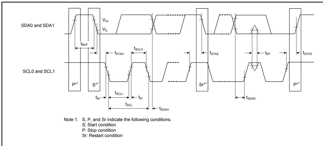
Figure 46.49 I2C bus interface input/output timing
