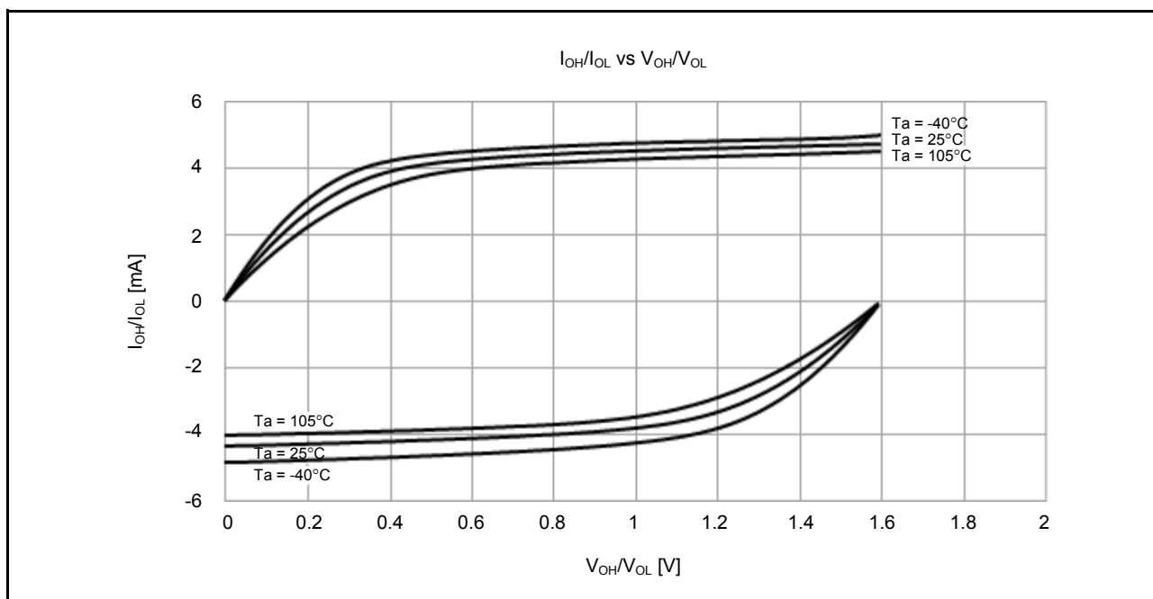
Figure 46.8 V_{OH}/V_{OL} and I_{OH}/I_{OL} temperature characteristics at V_{CC} = 1.6\text{ V} when middle drive output is selected (reference data, except for P914 and P915)
