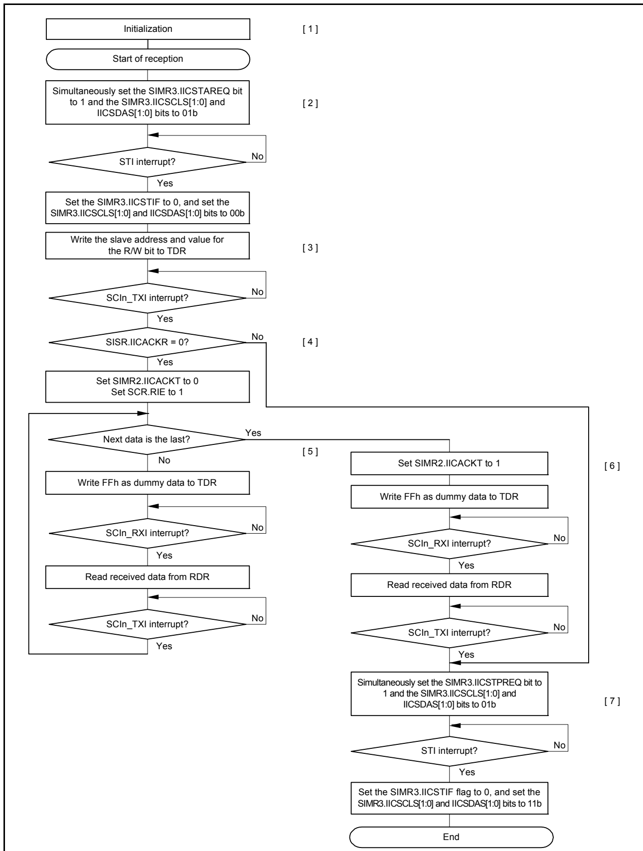
Figure 27.67 Example procedure for master reception operations in simple IIC mode with transmission interrupts and reception interrupts
