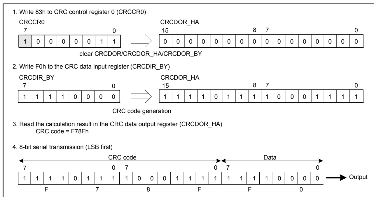
Figure 32.2 LSB-first data transmission
