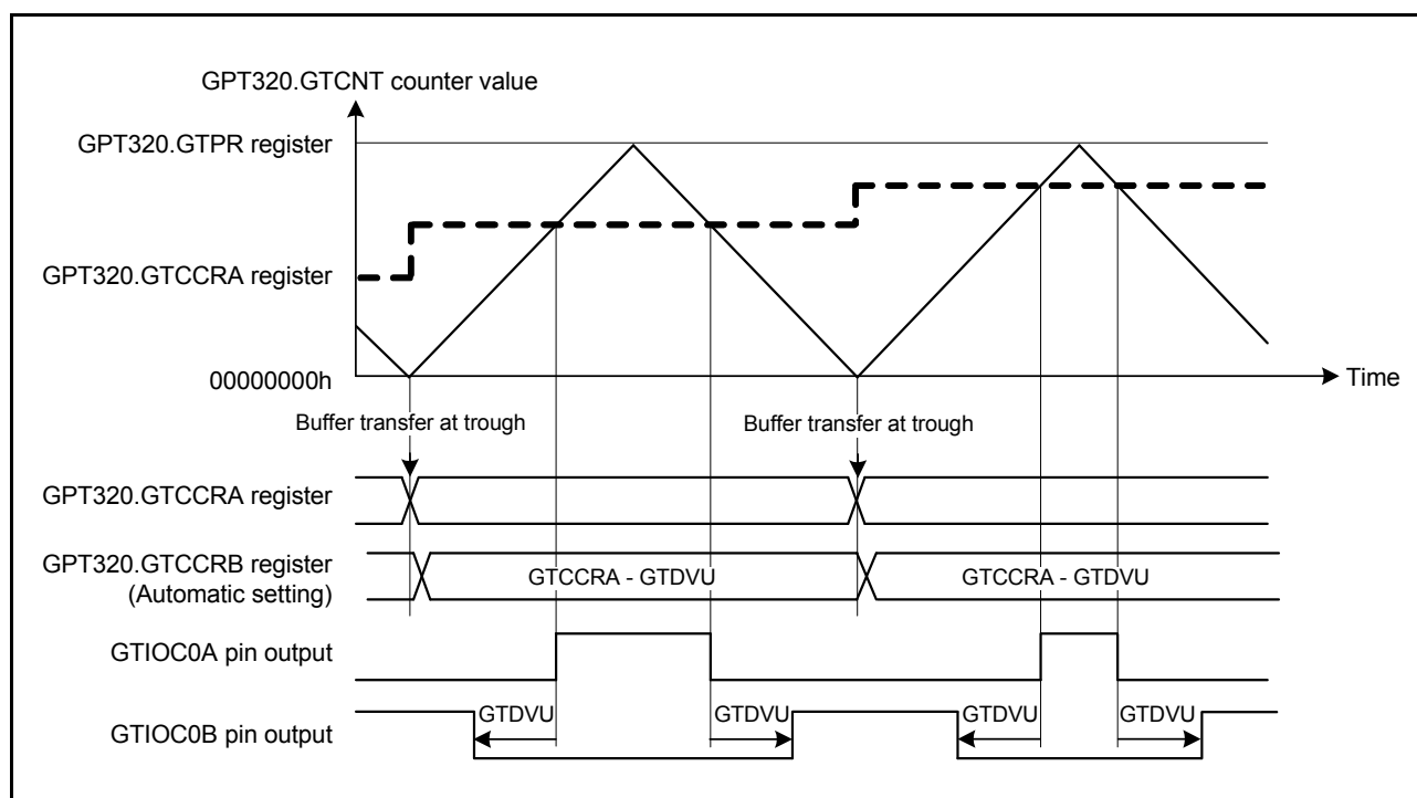
Figure 20.41 Example of automatic compare-match value setting function with dead time in triangle-wave PWM mode 1, and active-high
