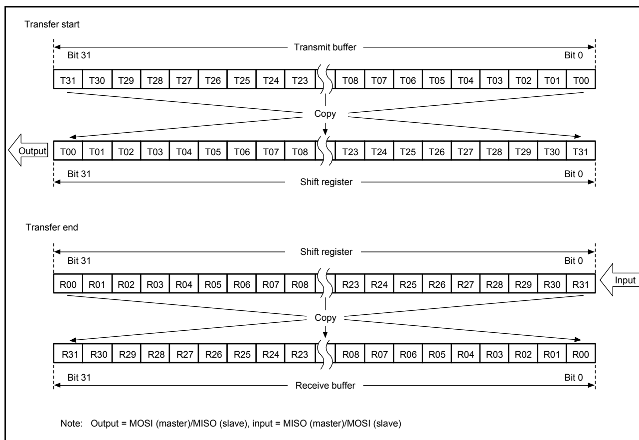
Figure 31.16 LSB-first transfer with 32-bit data and parity disabled
