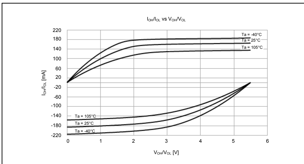
Figure 46.15 V_{OH}/V_{OL} and I_{OH}/I_{OL} temperature characteristics at V_{CC} = 5.5 V when low drive output is selected (reference data)
