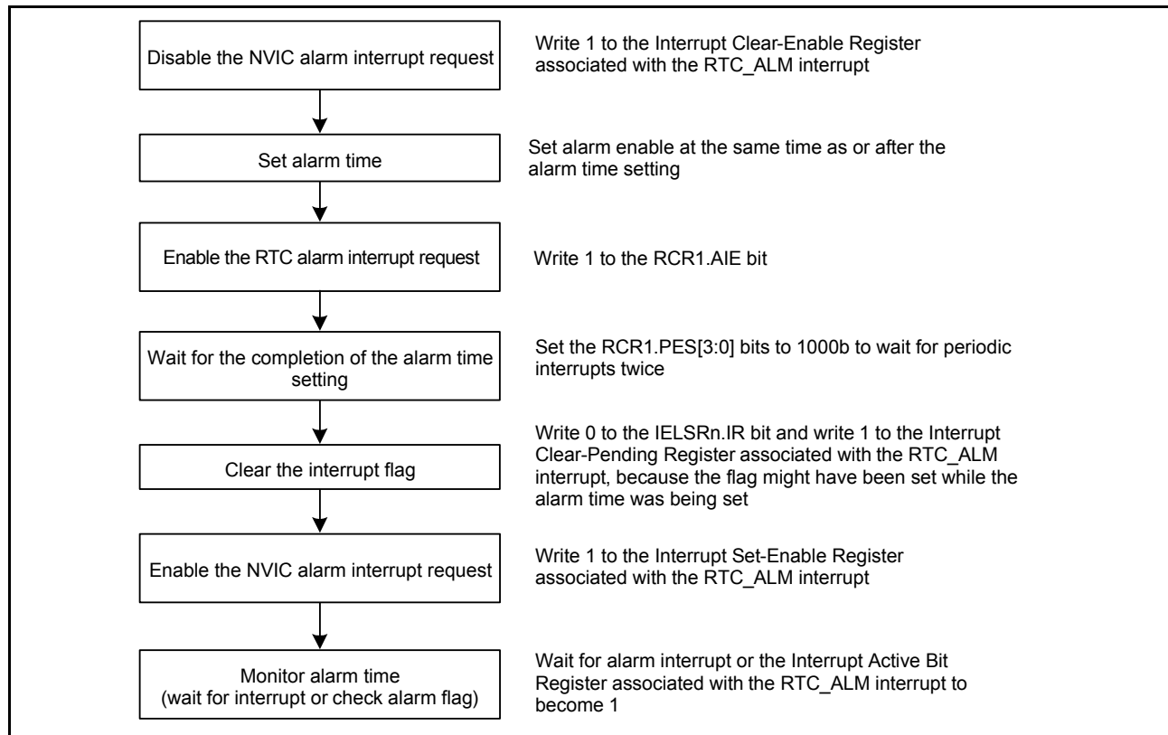
Figure 23.7 Using the alarm function
