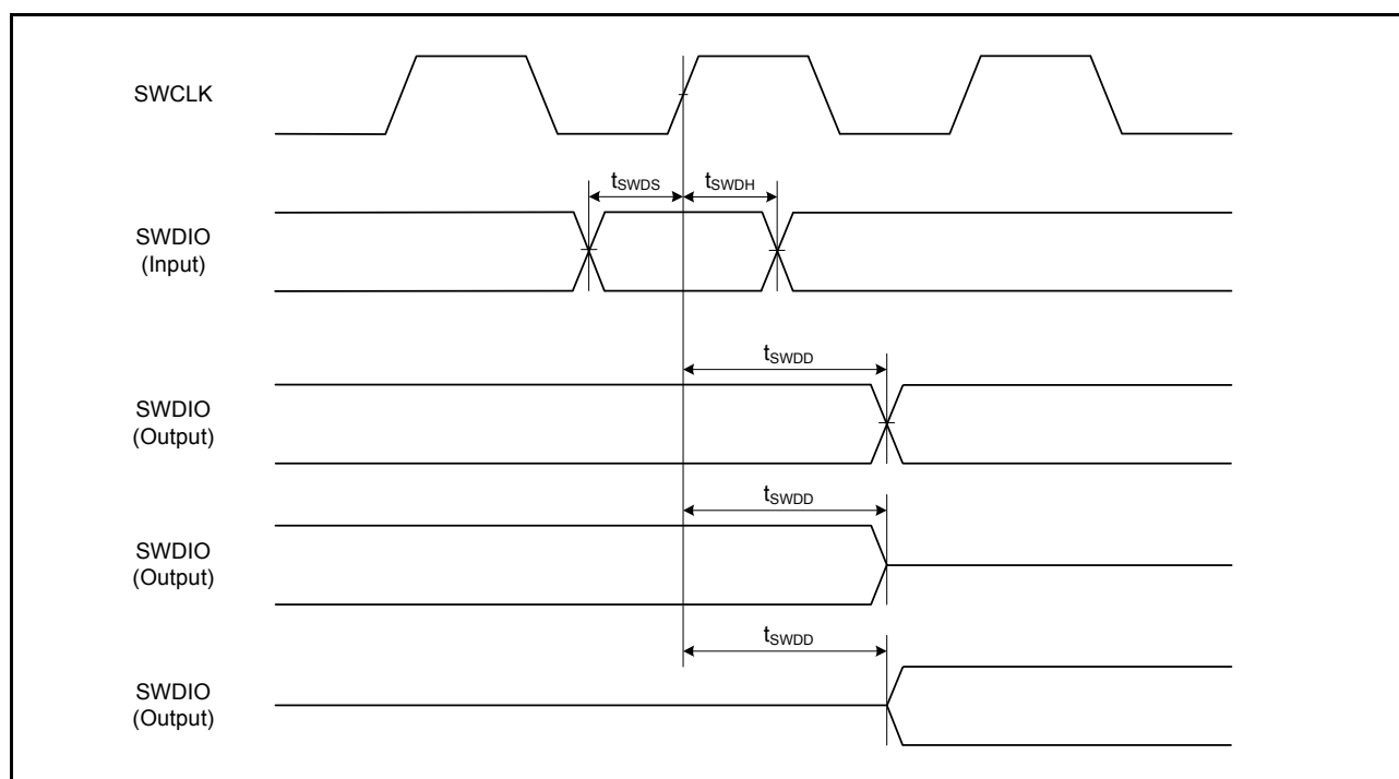
Figure 46.63 SWD input/output timing
