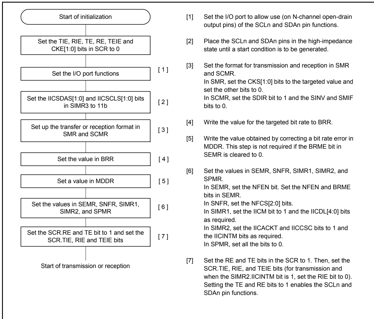
Figure 27.62 Example flow for SCI initialization in simple IIC mode
